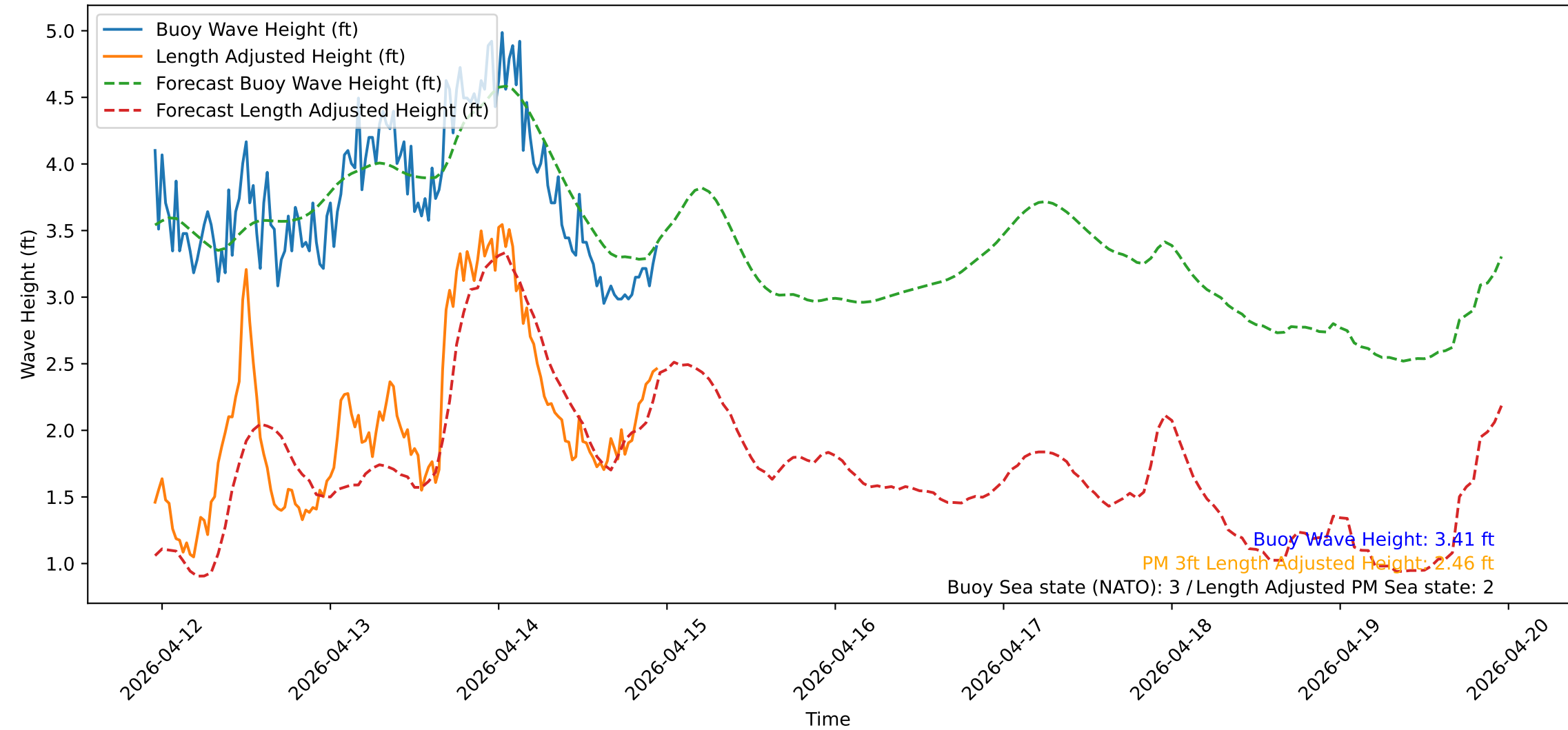
Wave Heights over Time for Green Beach at 2026-04-14 23:11:12
