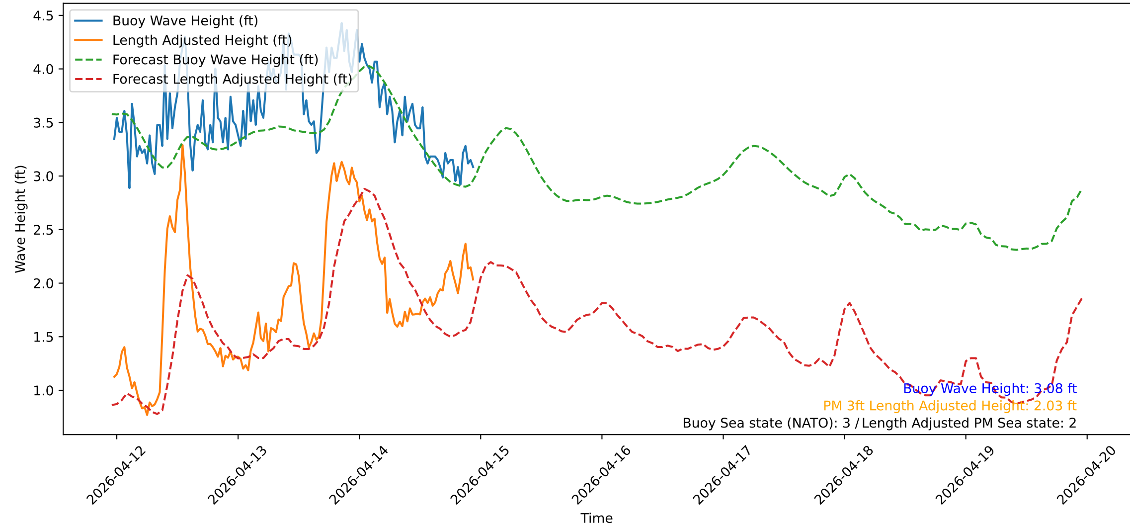
Wave Heights over Time for Red Beach at 2026-04-14 23:10:49
