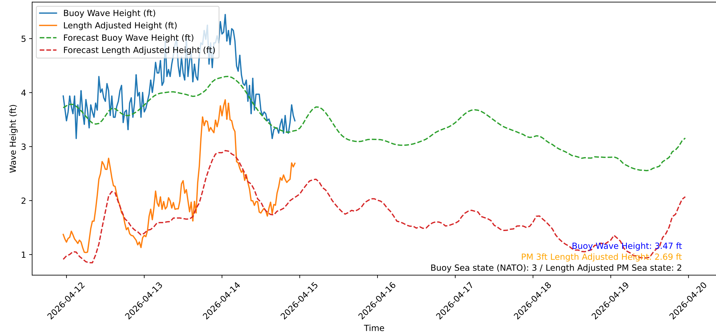
Wave Heights over Time for Oceanside Harbor at 2026-04-14 23:10:30
