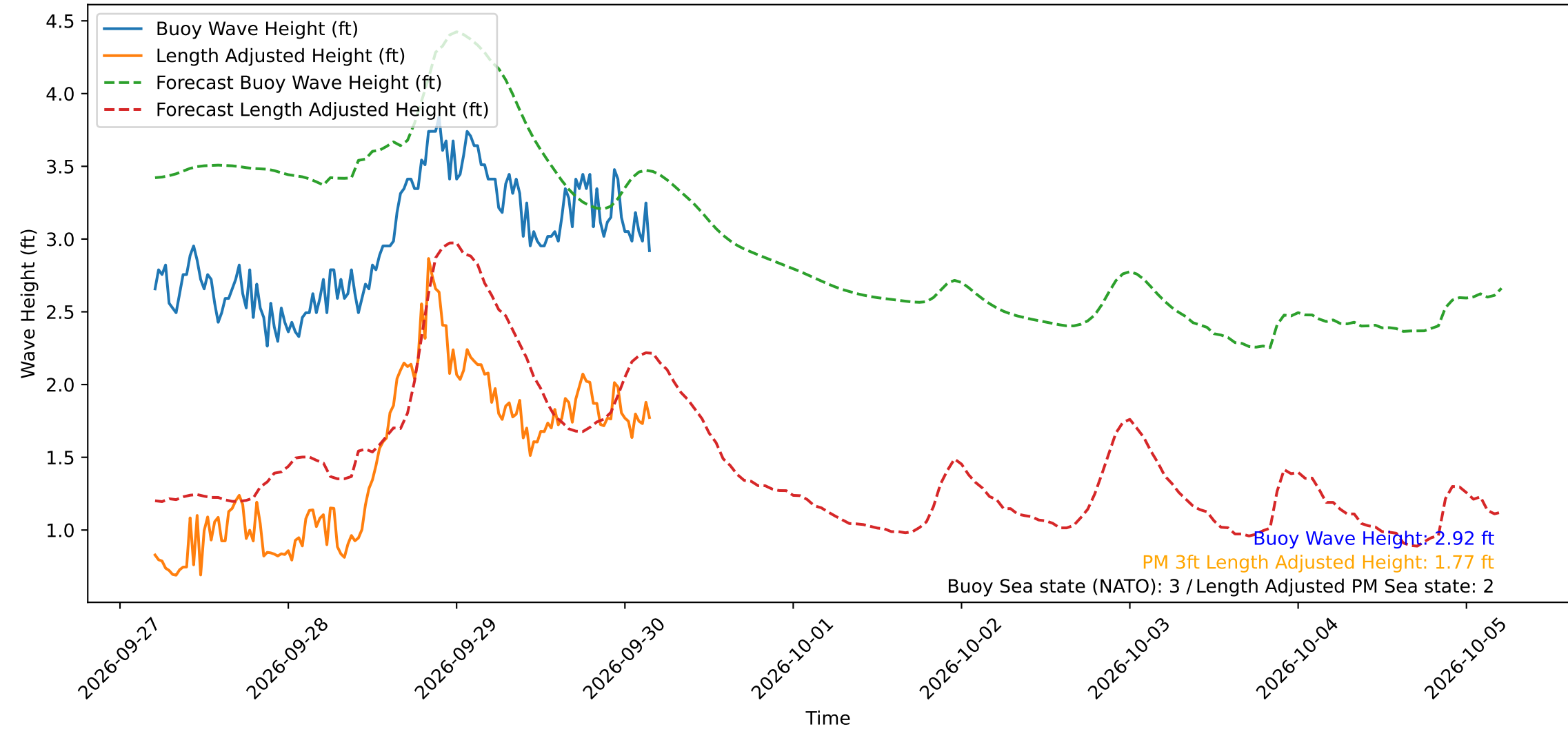
Wave Heights over Time for Red Beach at 2026-09-30 04:30:51
