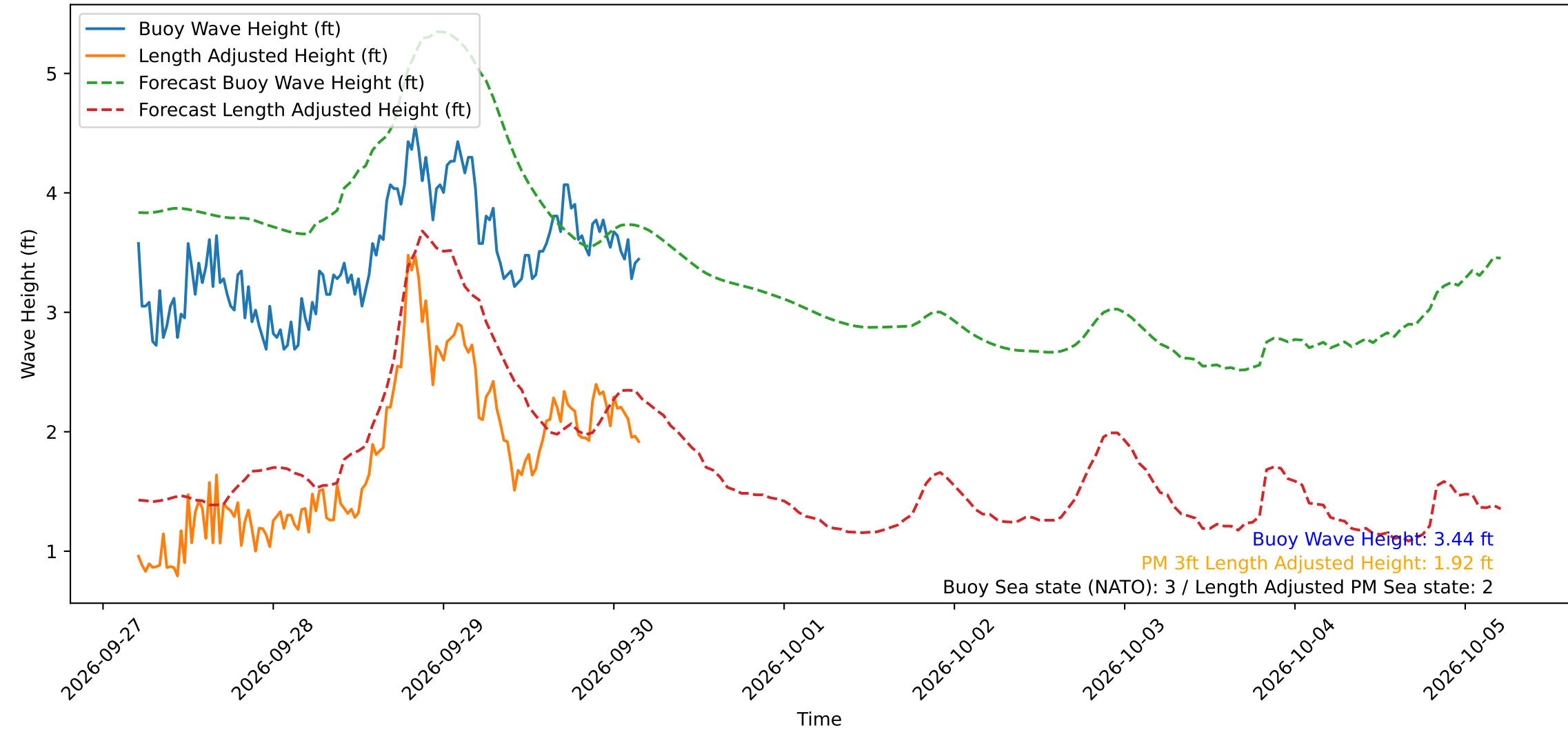
Wave Heights over Time for Green Beach at 2026-09-30 04:31:14
