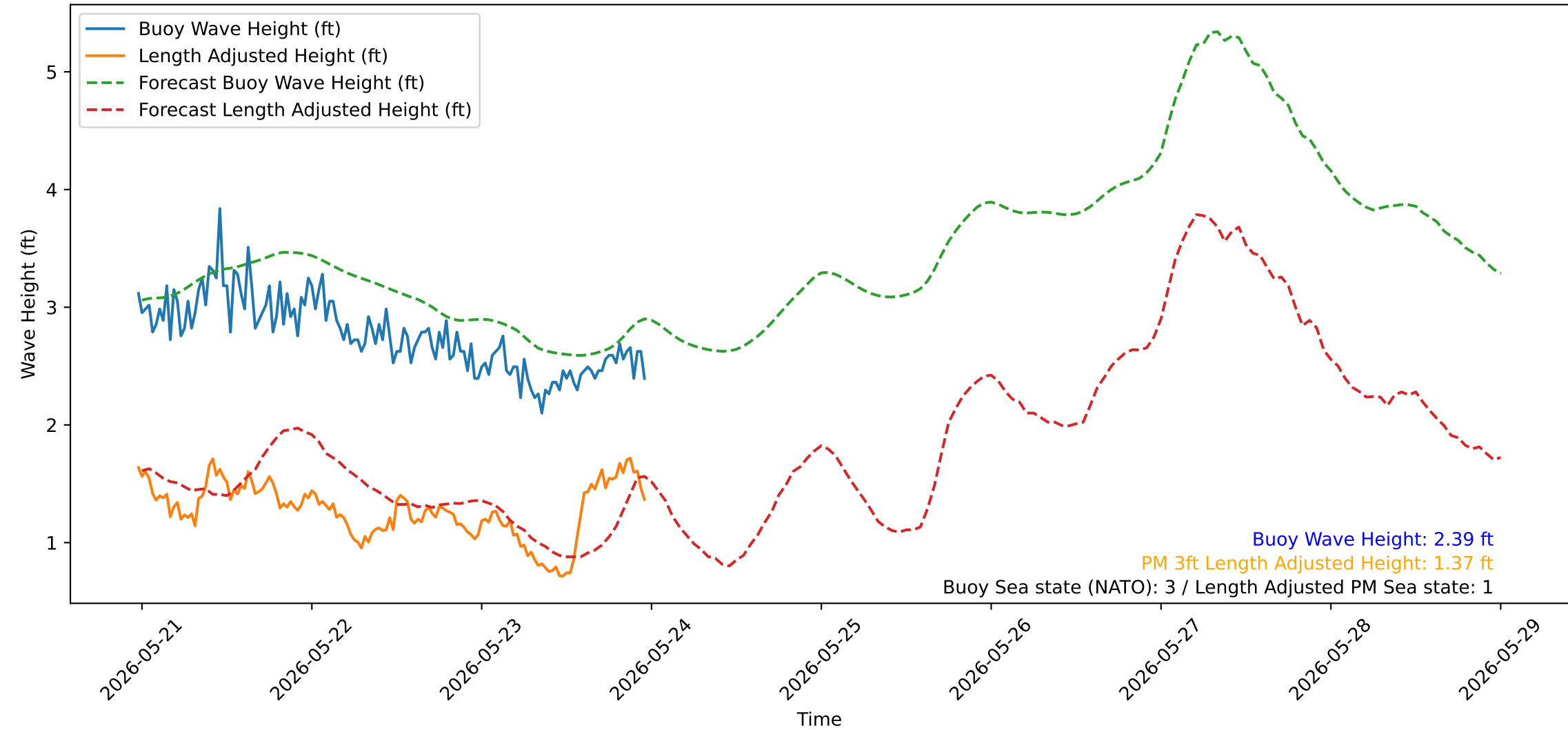
Wave Heights over Time for Oceanside Harbor at 2026-05-23 23:40:32
