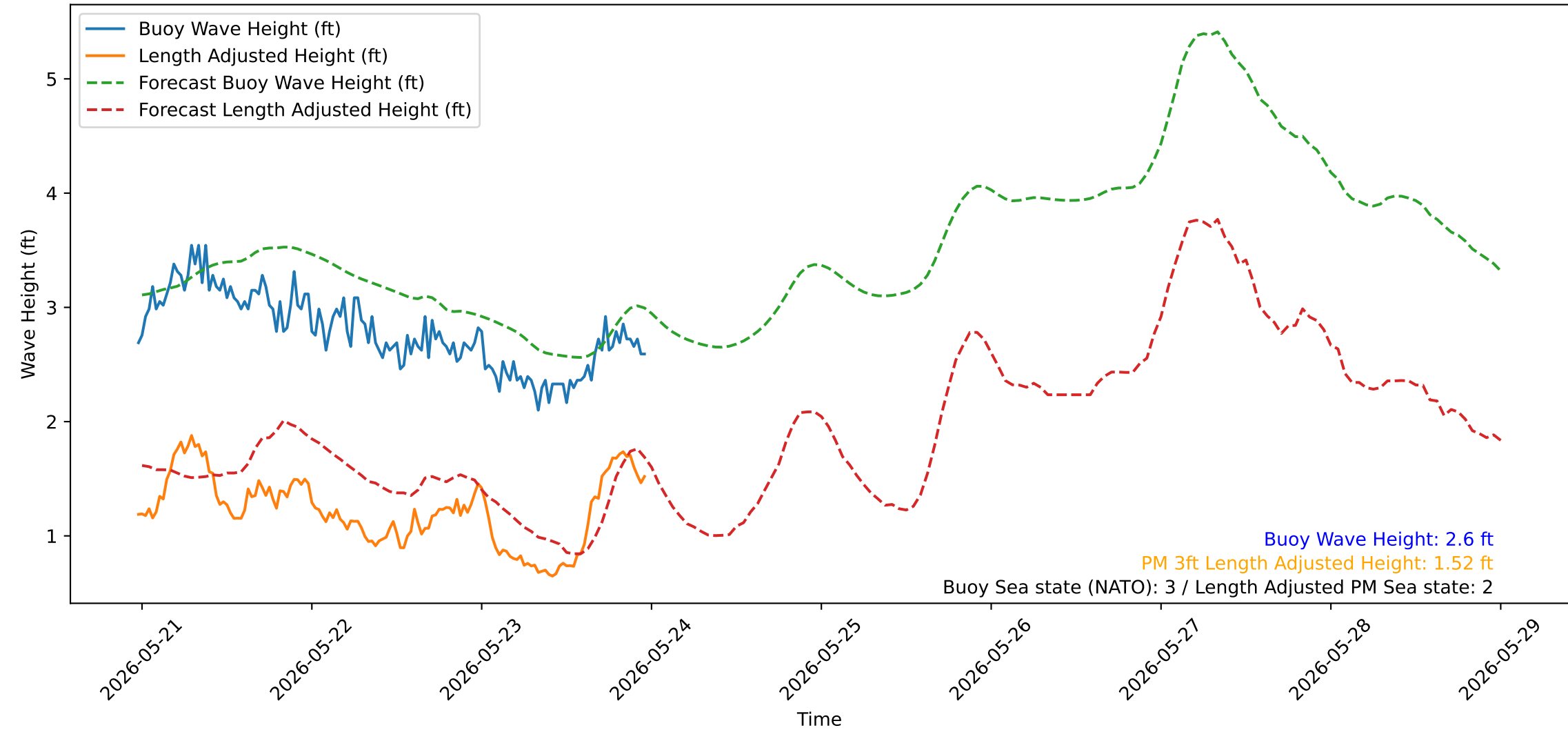
Wave Heights over Time for Green Beach at 2026-05-23 23:41:15
