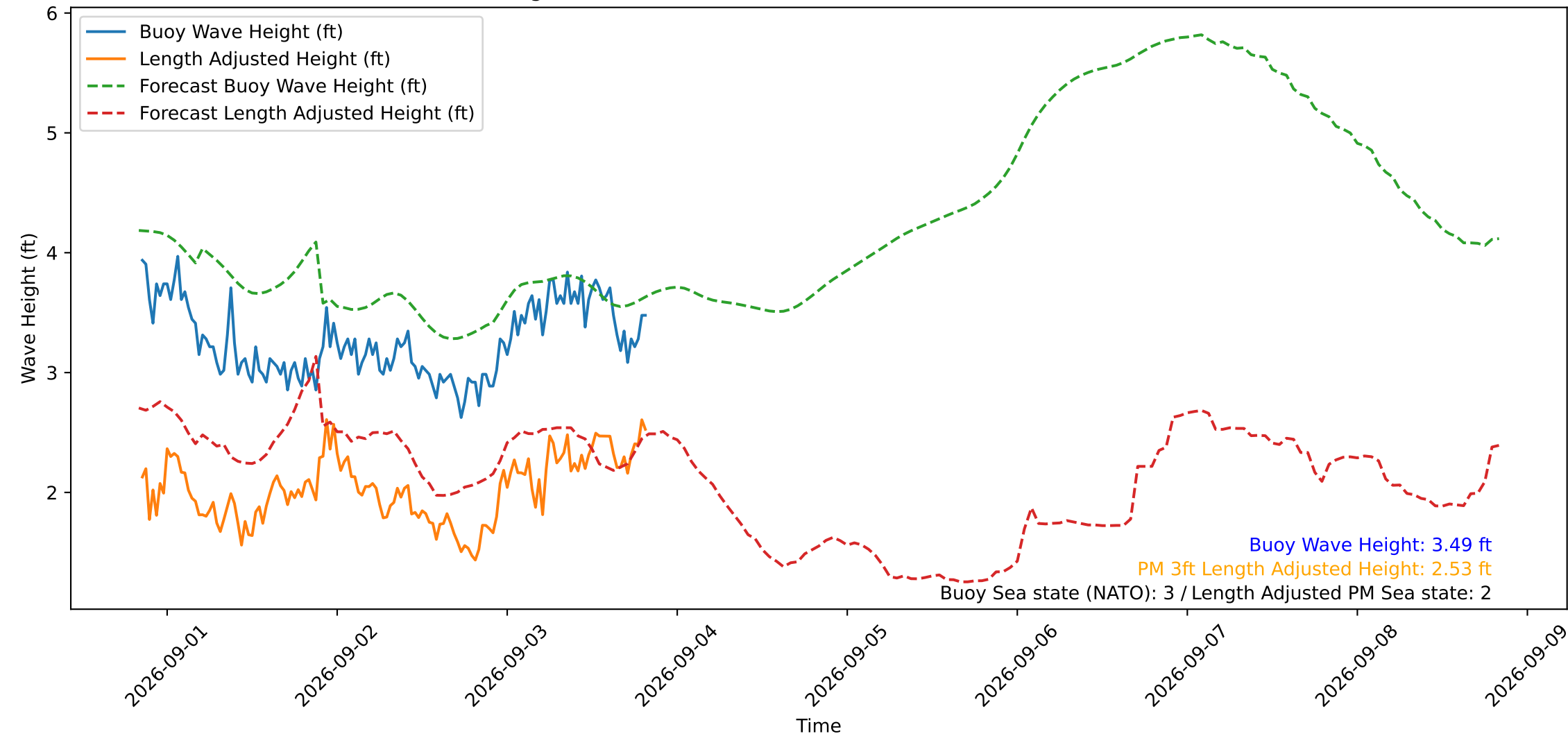
Wave Heights over Time for Oceanside Harbor at 2026-09-03 20:20:30
