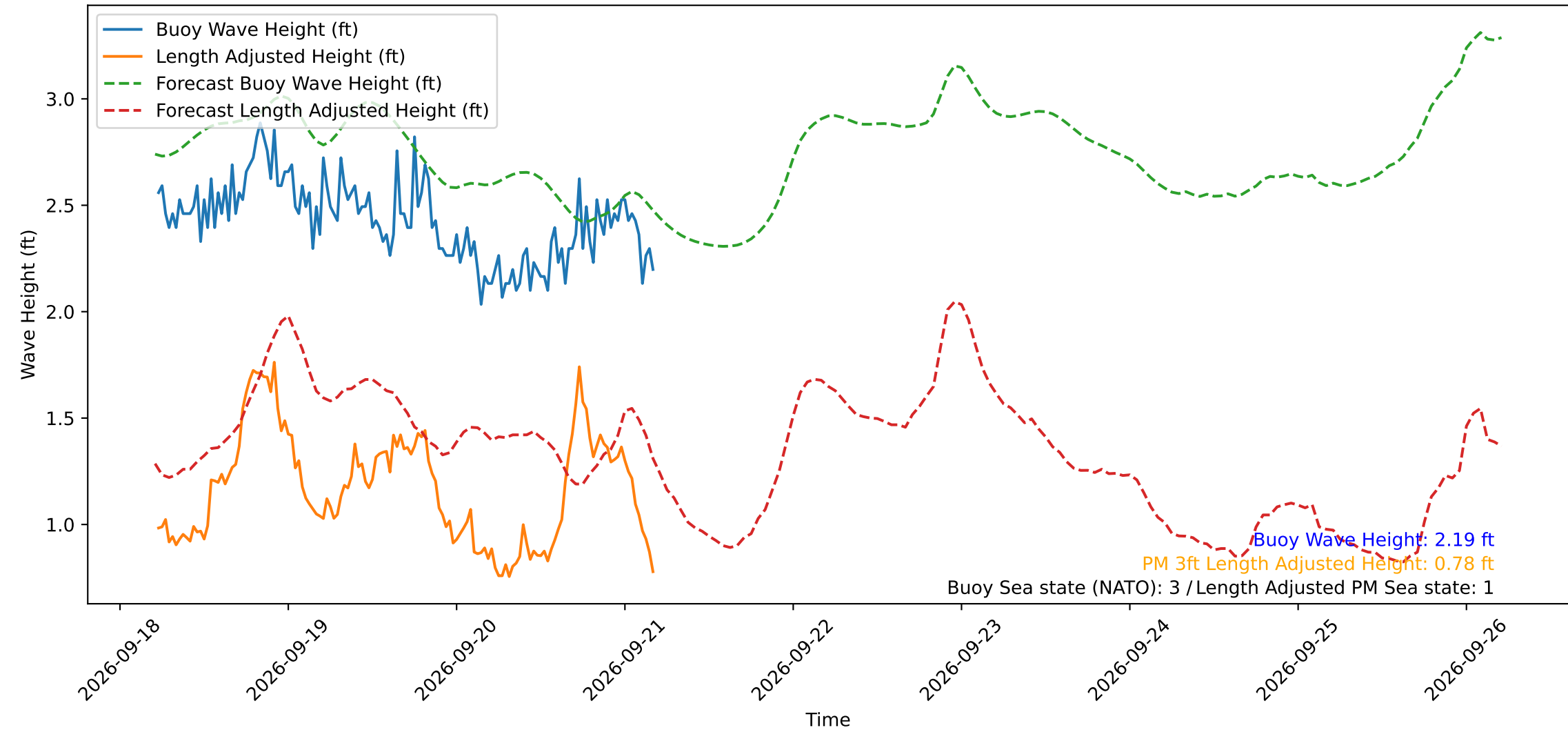
Wave Heights over Time for Red Beach at 2026-09-21 05:00:48
