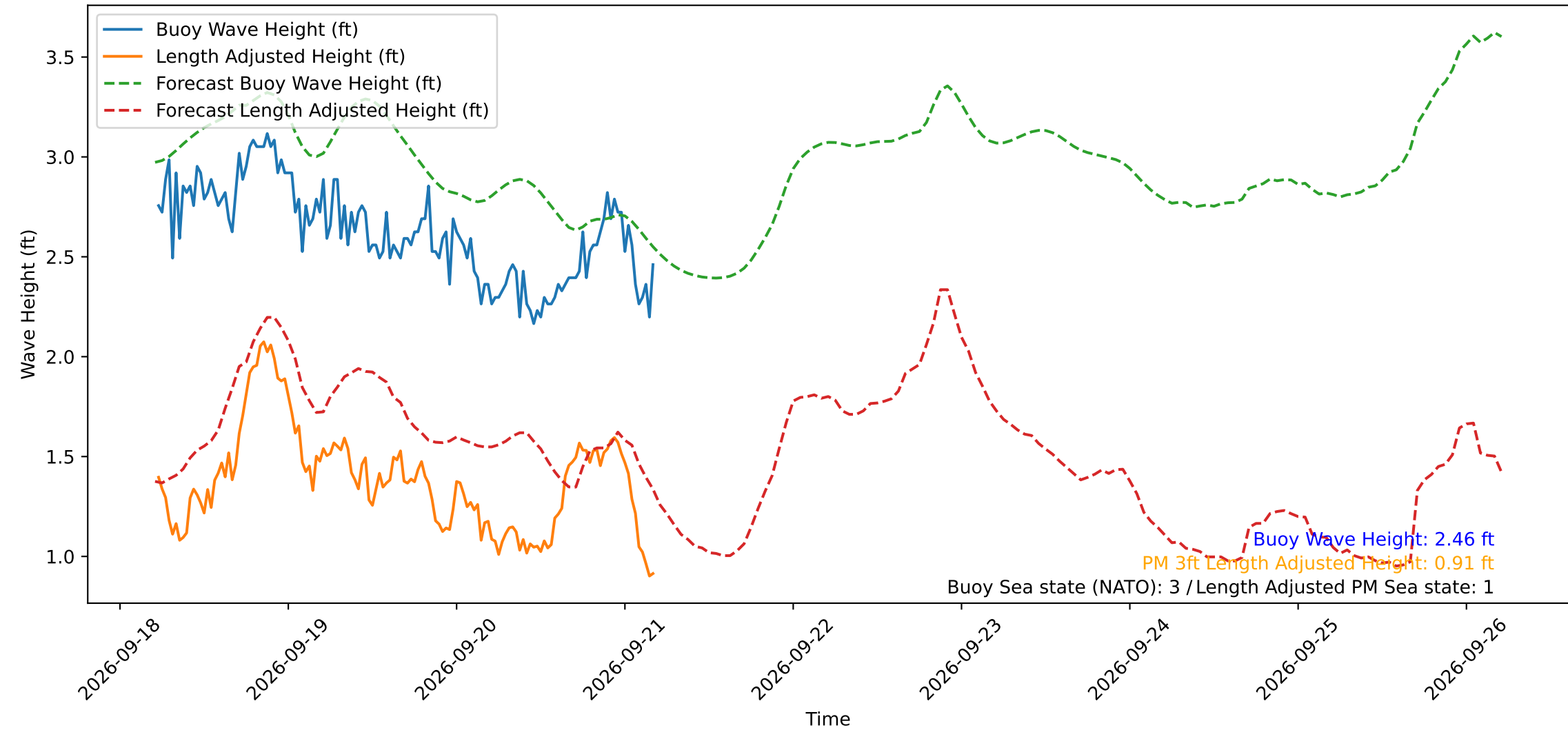
Wave Heights over Time for Green Beach at 2026-09-21 05:01:11
