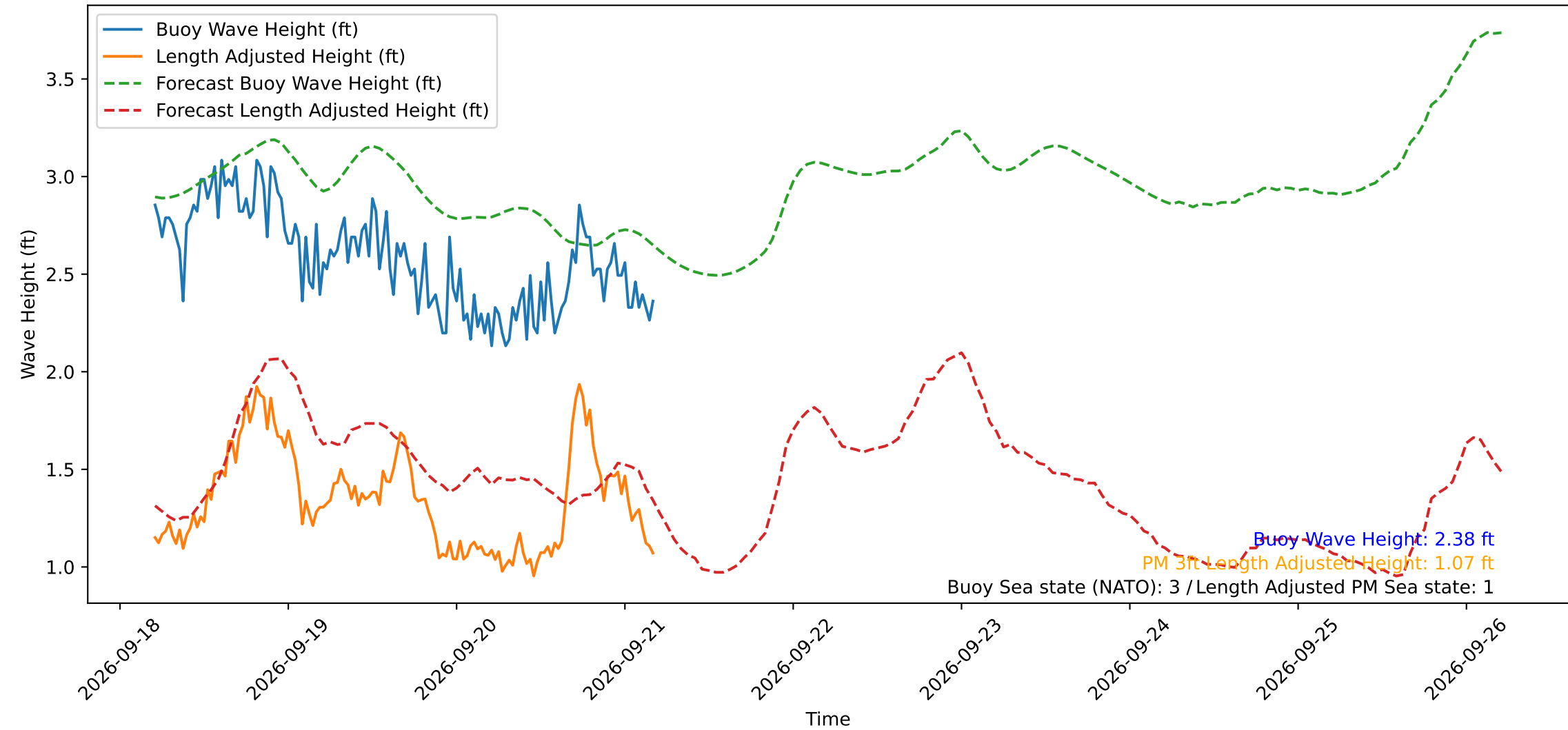
Wave Heights over Time for Oceanside Harbor at 2026-09-21 05:00:29
