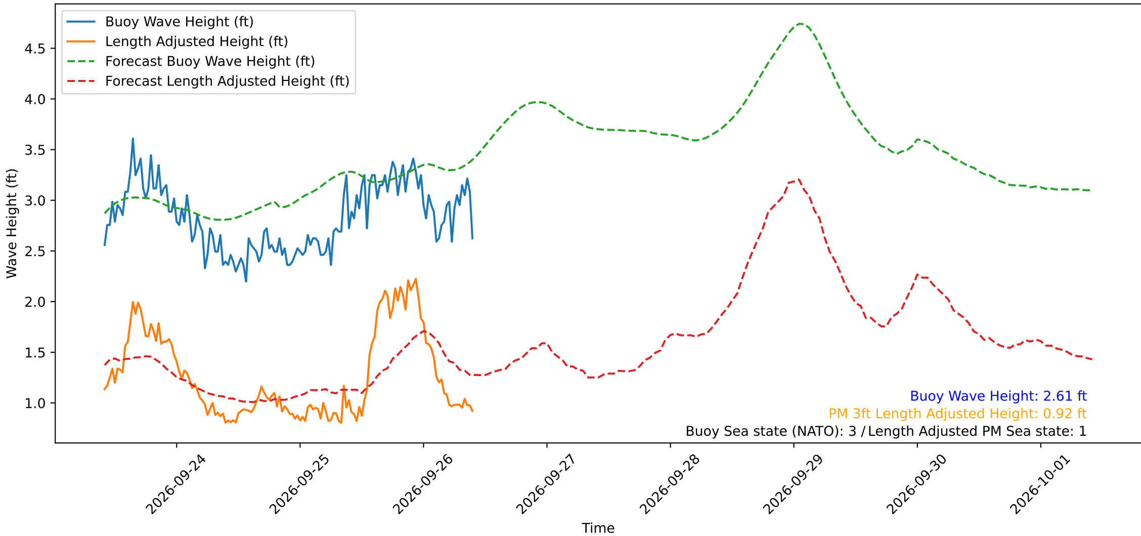
Wave Heights over Time for Oceanside Harbor at 2026-09-26 10:00:29
