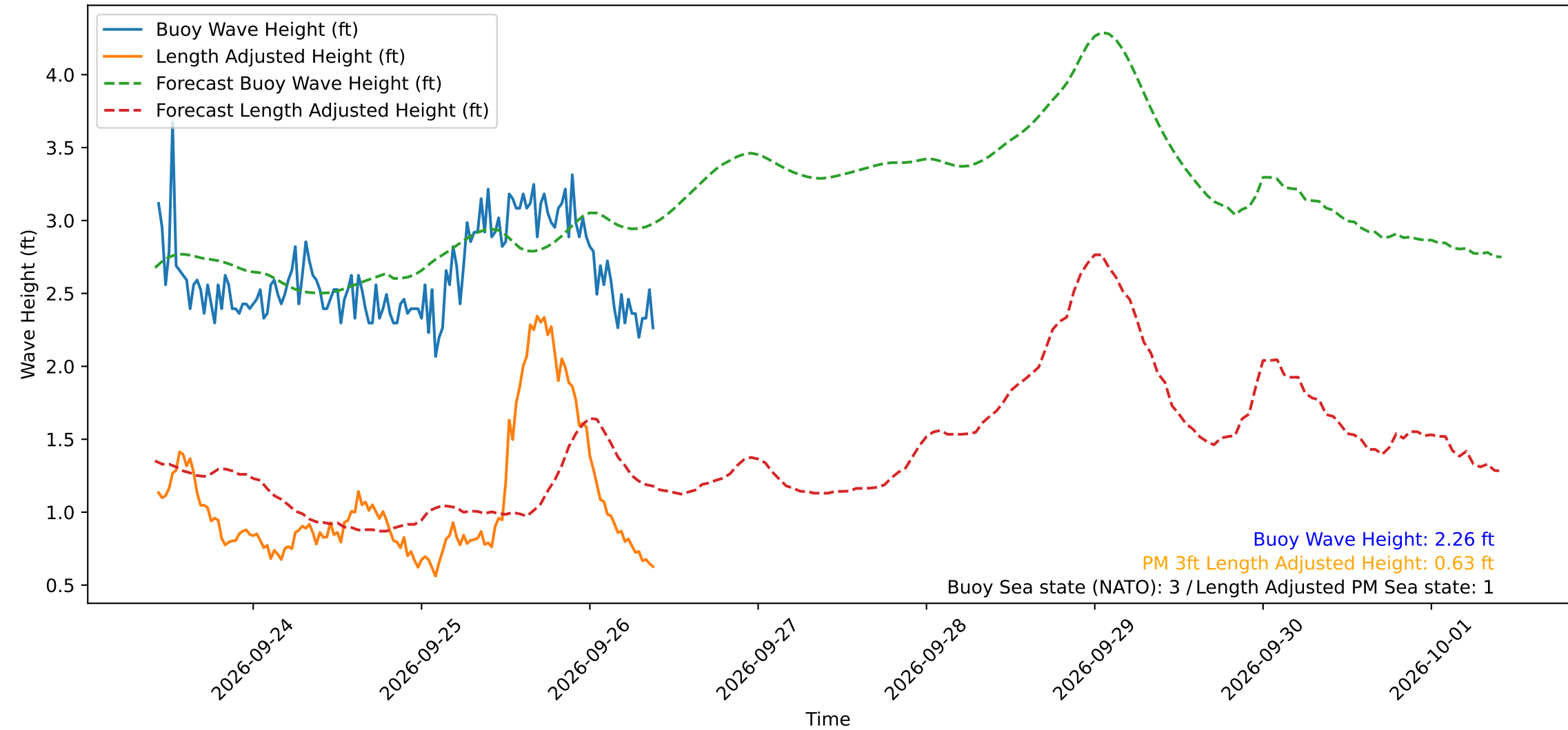
Wave Heights over Time for Red Beach at 2026-09-26 10:00:49
