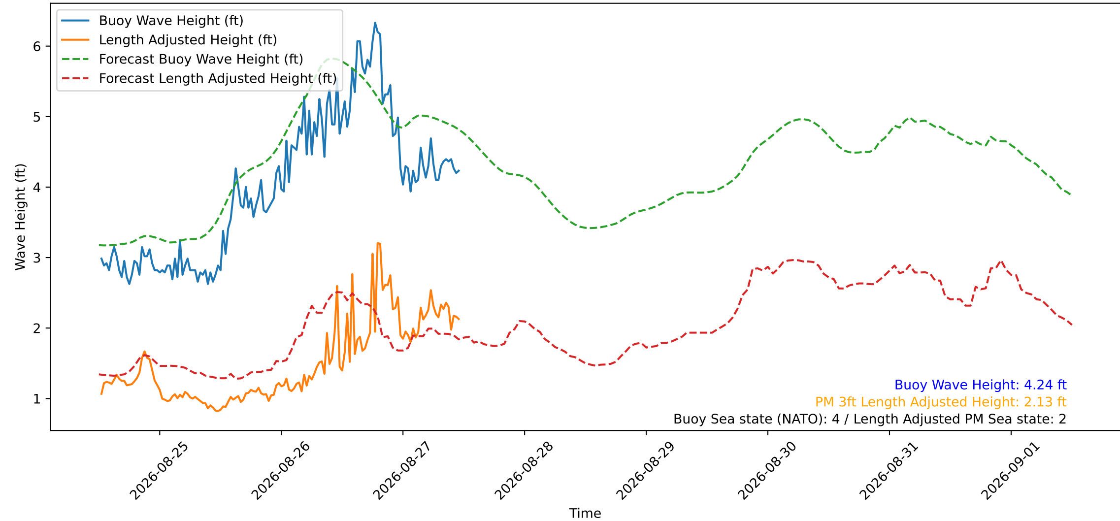
Wave Heights over Time for Green Beach at 2026-08-27 12:11:11
