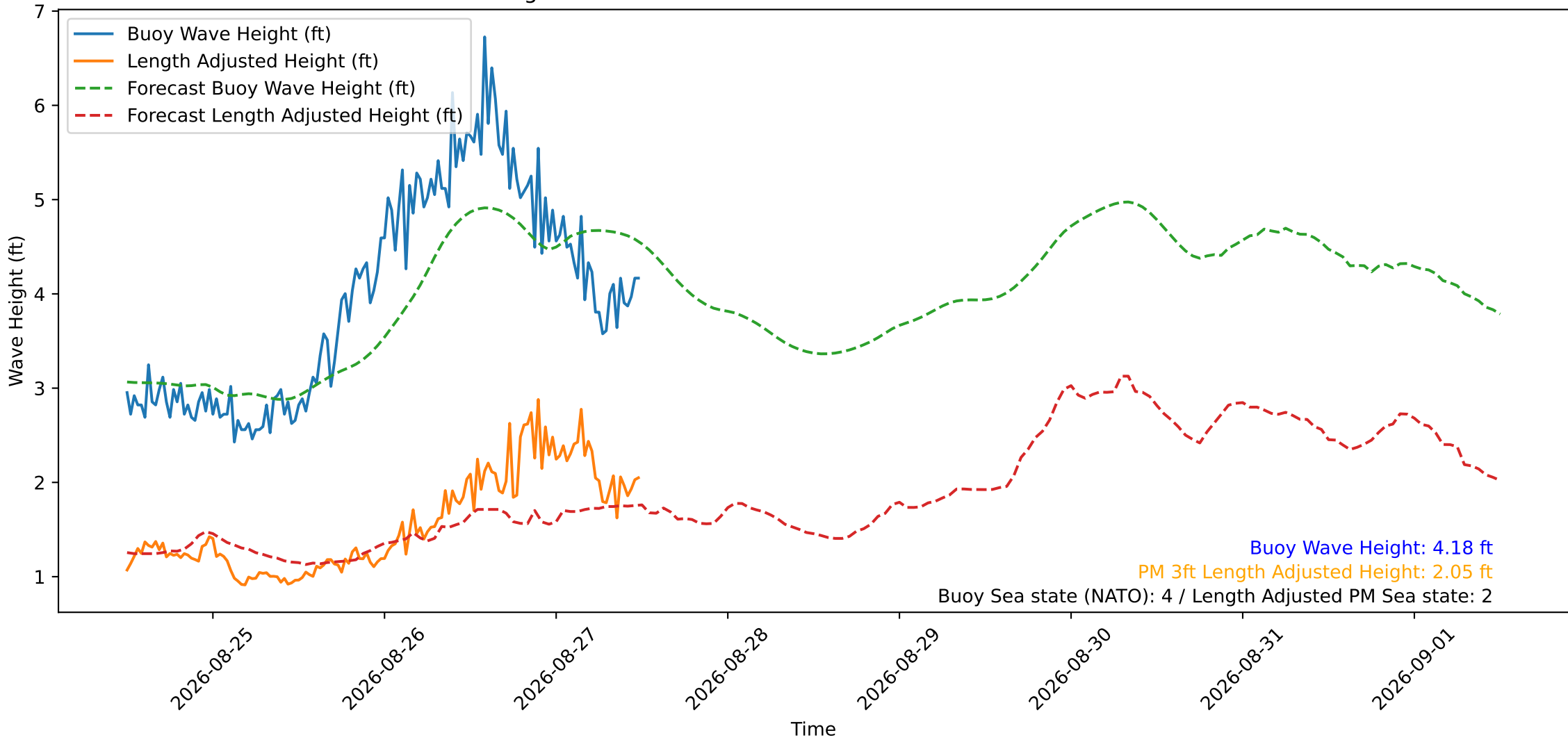
Wave Heights over Time for Oceanside Harbor at 2026-08-27 12:10:29
