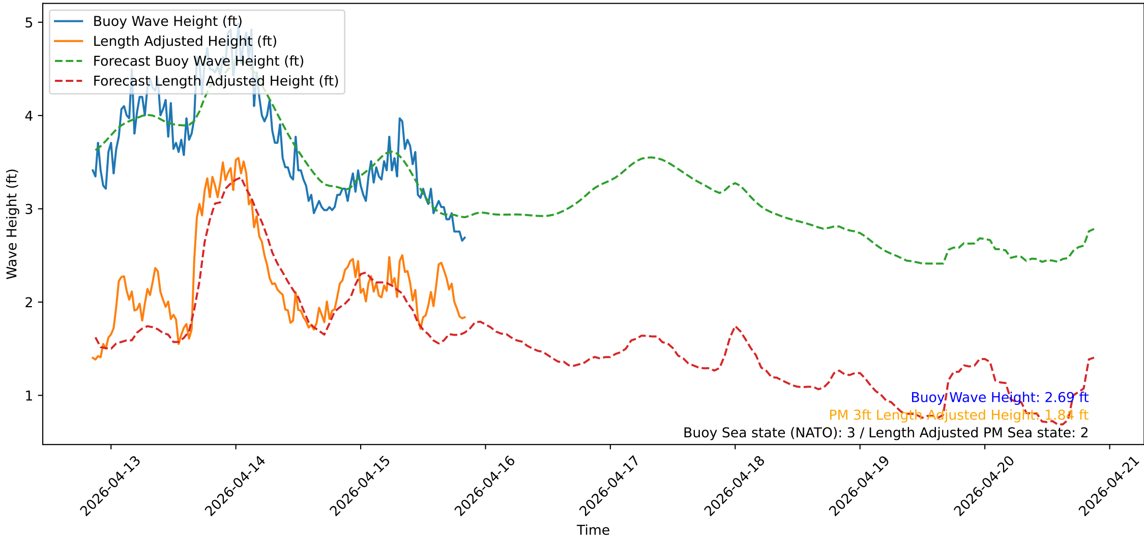
Wave Heights over Time for Green Beach at 2026-04-15 20:41:13
