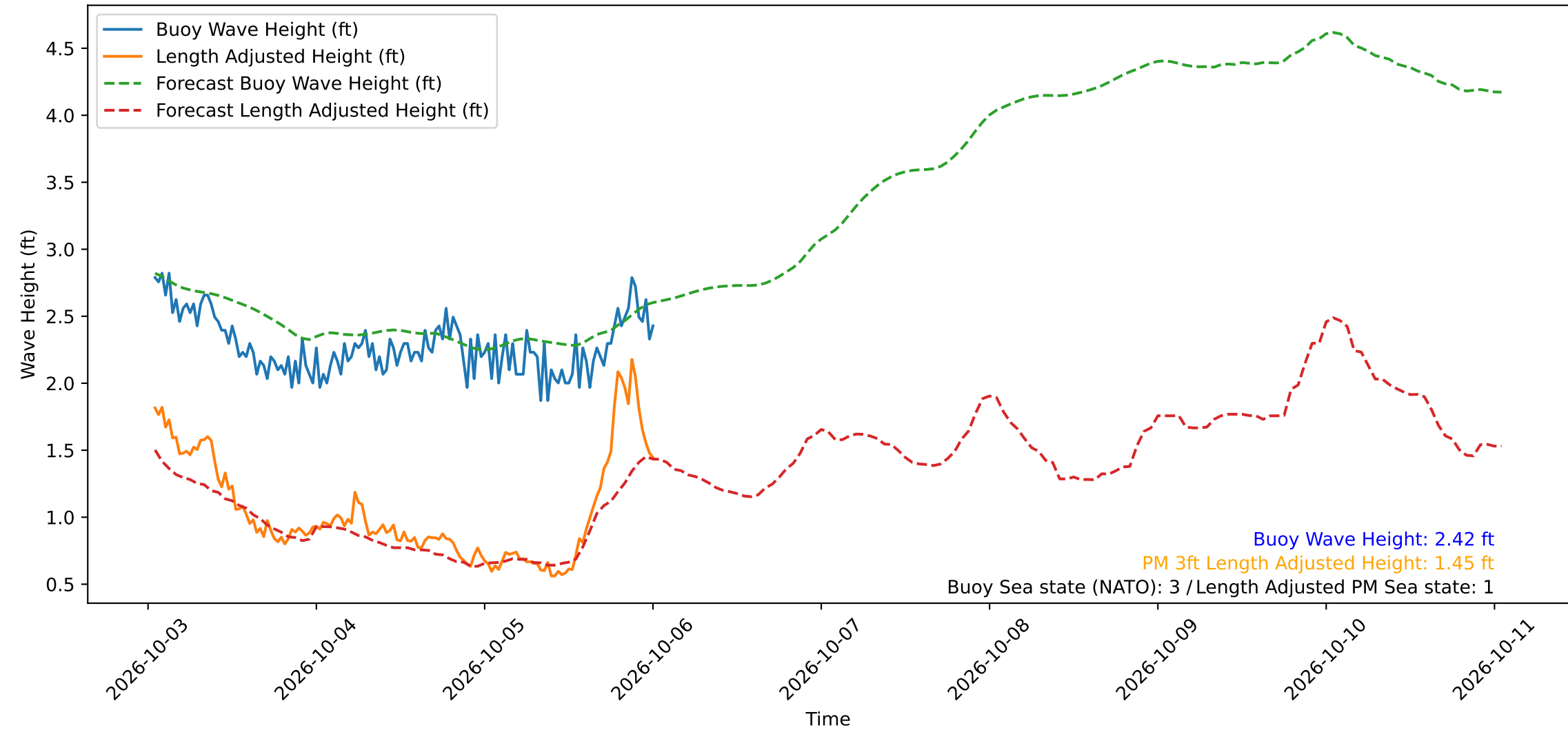
Wave Heights over Time for Oceanside Harbor at 2026-10-06 00:50:30
