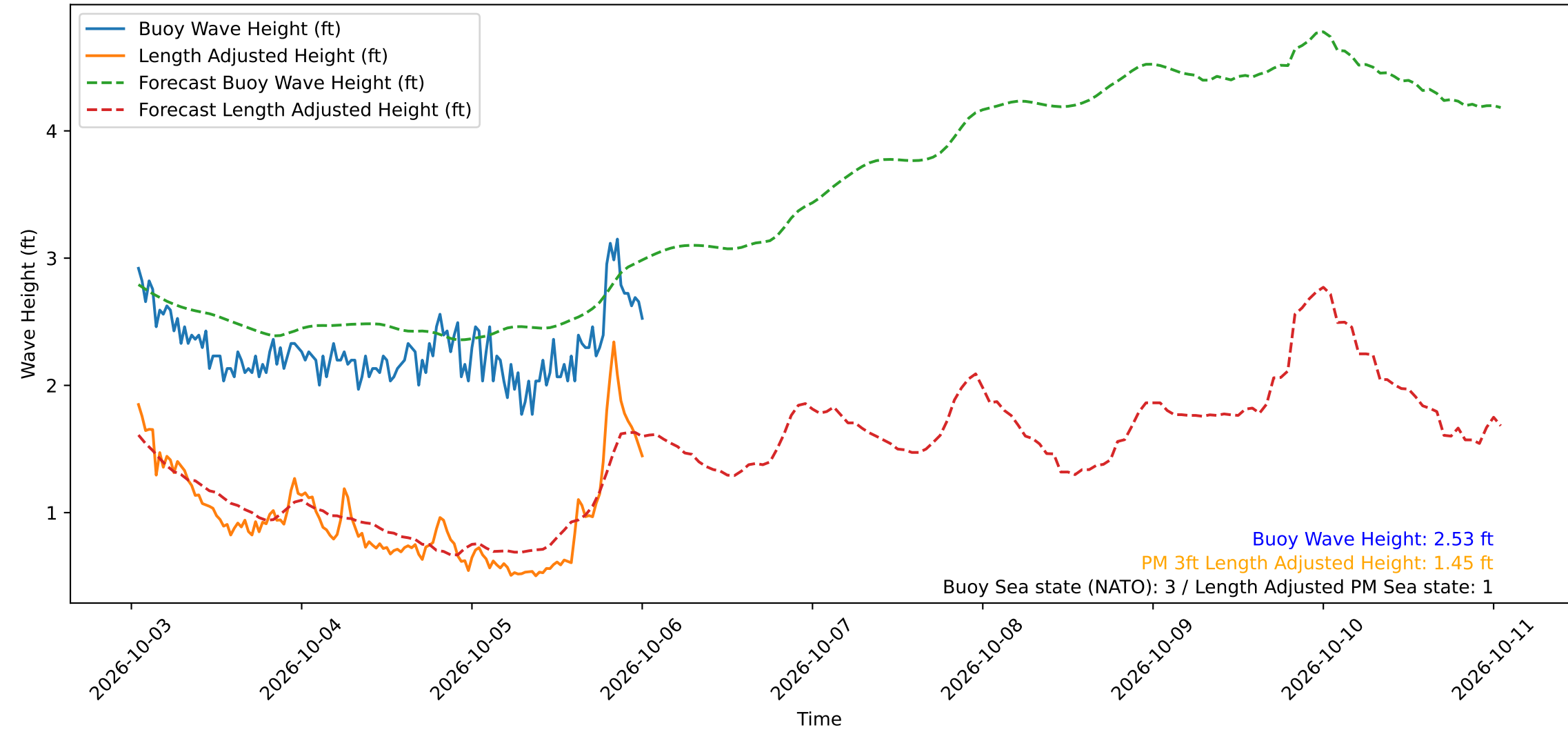
Wave Heights over Time for Green Beach at 2026-10-06 00:51:15
