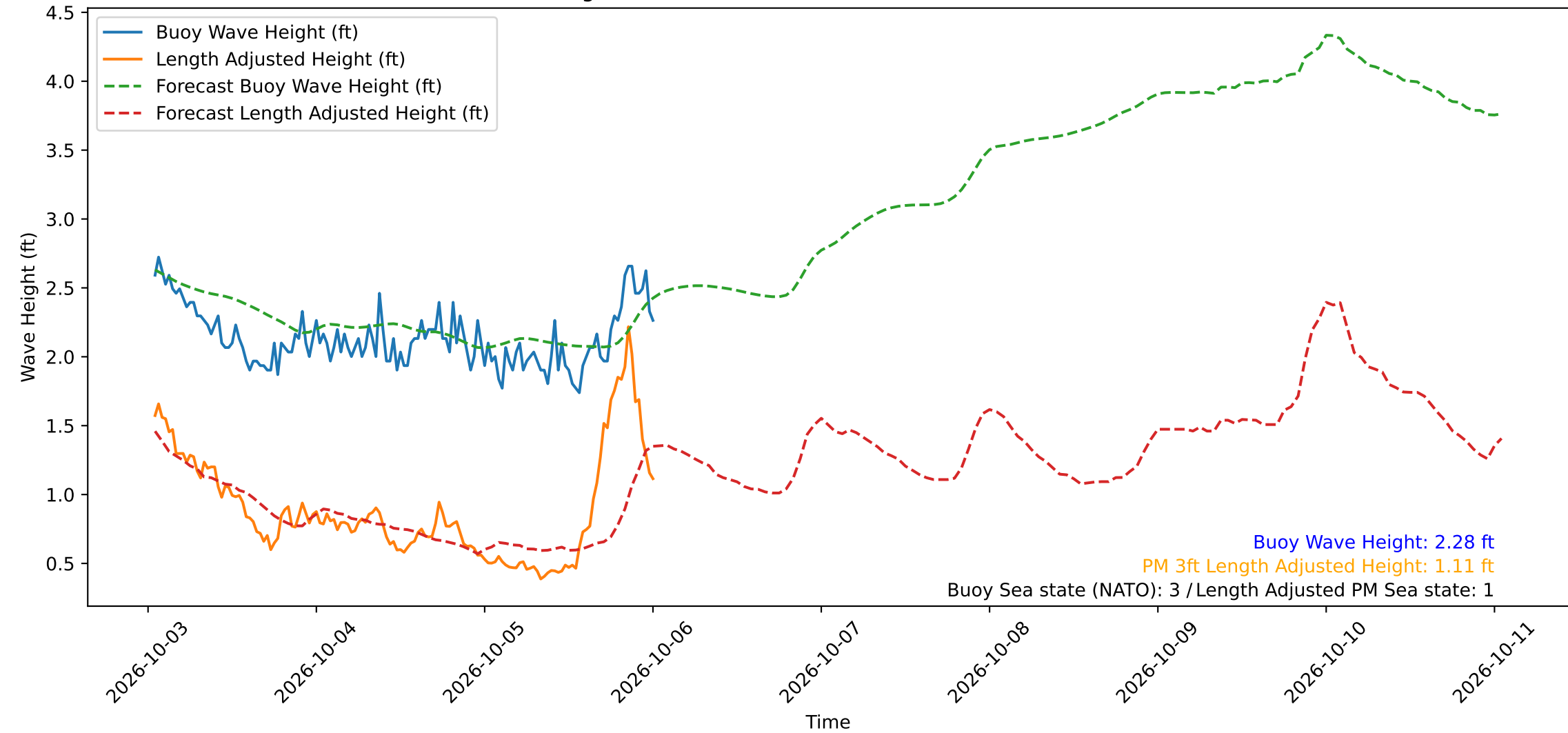
Wave Heights over Time for Red Beach at 2026-10-06 00:50:51
