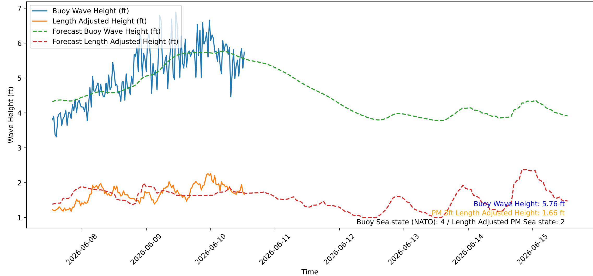
Wave Heights over Time for Green Beach at 2026-06-10 13:11:10
