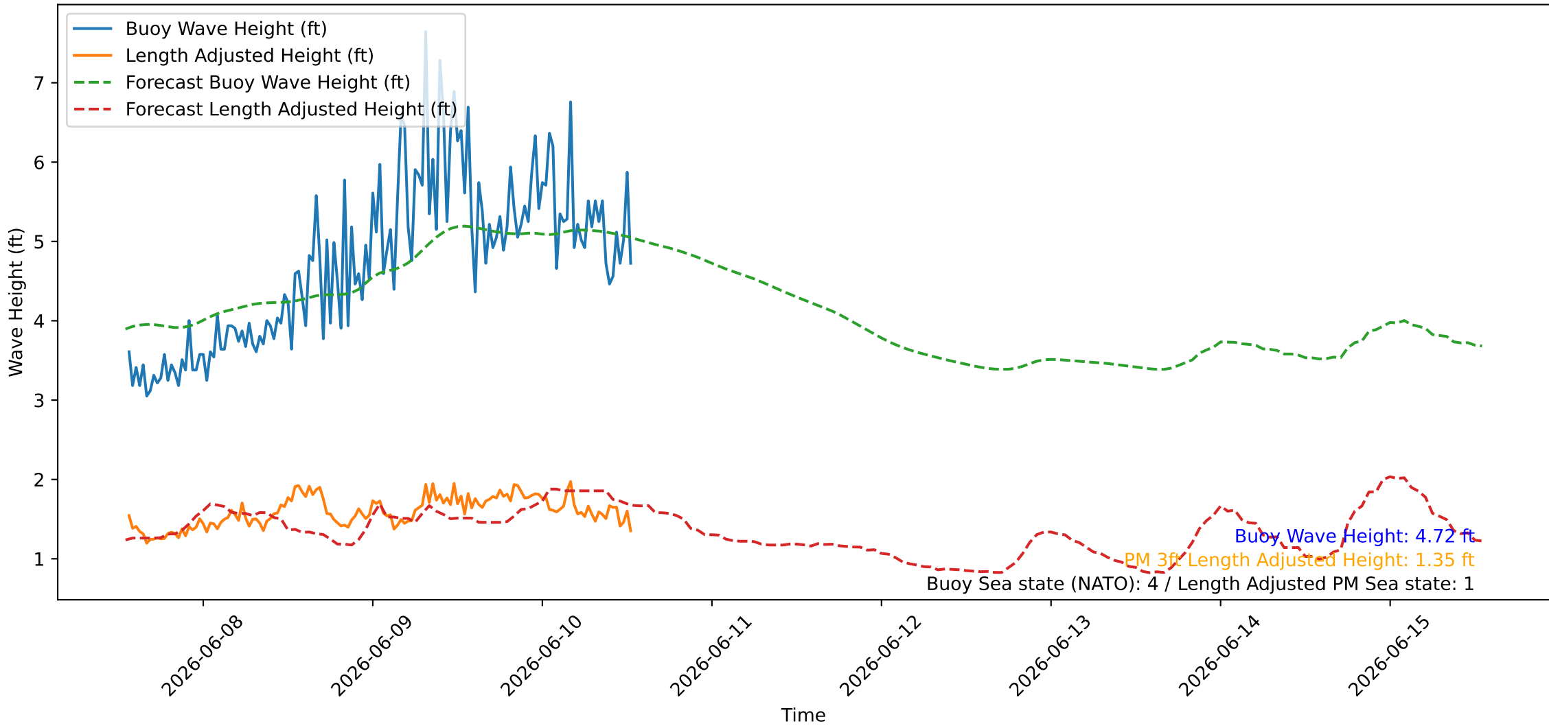
Wave Heights over Time for Red Beach at 2026-06-10 13:10:47
