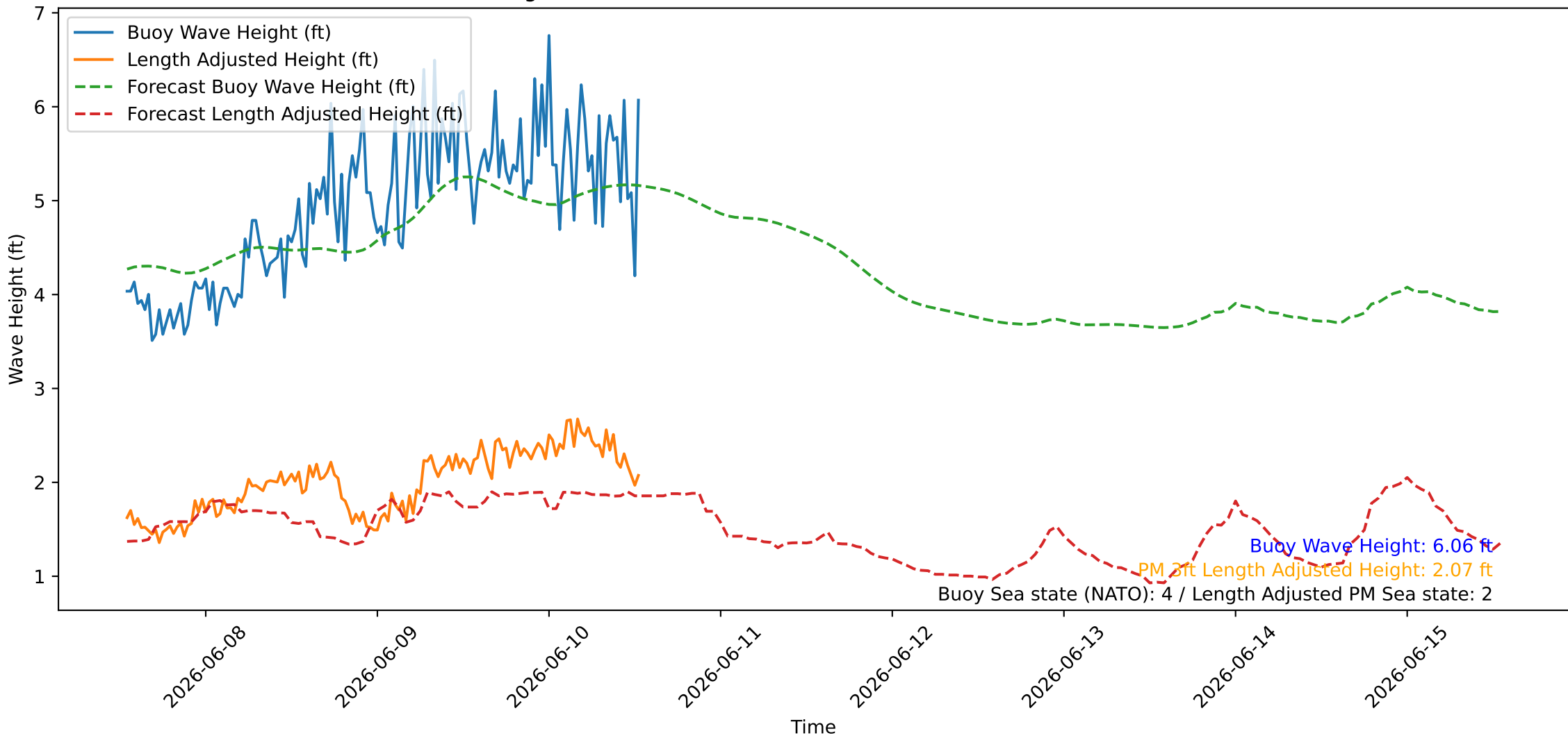
Wave Heights over Time for Oceanside Harbor at 2026-06-10 13:10:26
