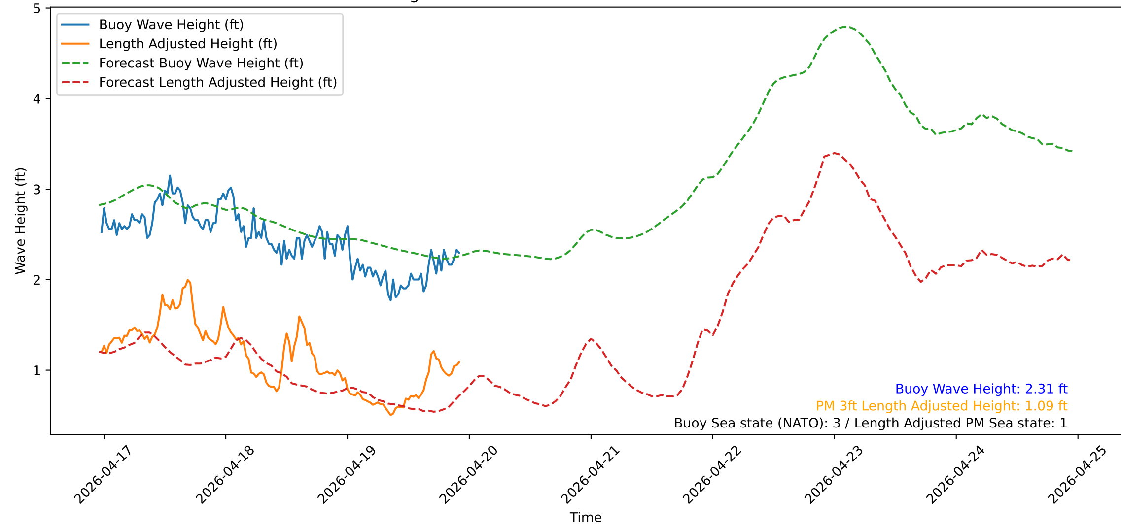
Wave Heights over Time for Red Beach at 2026-04-19 23:10:50
