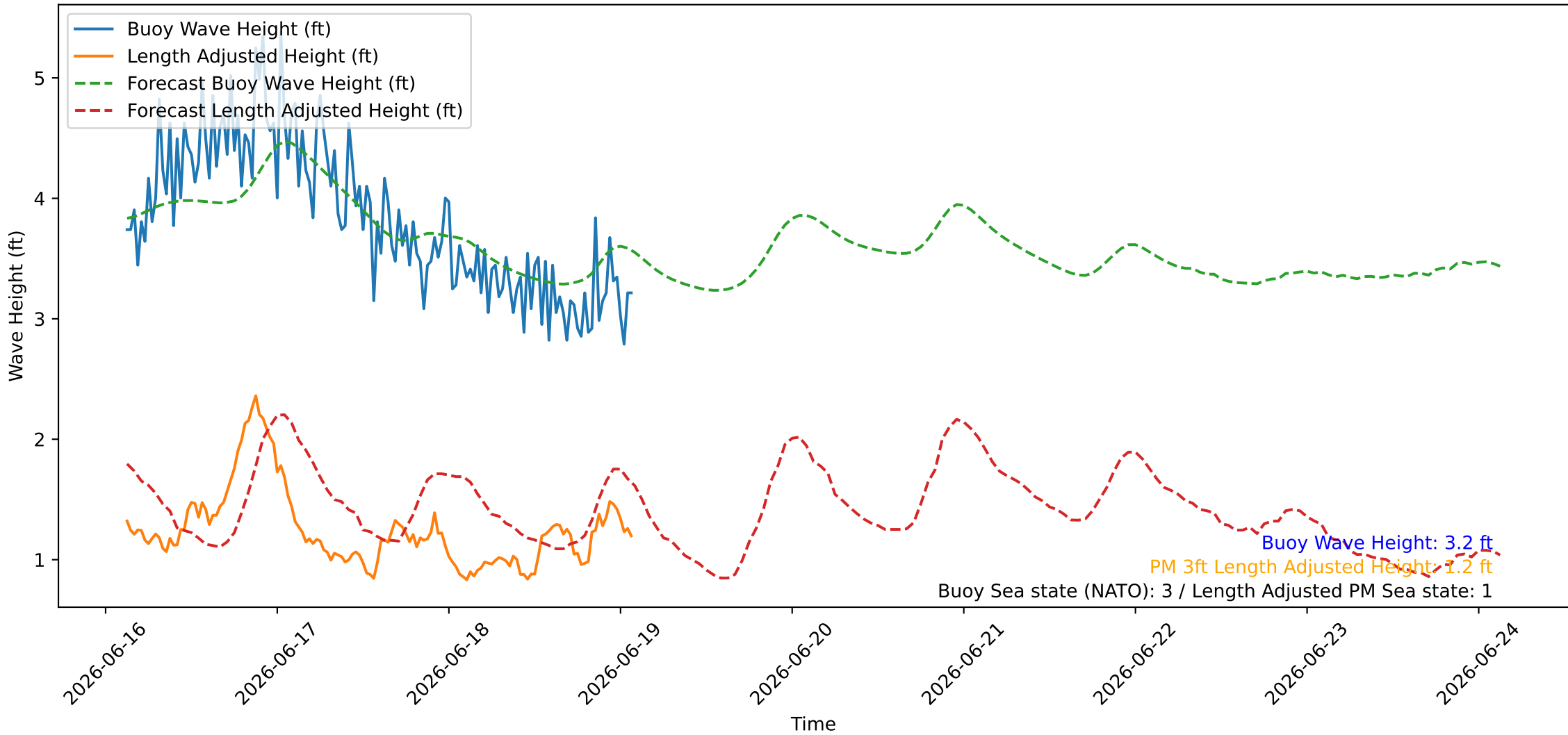
Wave Heights over Time for Red Beach at 2026-06-19 02:30:45
