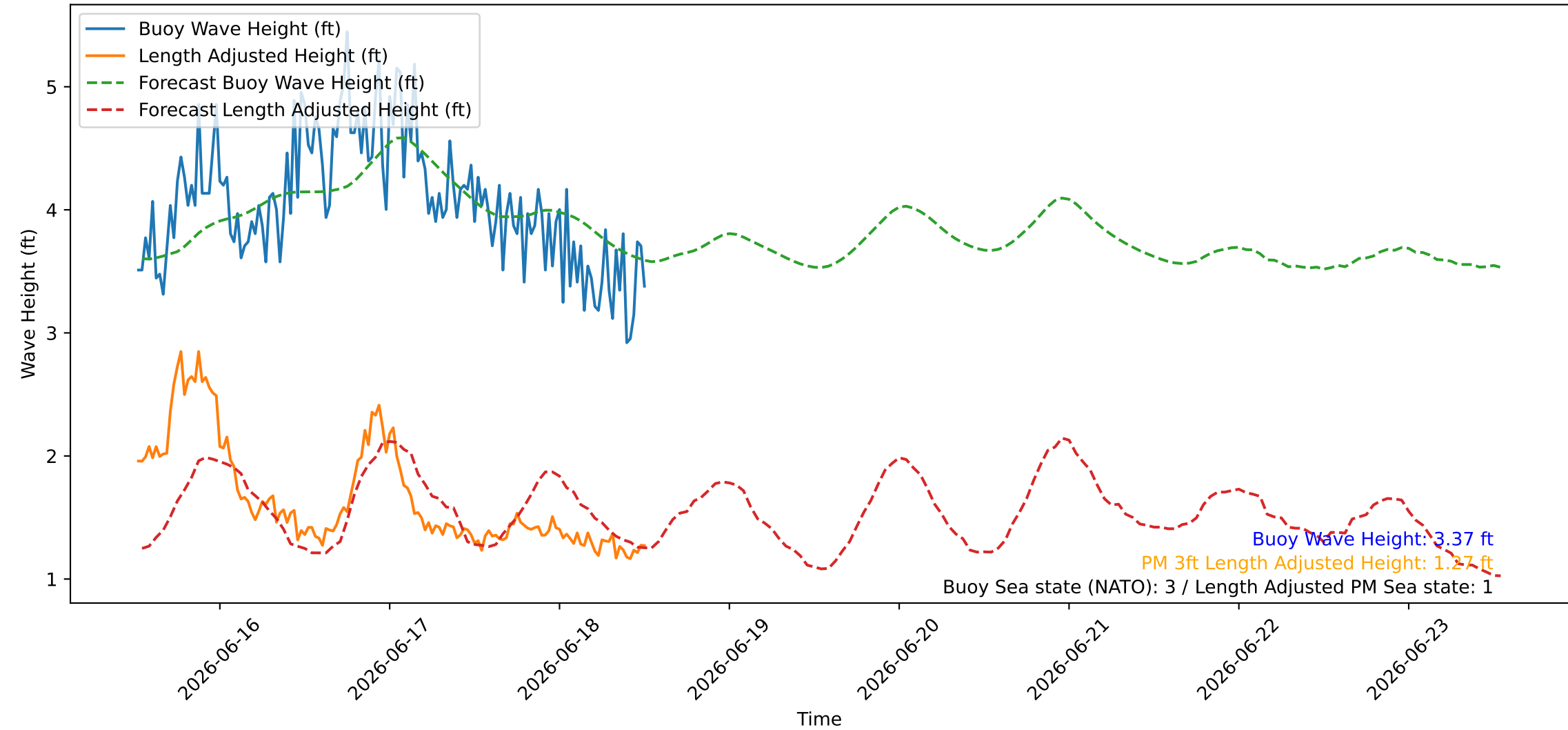
Wave Heights over Time for Oceanside Harbor at 2026-06-18 12:40:26
