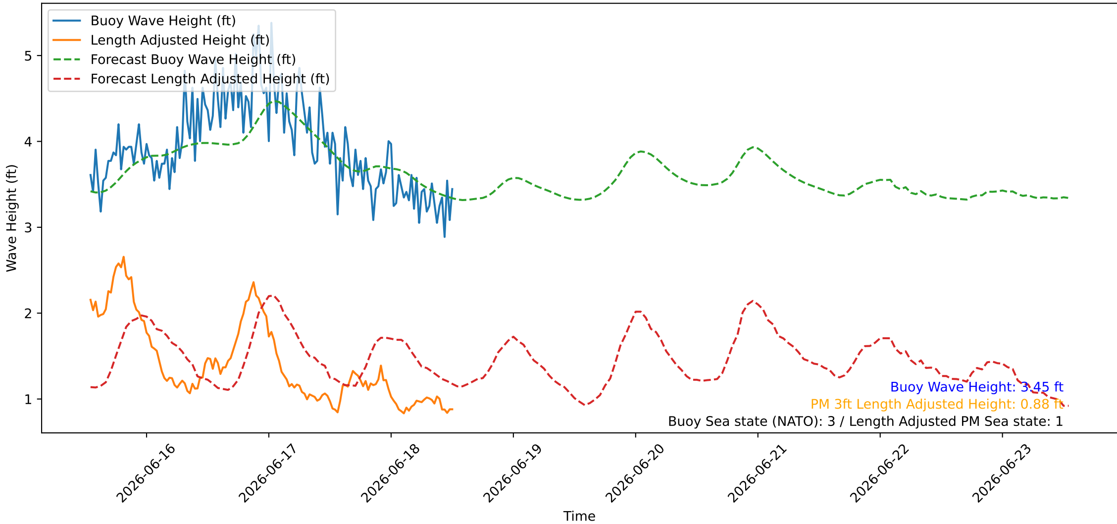
Wave Heights over Time for Red Beach at 2026-06-18 12:40:46
