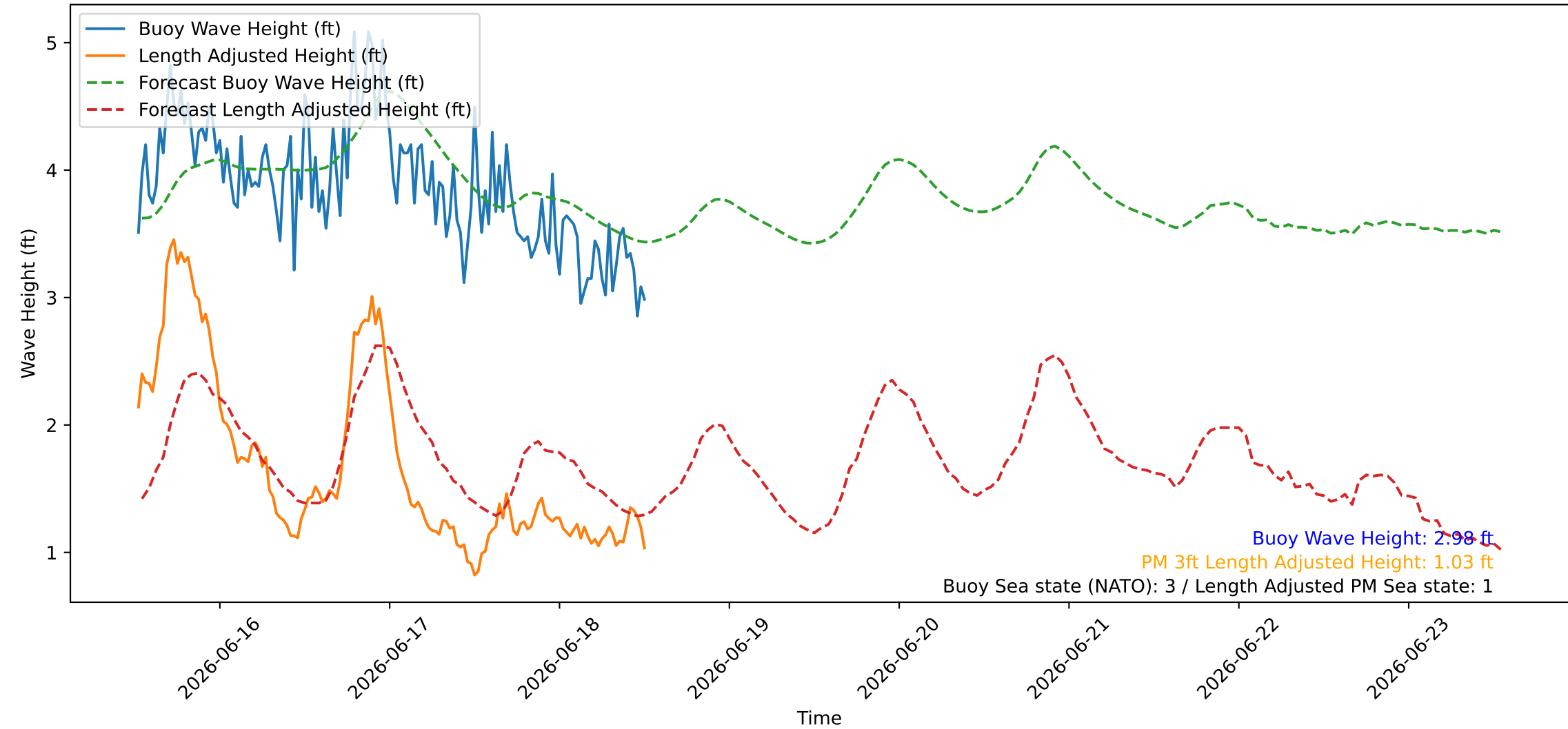
Wave Heights over Time for Green Beach at 2026-06-18 12:41:09
