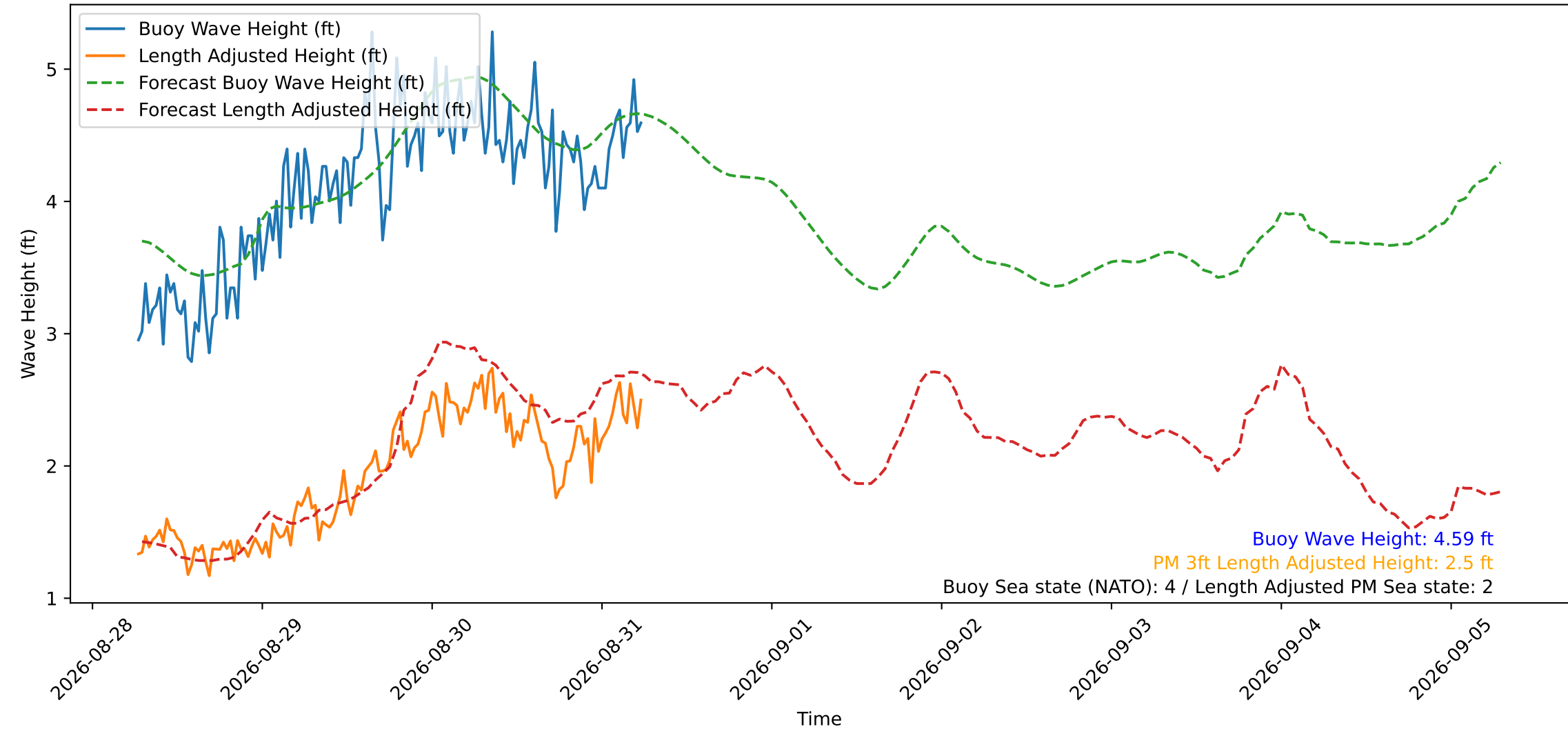
Wave Heights over Time for Oceanside Harbor at 2026-08-31 06:40:29
