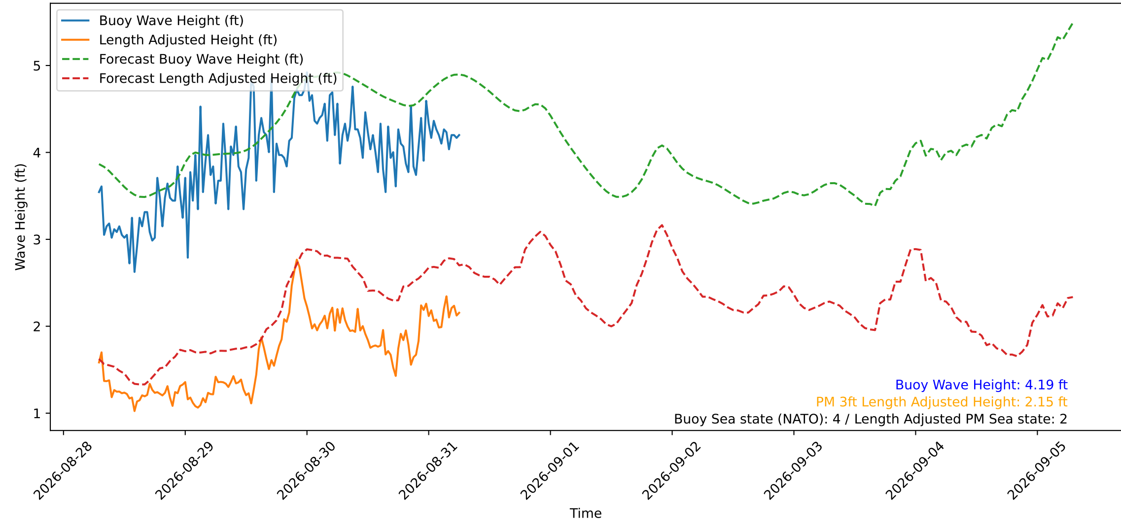
Wave Heights over Time for Green Beach at 2026-08-31 06:41:12
