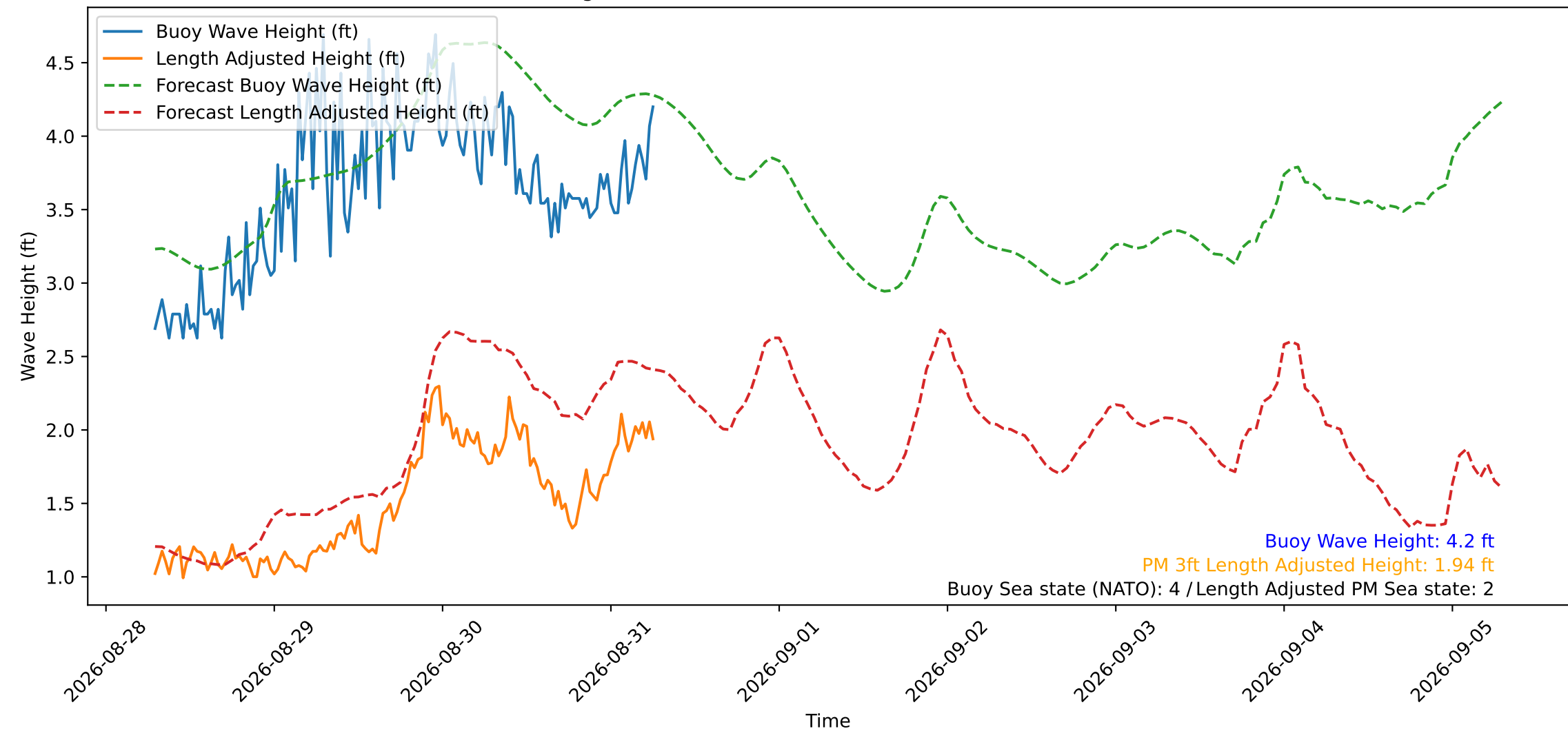
Wave Heights over Time for Red Beach at 2026-08-31 06:40:49
