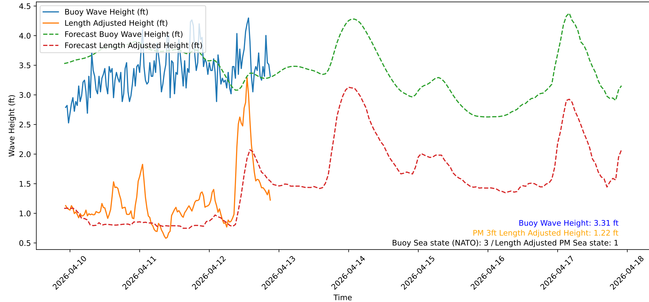
Wave Heights over Time for Red Beach at 2026-04-12 22:00:50
