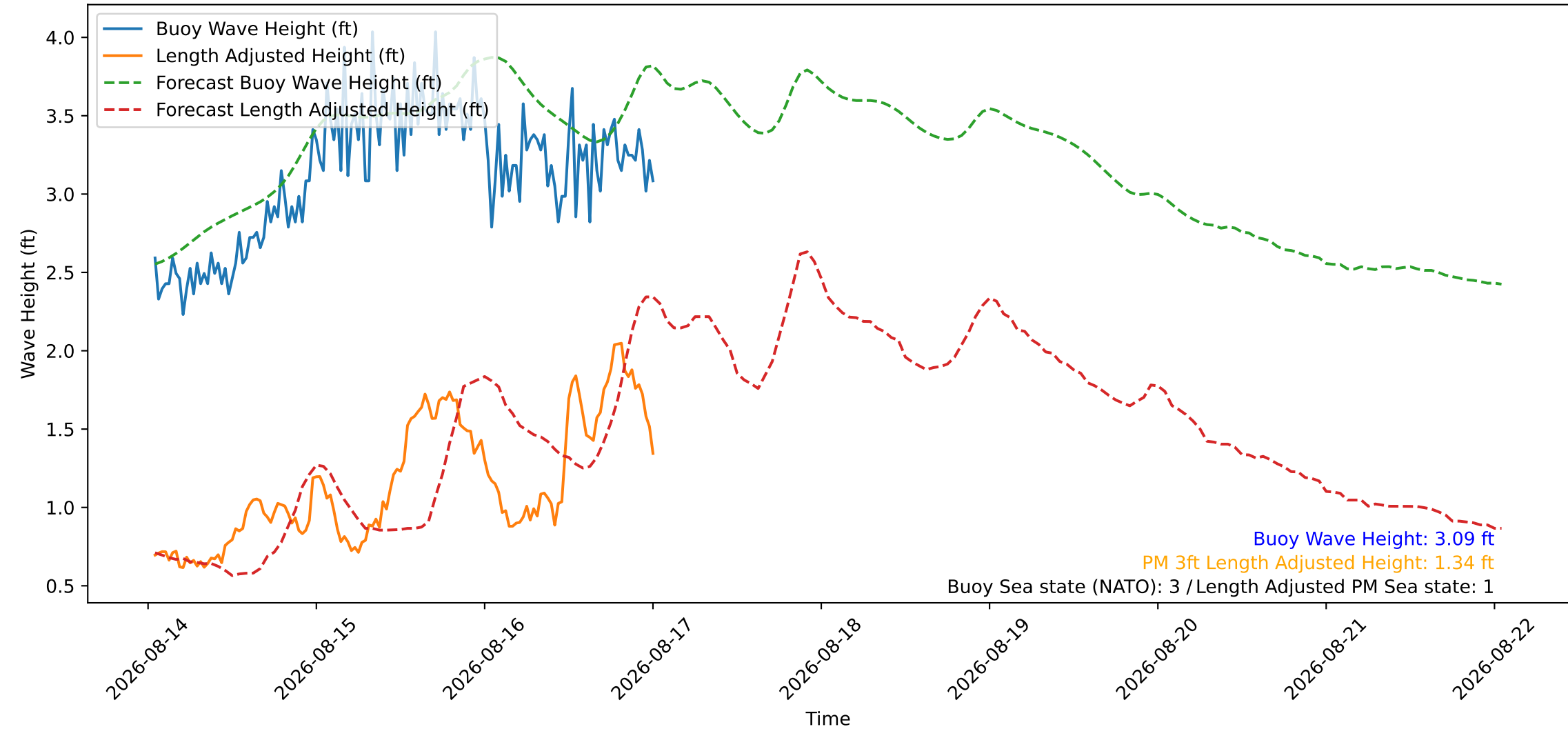
Wave Heights over Time for Red Beach at 2026-08-17 00:50:46
