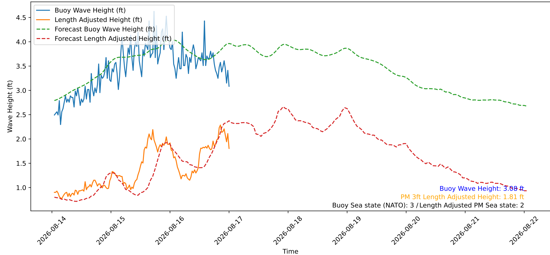
Wave Heights over Time for Oceanside Harbor at 2026-08-17 00:50:25
