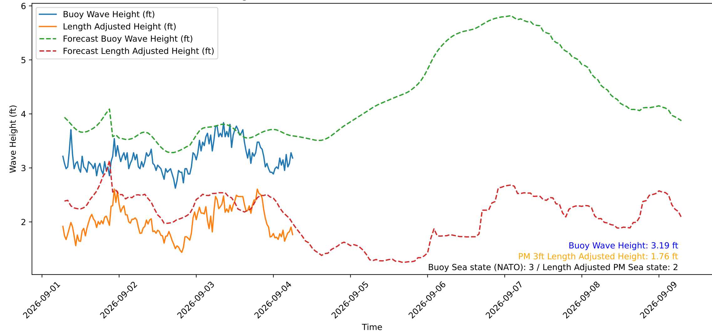
Wave Heights over Time for Oceanside Harbor at 2026-09-04 06:40:30
