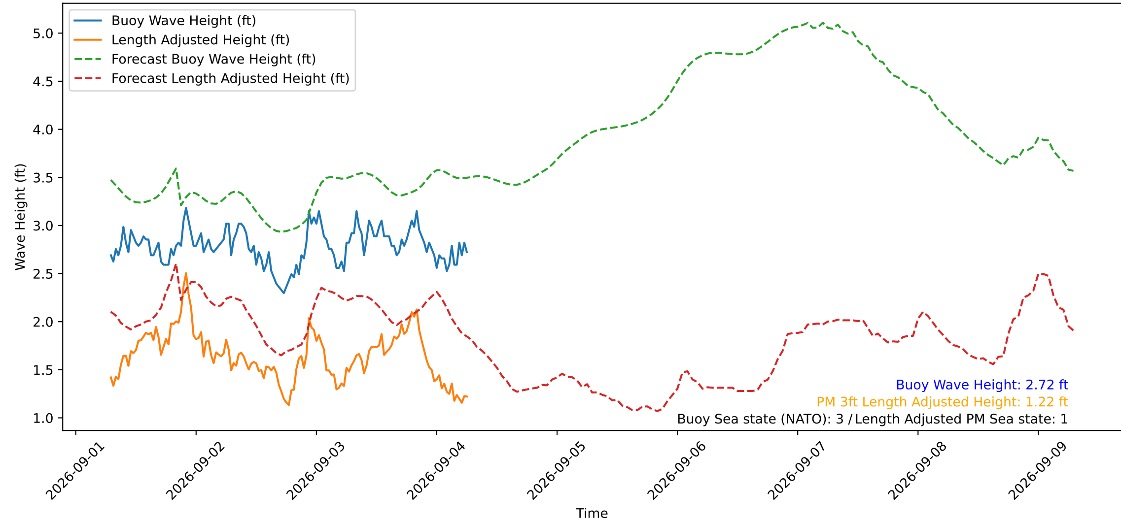
Wave Heights over Time for Red Beach at 2026-09-04 06:40:50
