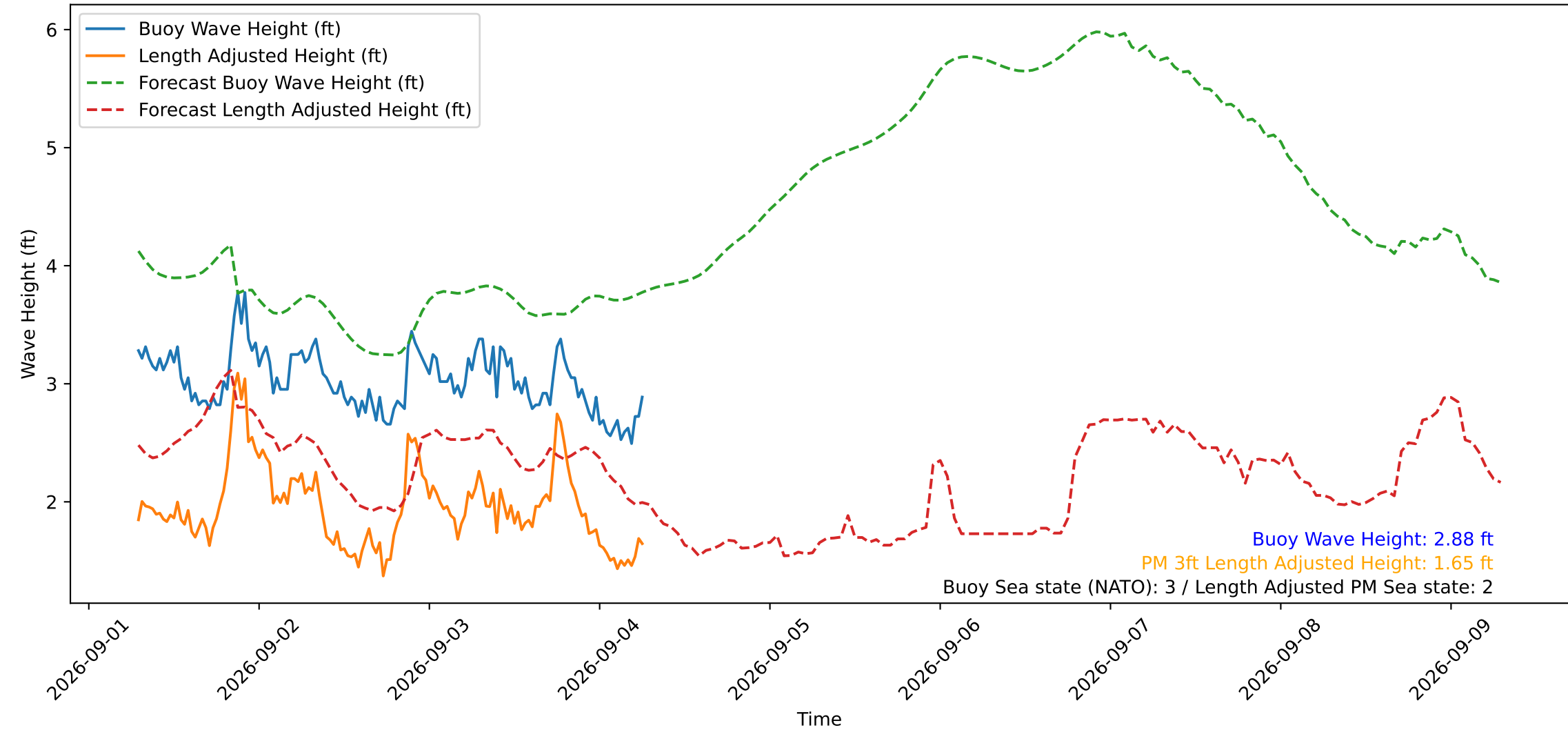
Wave Heights over Time for Green Beach at 2026-09-04 06:41:13
