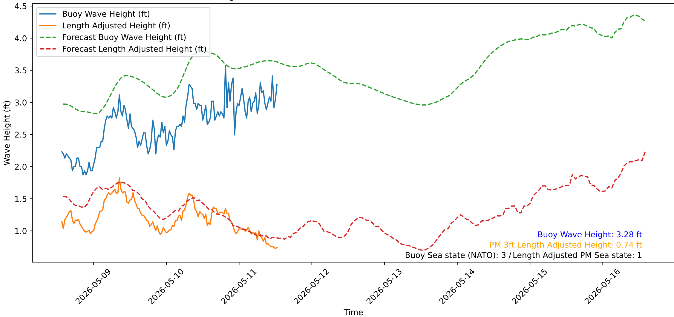
Wave Heights over Time for Oceanside Harbor at 2026-05-11 13:30:31
