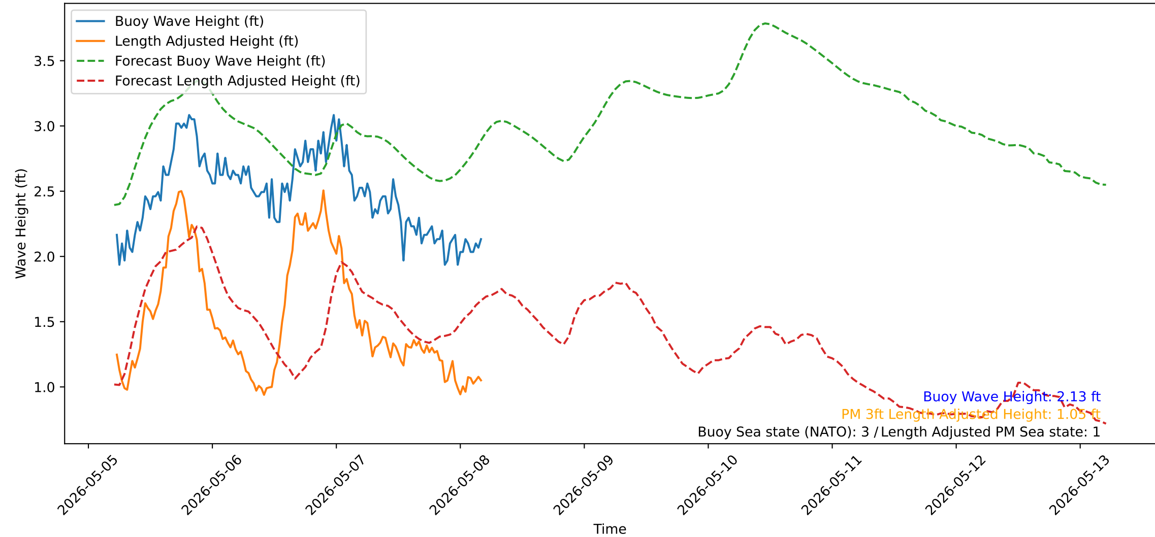
Wave Heights over Time for Red Beach at 2026-05-08 05:00:50
