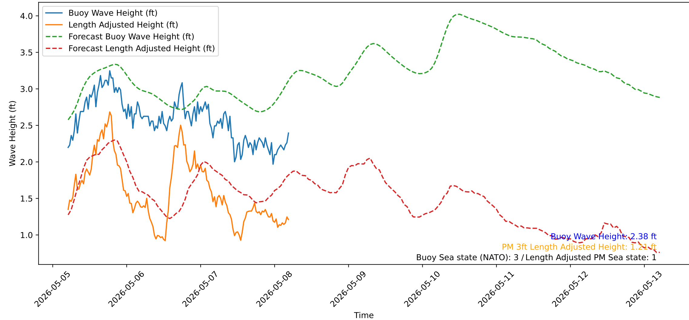
Wave Heights over Time for Oceanside Harbor at 2026-05-08 05:00:31
