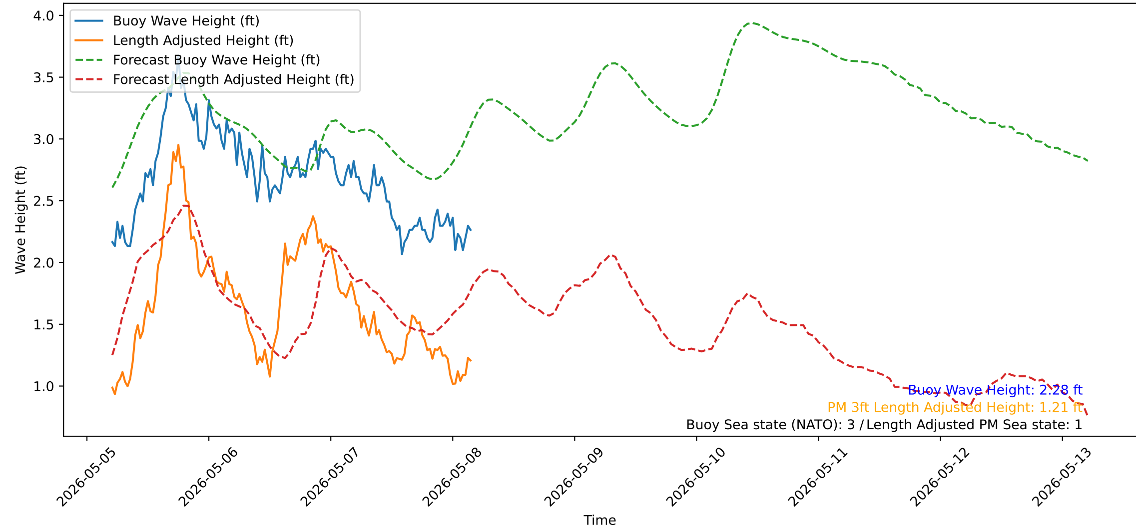
Wave Heights over Time for Green Beach at 2026-05-08 05:01:12
