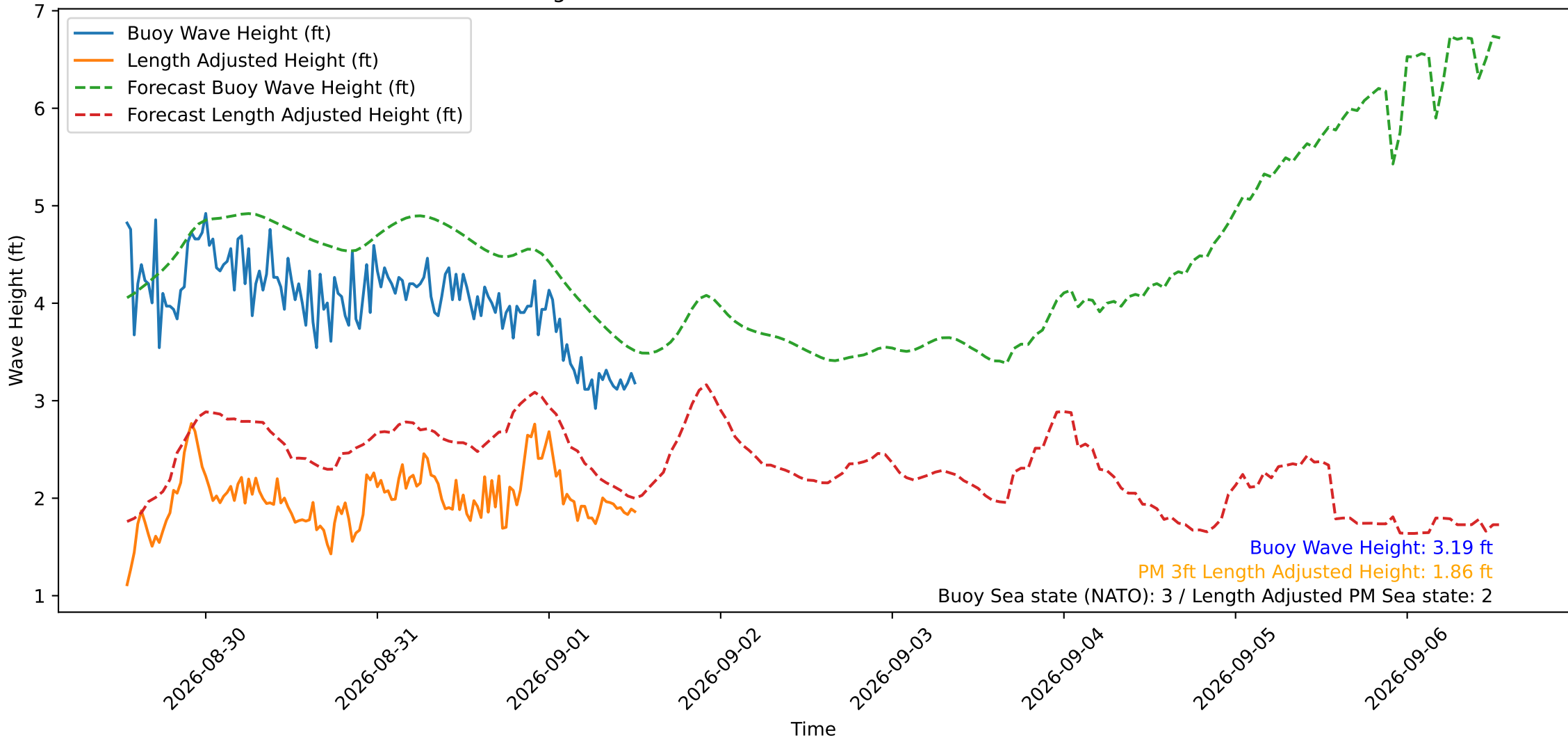
Wave Heights over Time for Green Beach at 2026-09-01 12:41:12
