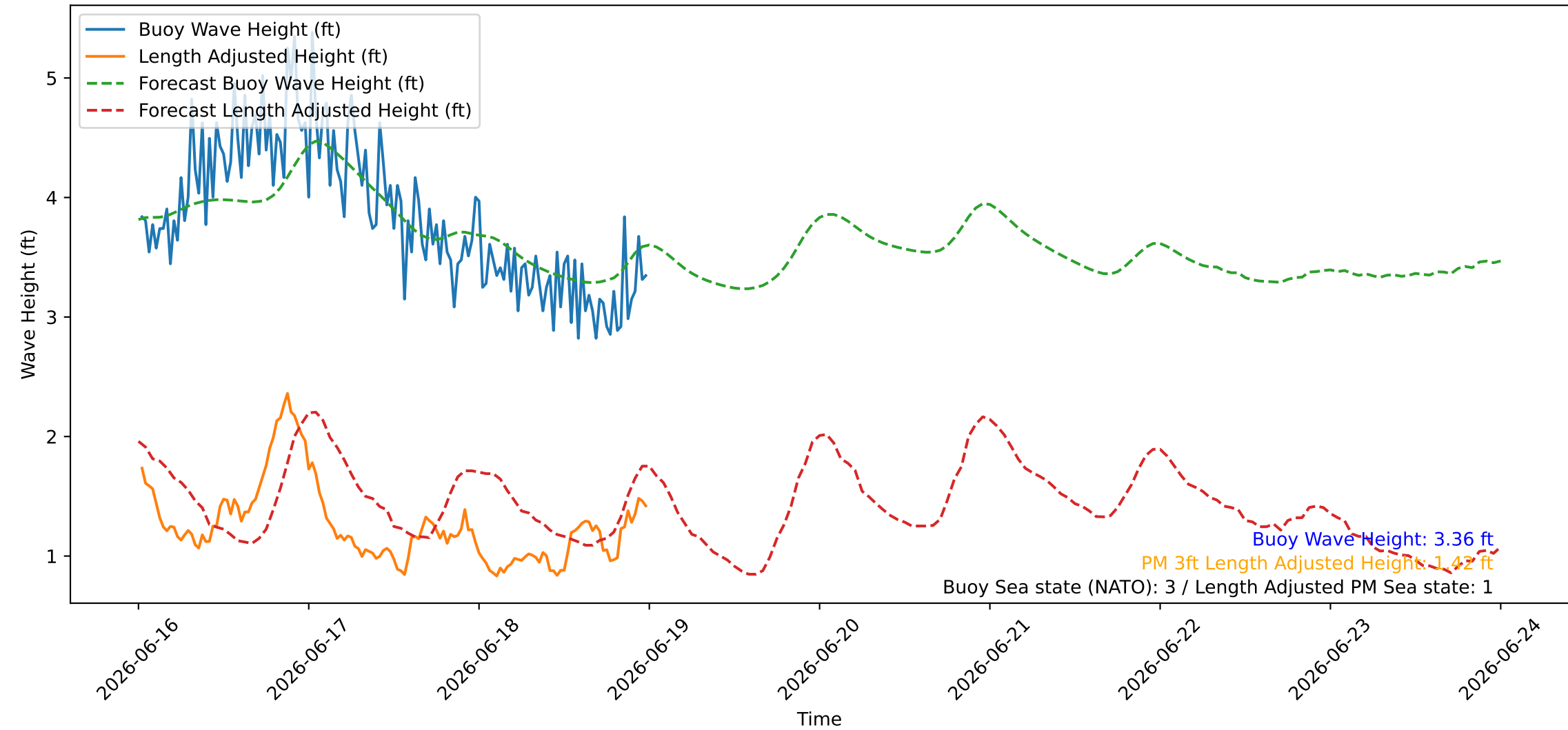
Wave Heights over Time for Red Beach at 2026-06-19 00:10:46
