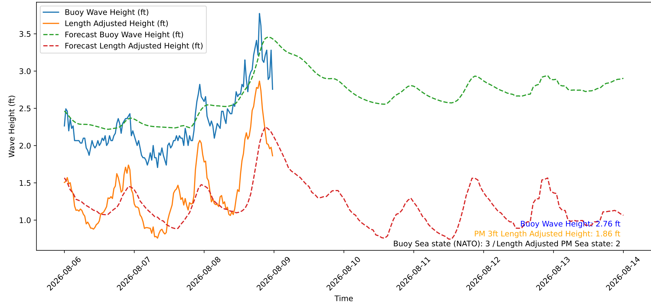
Wave Heights over Time for Green Beach at 2026-08-09 00:11:09
