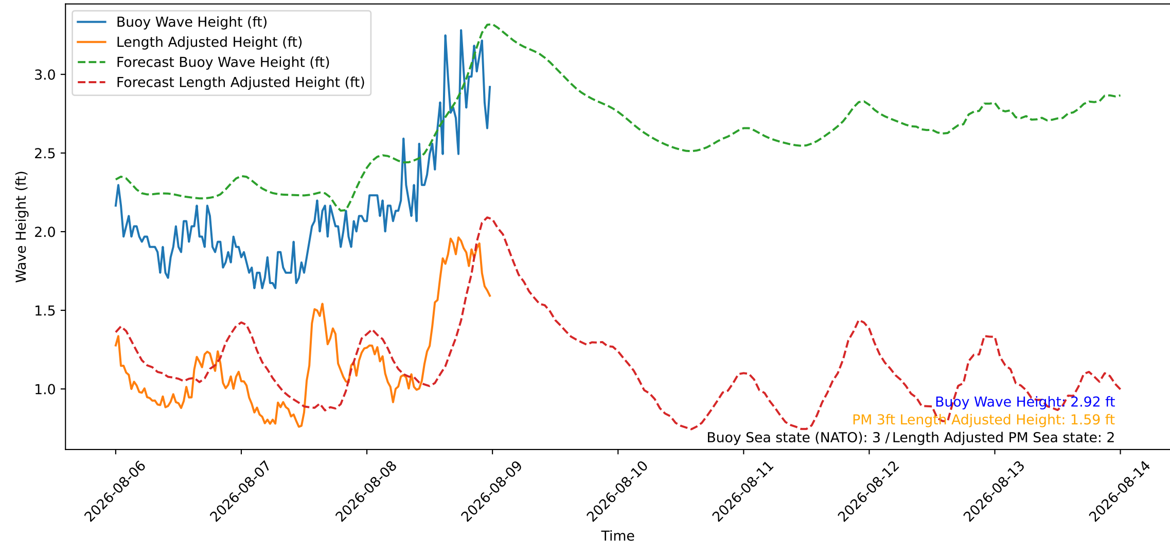
Wave Heights over Time for Oceanside Harbor at 2026-08-09 00:10:26
