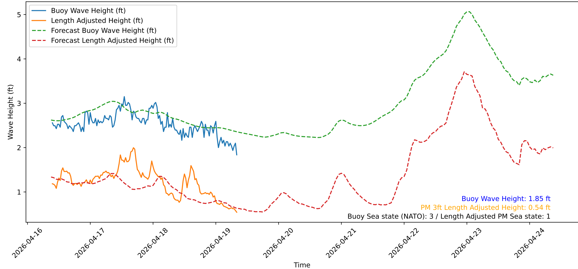
Wave Heights over Time for Red Beach at 2026-04-19 09:10:50
