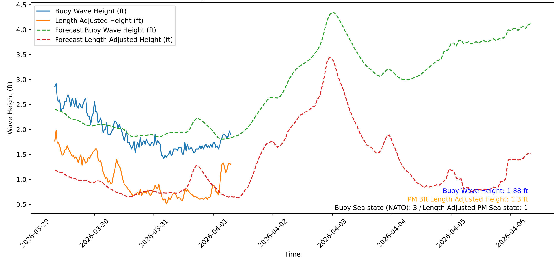
Wave Heights over Time for Green Beach at 2026-04-01 08:01:09
