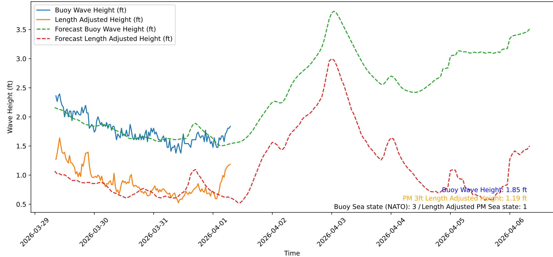
Wave Heights over Time for Red Beach at 2026-04-01 08:00:47
