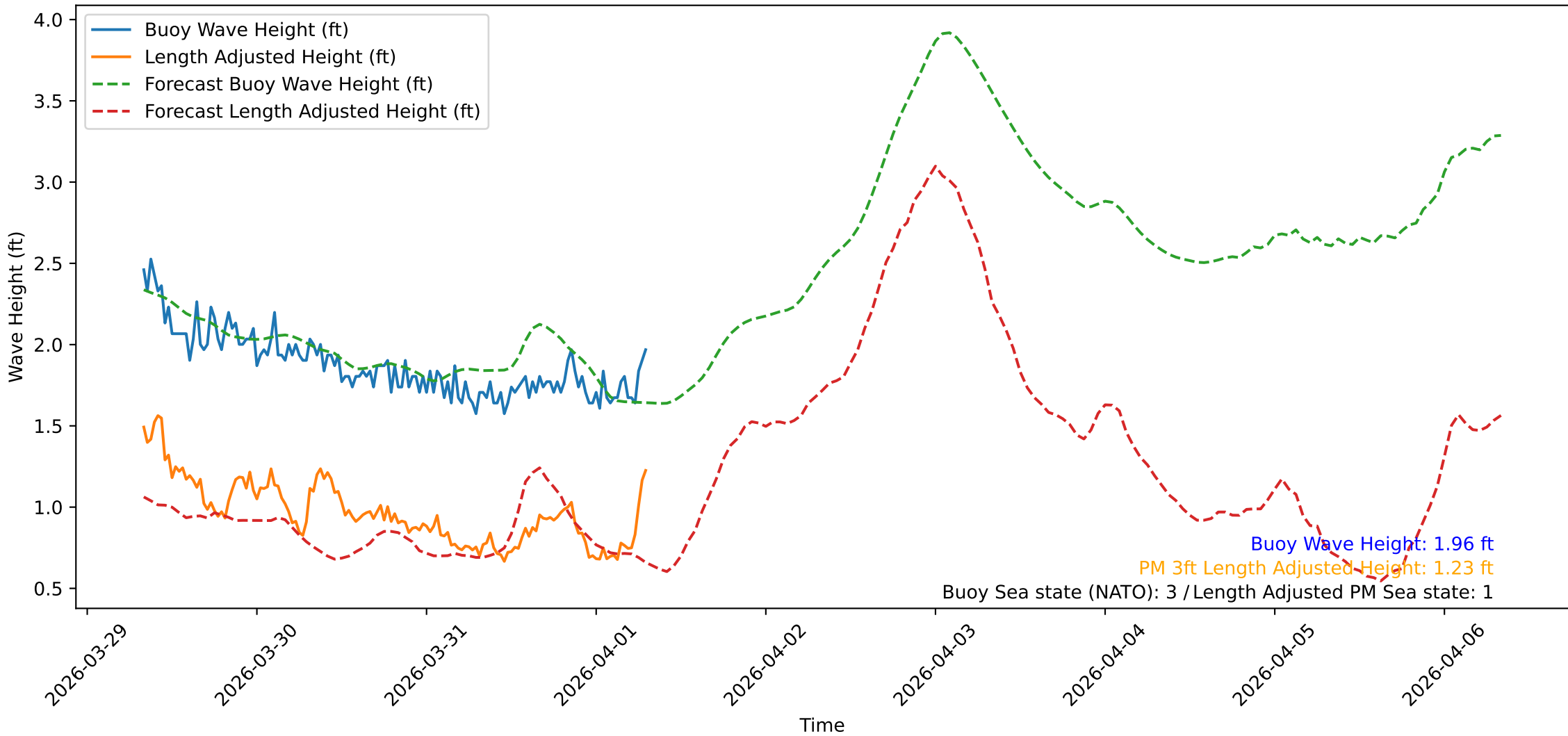
Wave Heights over Time for Oceanside Harbor at 2026-04-01 08:00:30
