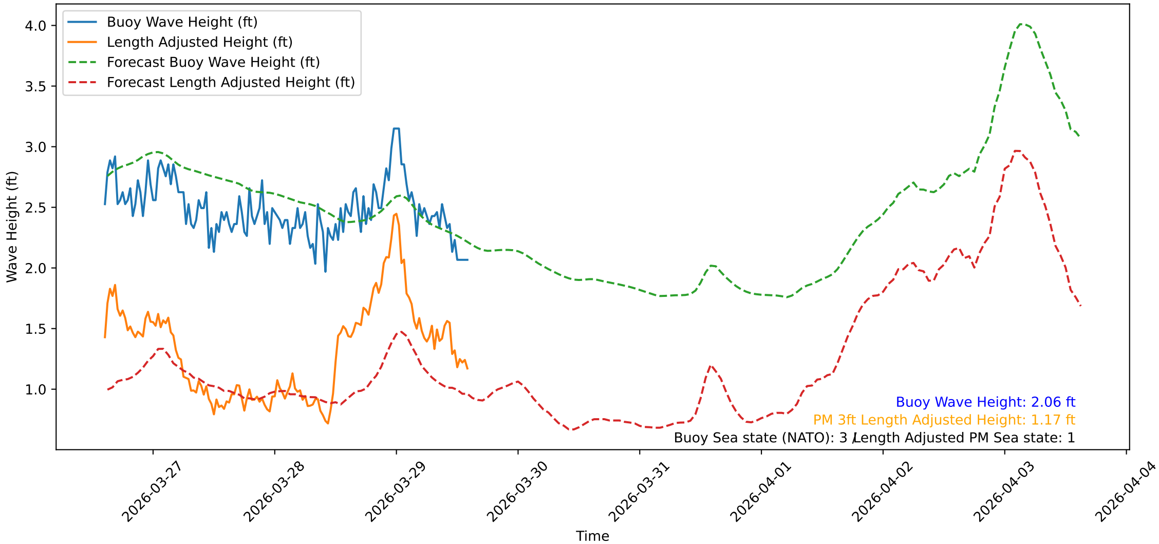
Wave Heights over Time for Oceanside Harbor at 2026-03-29 14:30:31
