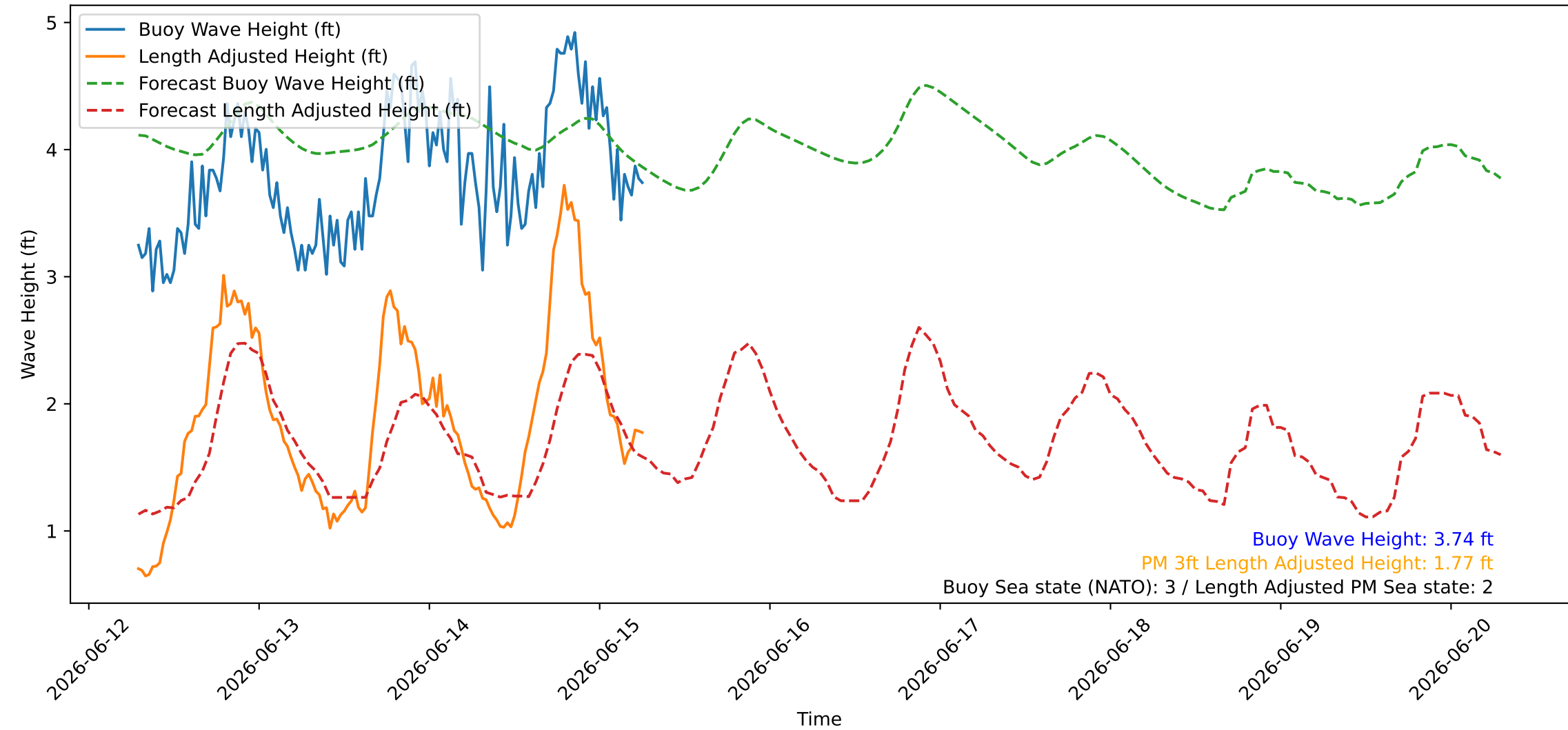
Wave Heights over Time for Green Beach at 2026-06-15 07:01:09
