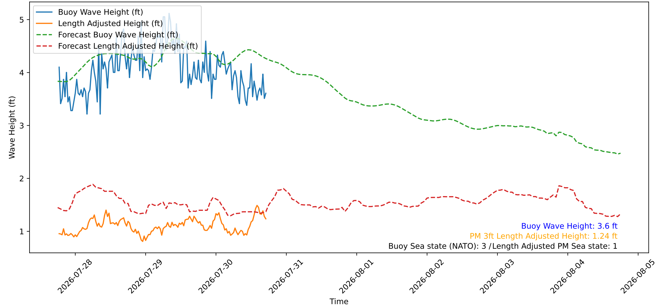
Wave Heights over Time for Red Beach at 2026-07-30 18:00:46
