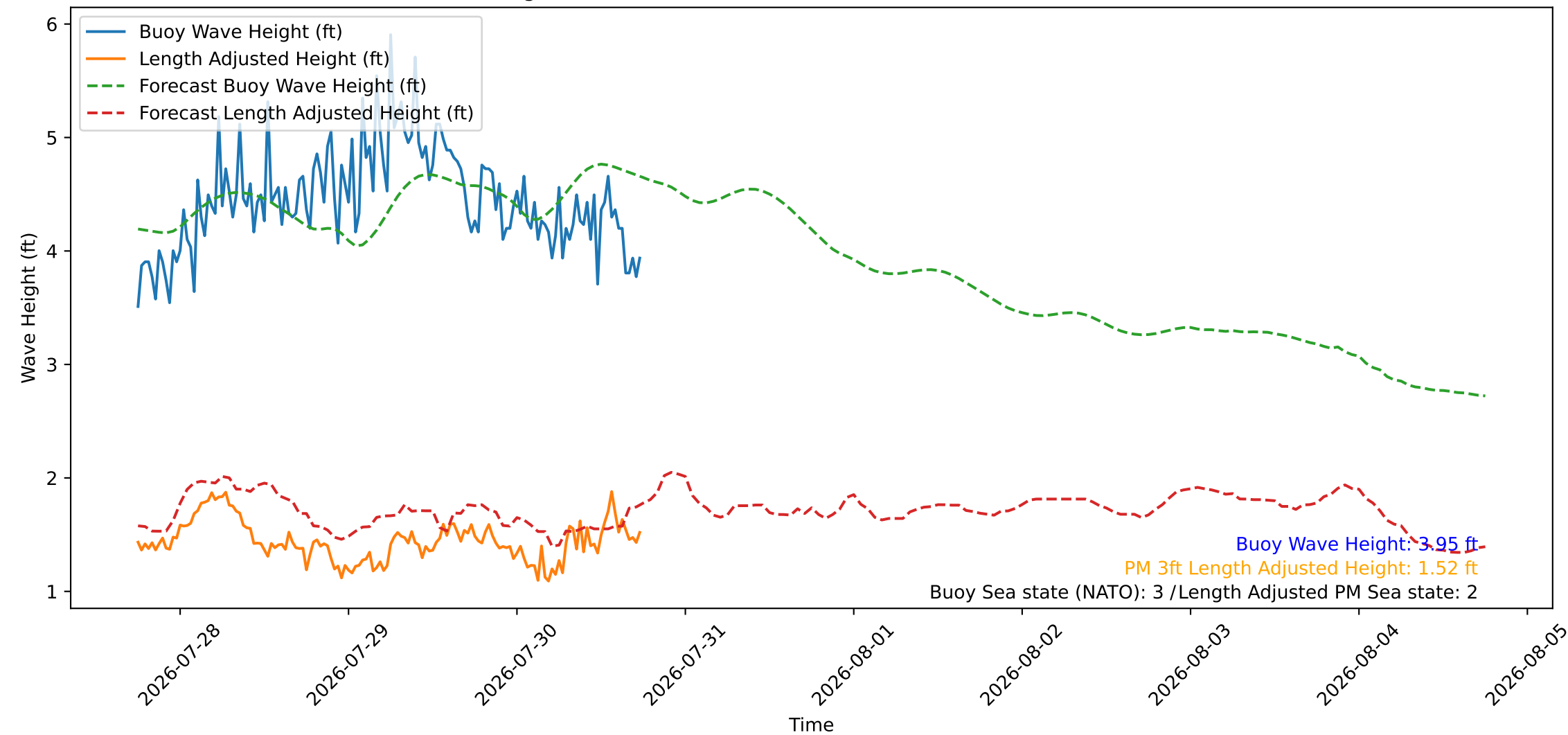
Wave Heights over Time for Oceanside Harbor at 2026-07-30 18:00:27
