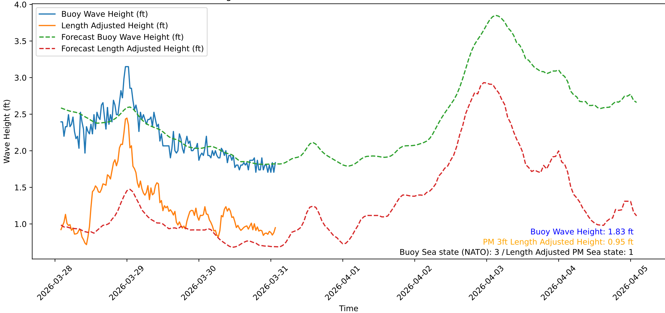
Wave Heights over Time for Oceanside Harbor at 2026-03-31 02:00:32
