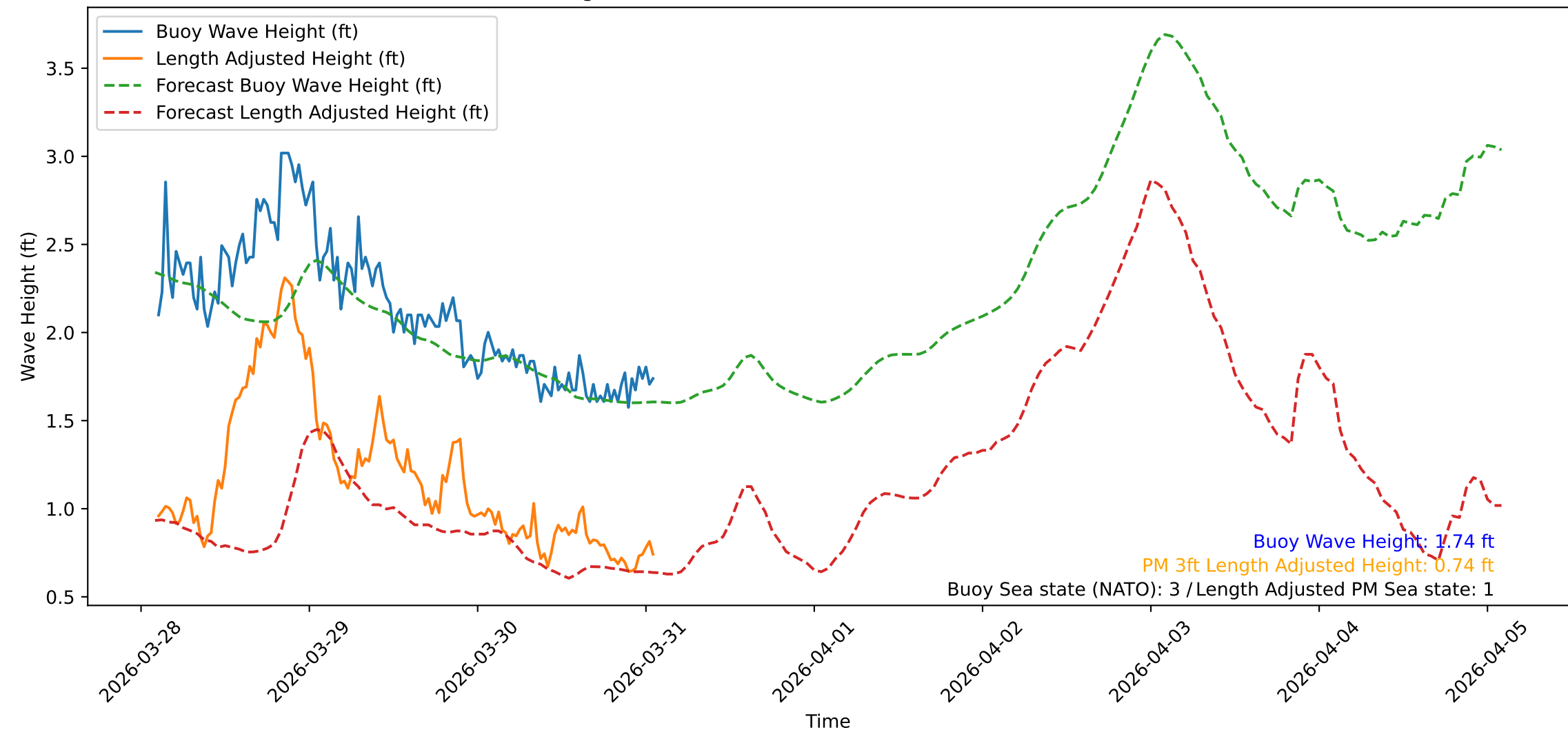
Wave Heights over Time for Red Beach at 2026-03-31 02:00:48
