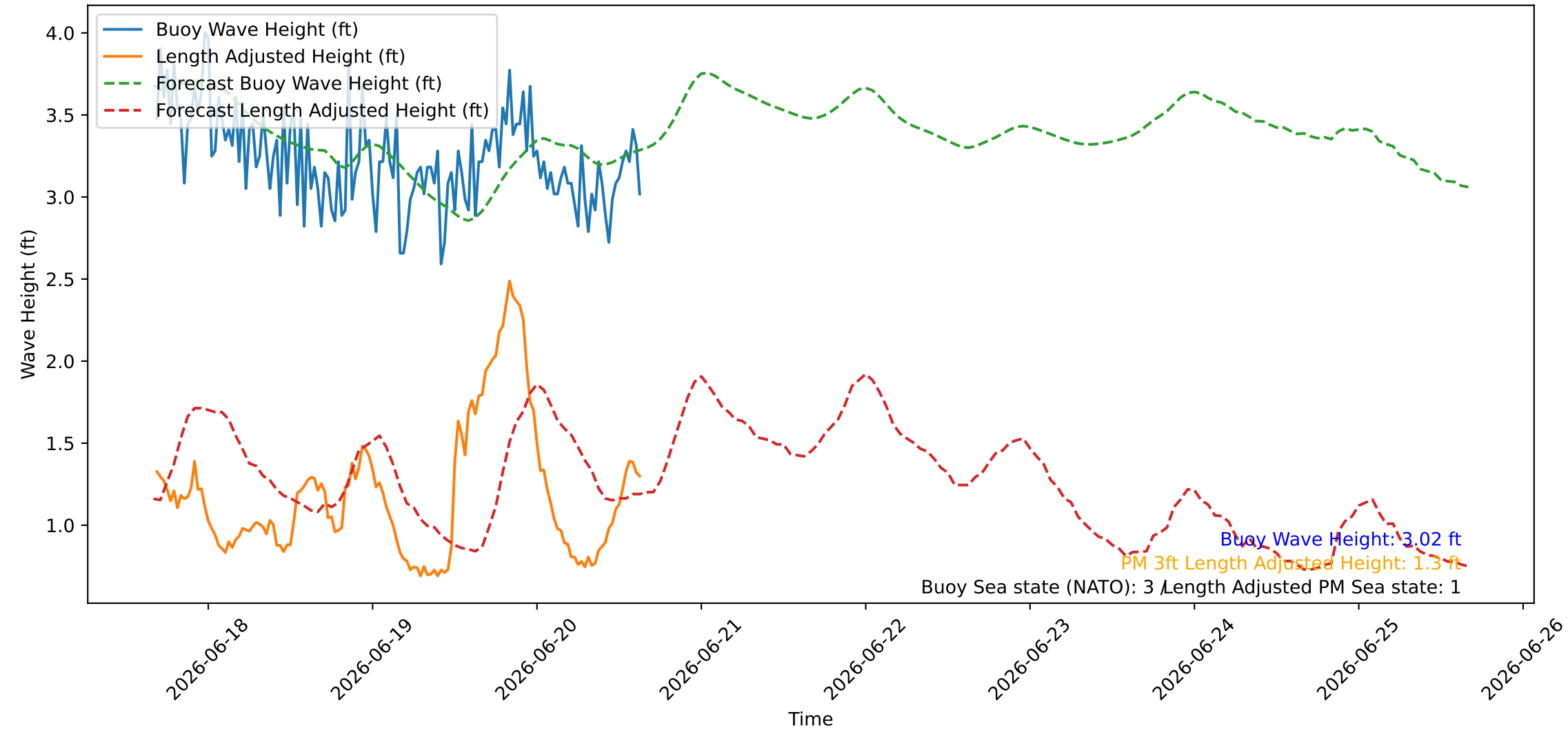
Wave Heights over Time for Red Beach at 2026-06-20 16:00:46
