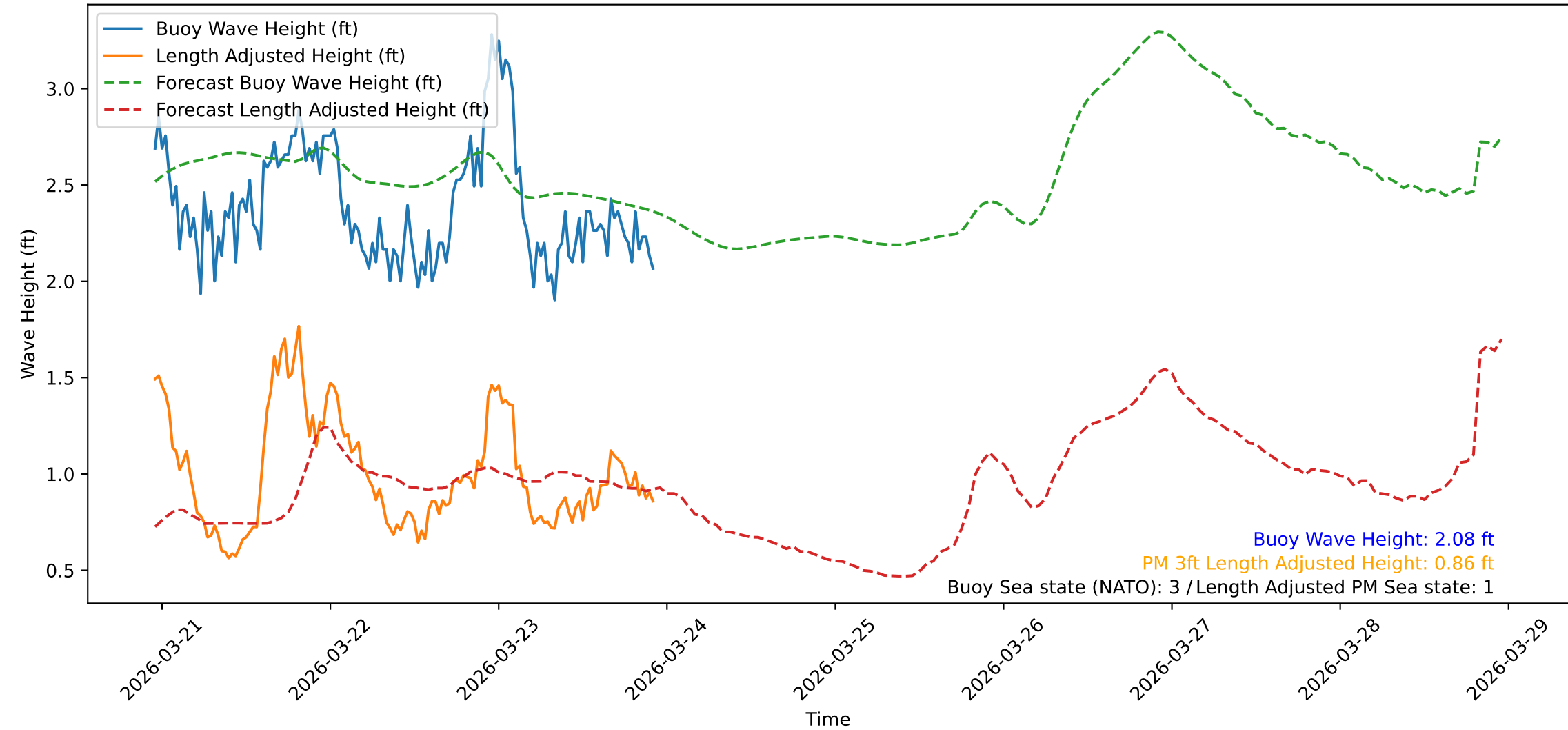
Wave Heights over Time for Green Beach at 2026-03-23 23:11:09
