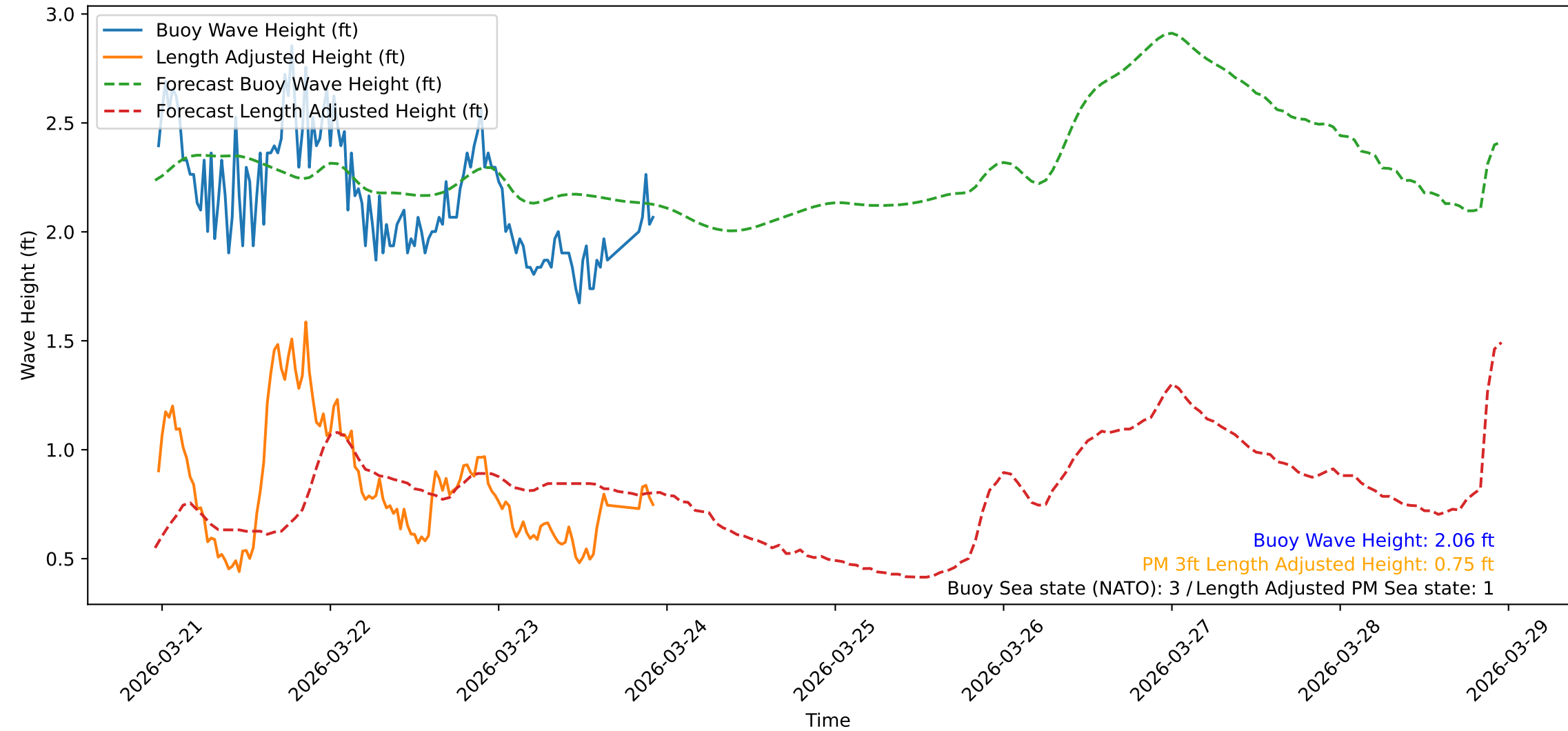
Wave Heights over Time for Red Beach at 2026-03-23 23:10:47
