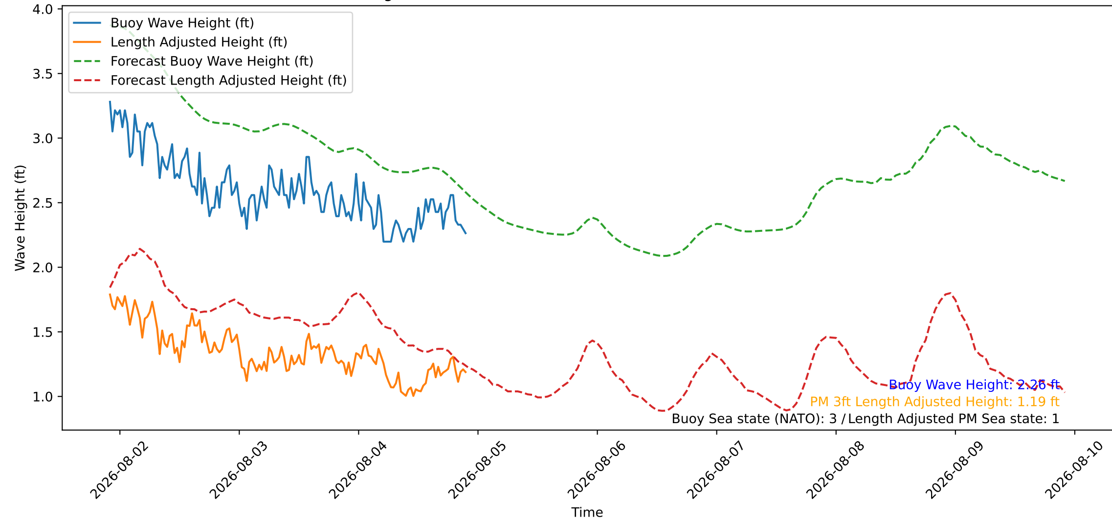
Wave Heights over Time for Oceanside Harbor at 2026-08-04 22:00:26
