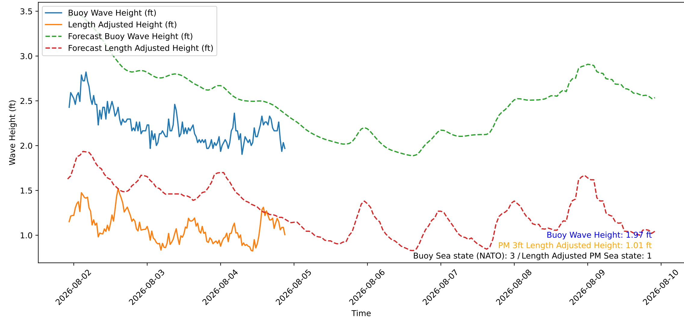
Wave Heights over Time for Red Beach at 2026-08-04 22:00:46
