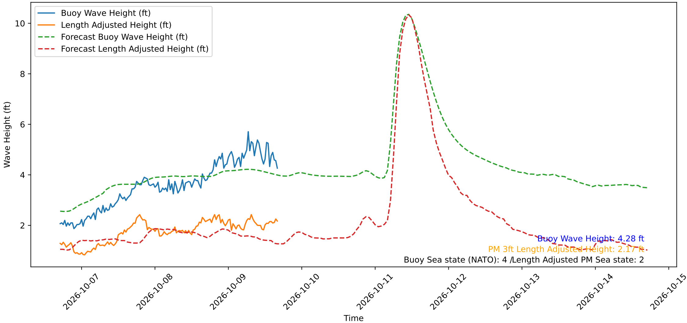
Wave Heights over Time for Red Beach at 2026-10-09 16:50:50
