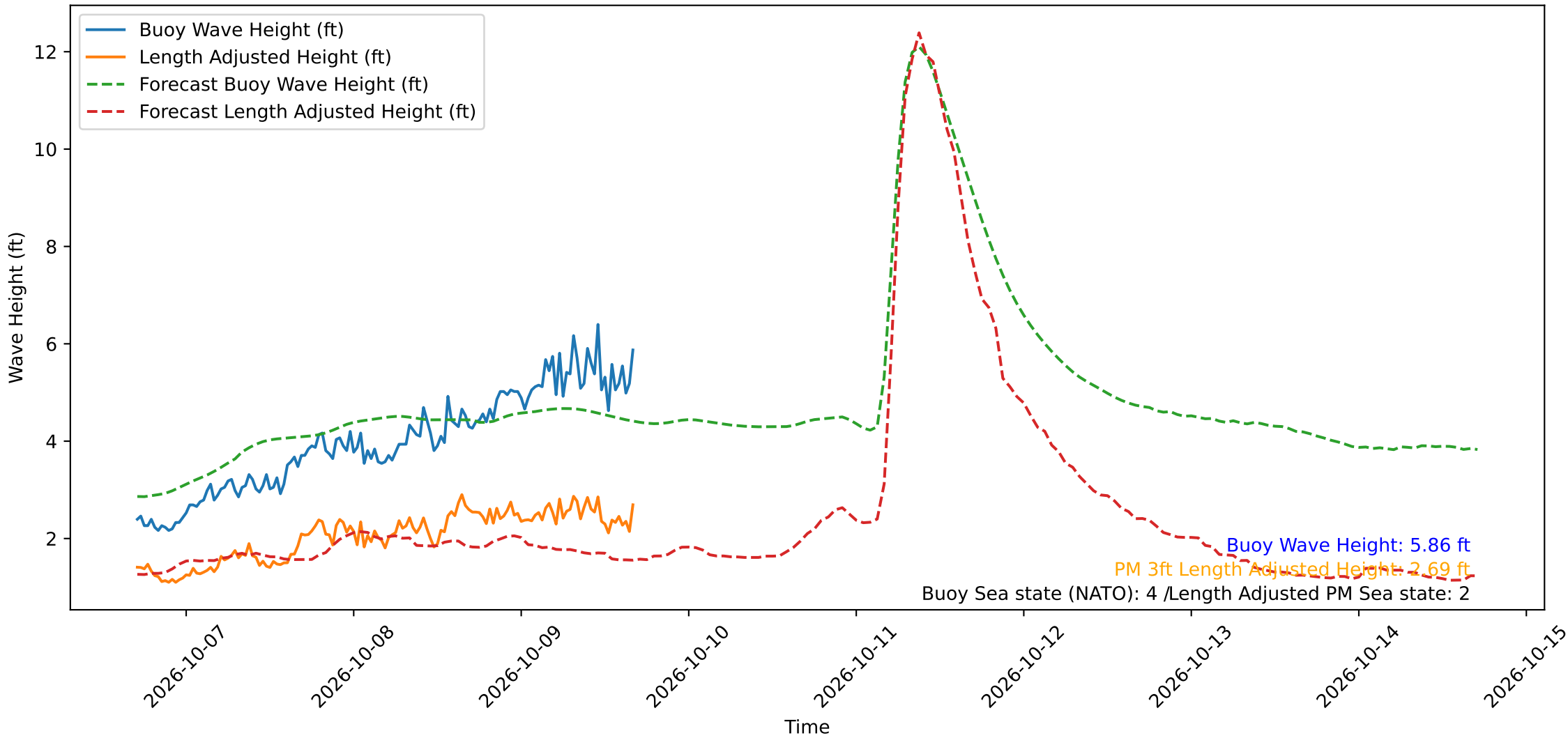
Wave Heights over Time for Oceanside Harbor at 2026-10-09 16:50:29
