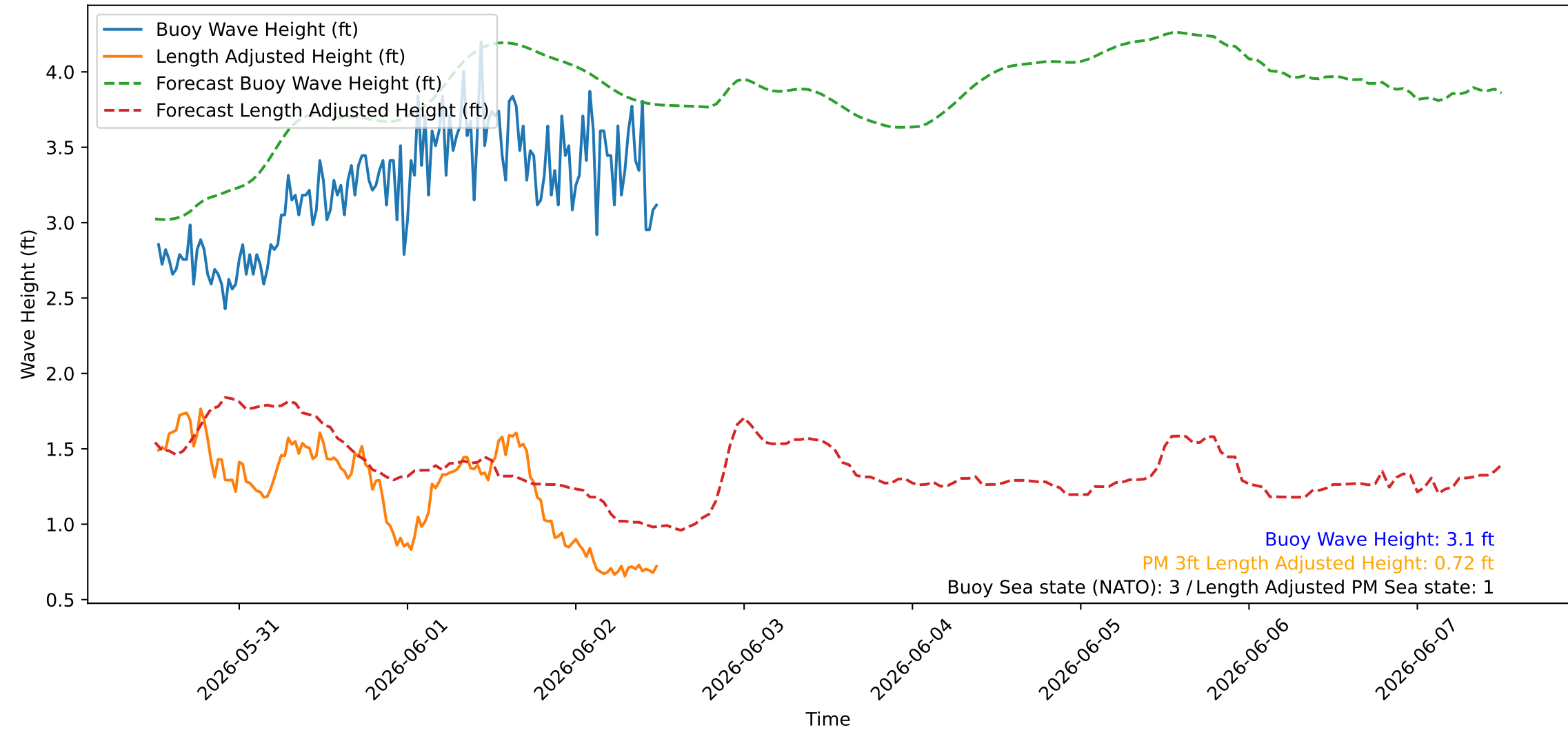
Wave Heights over Time for Red Beach at 2026-06-02 12:20:46
