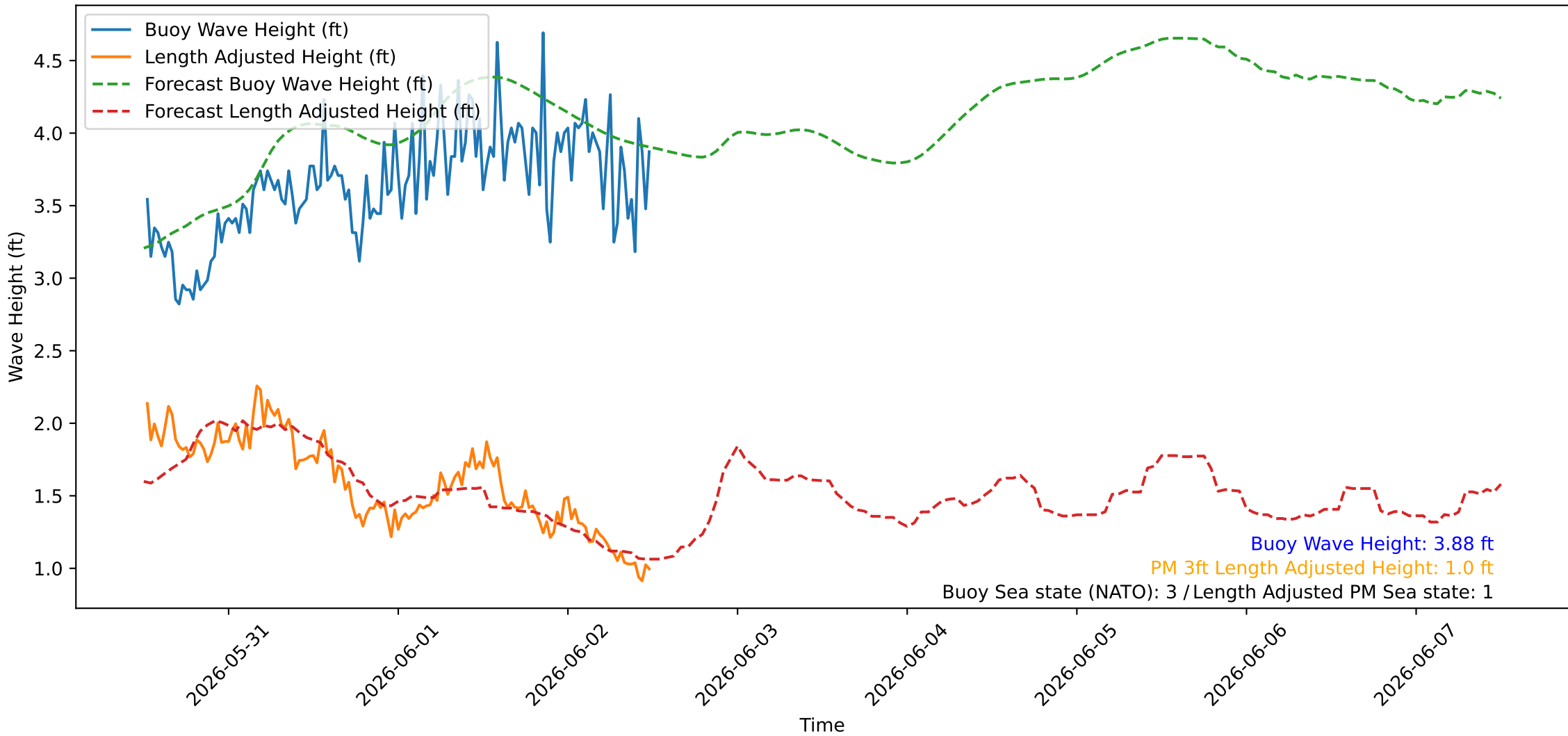
Wave Heights over Time for Oceanside Harbor at 2026-06-02 12:20:25
