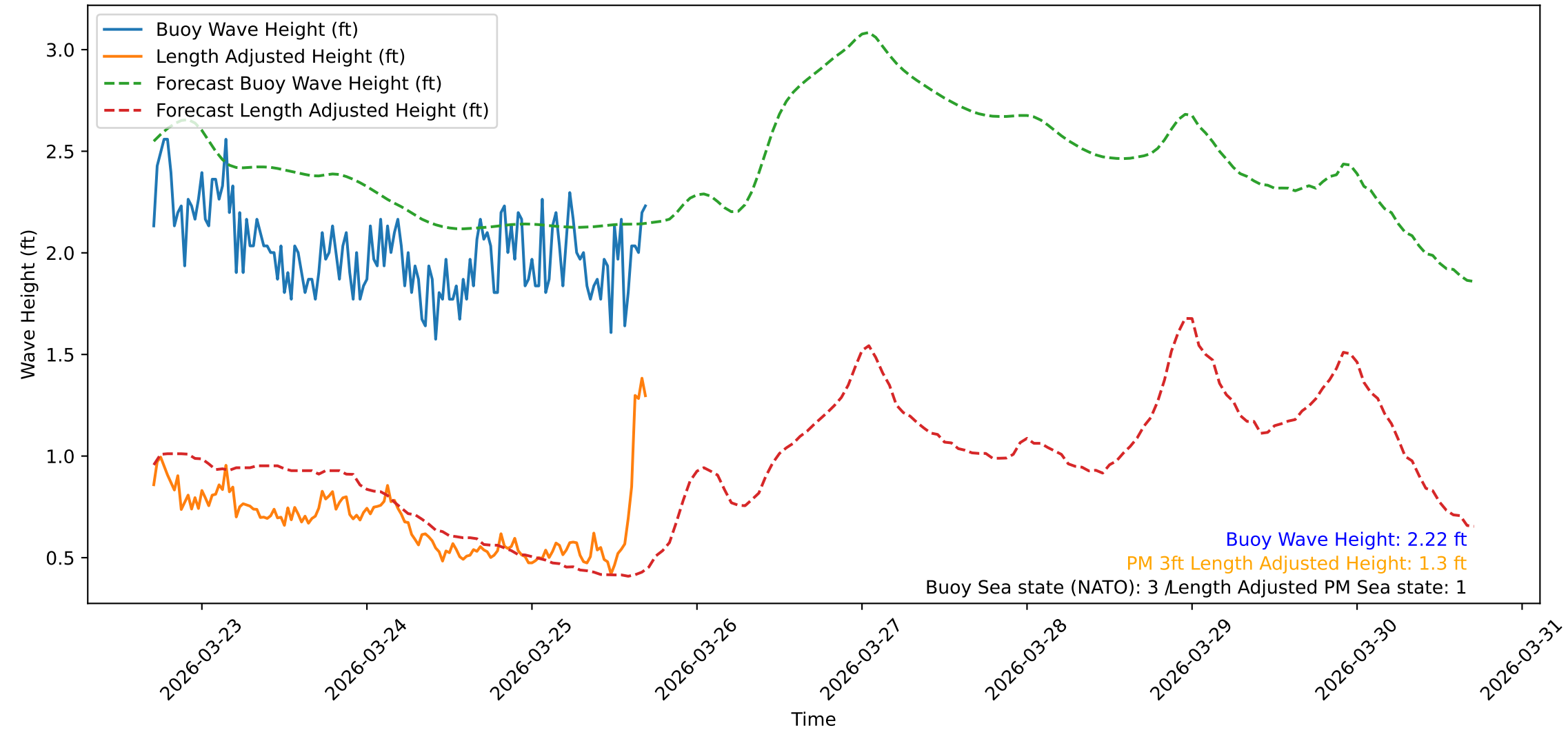
Wave Heights over Time for Oceanside Harbor at 2026-03-25 17:00:32
