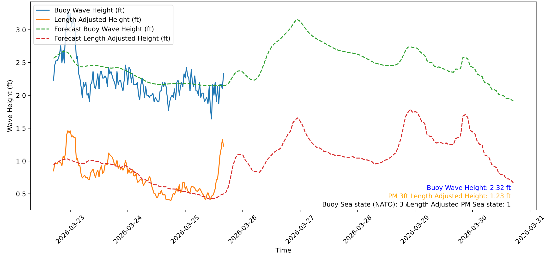
Wave Heights over Time for Green Beach at 2026-03-25 17:01:11
