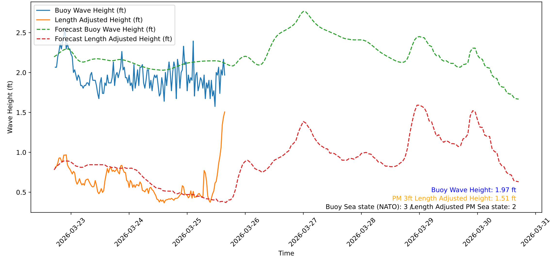
Wave Heights over Time for Red Beach at 2026-03-25 17:00:49
