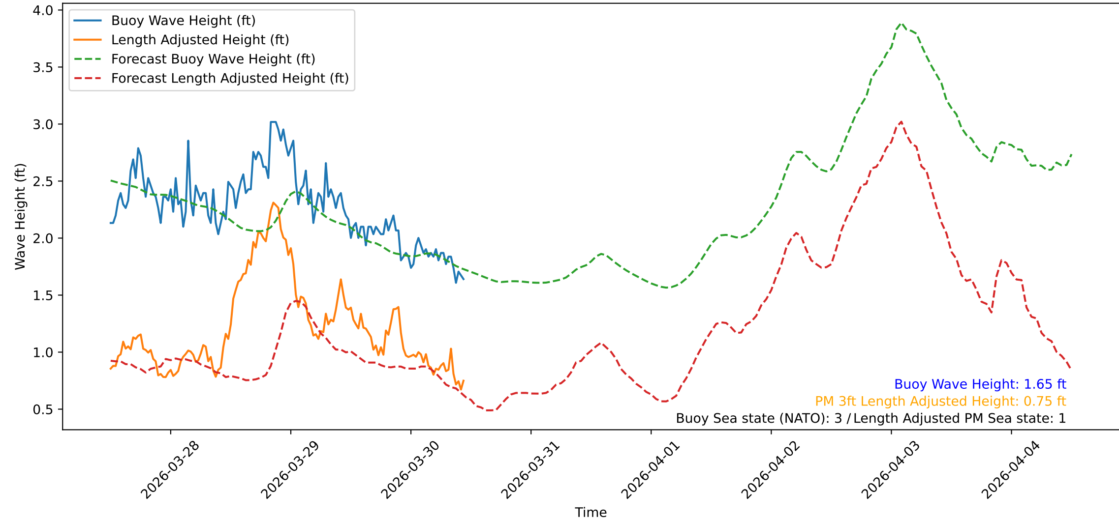
Wave Heights over Time for Red Beach at 2026-03-30 11:30:47
