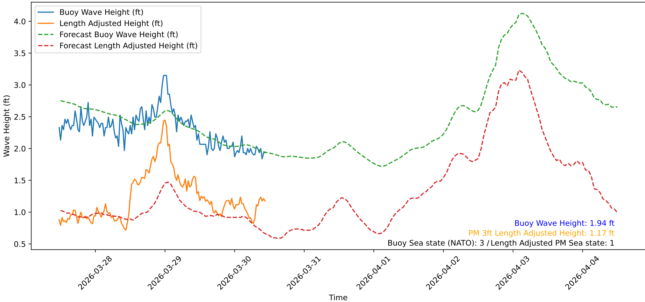
Wave Heights over Time for Oceanside Harbor at 2026-03-30 11:30:31
