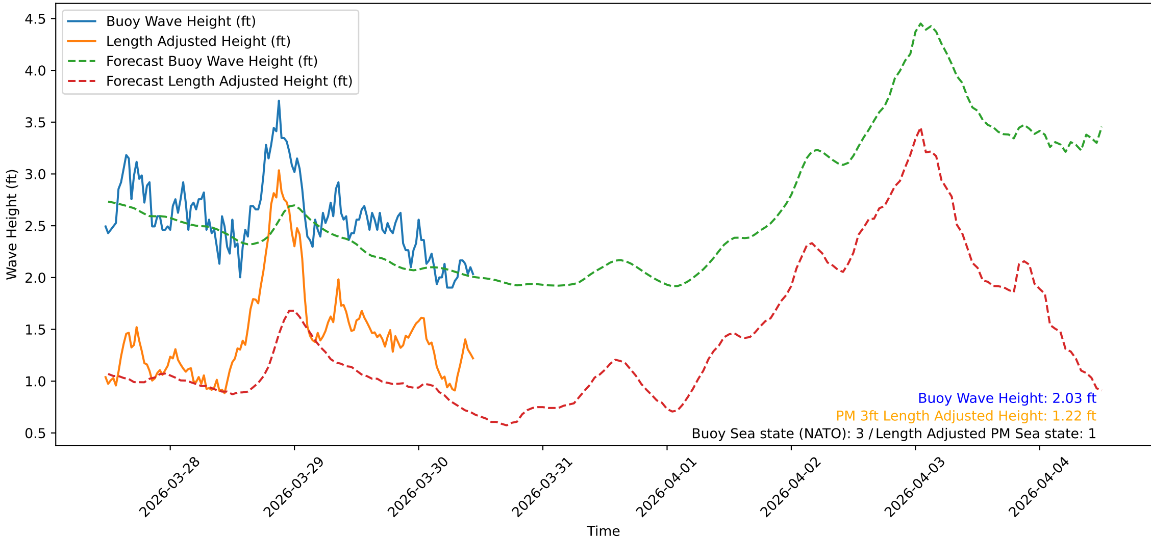
Wave Heights over Time for Green Beach at 2026-03-30 11:31:10
