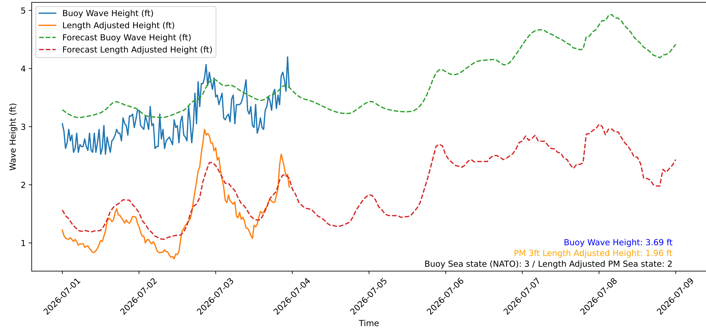
Wave Heights over Time for Green Beach at 2026-07-03 23:51:09
