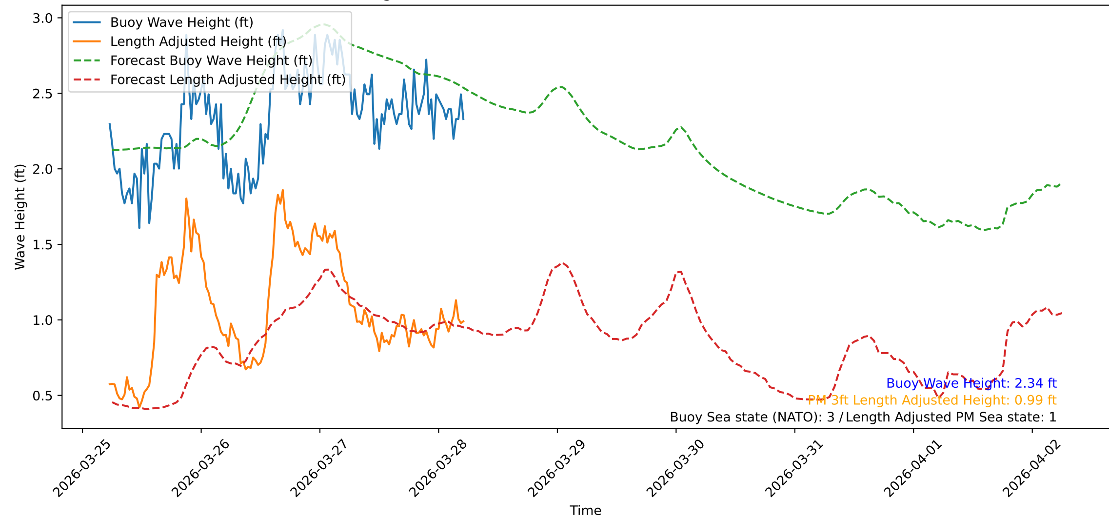
Wave Heights over Time for Oceanside Harbor at 2026-03-28 05:30:30
