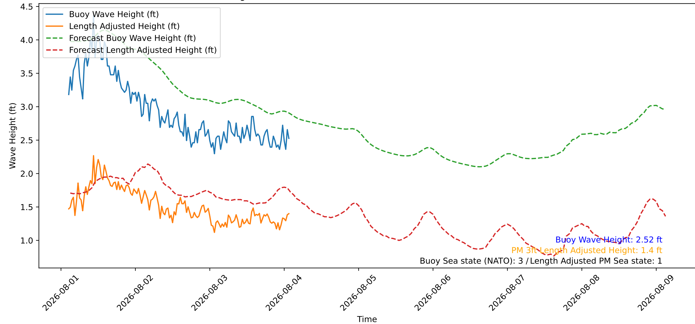
Wave Heights over Time for Oceanside Harbor at 2026-08-04 02:30:27
