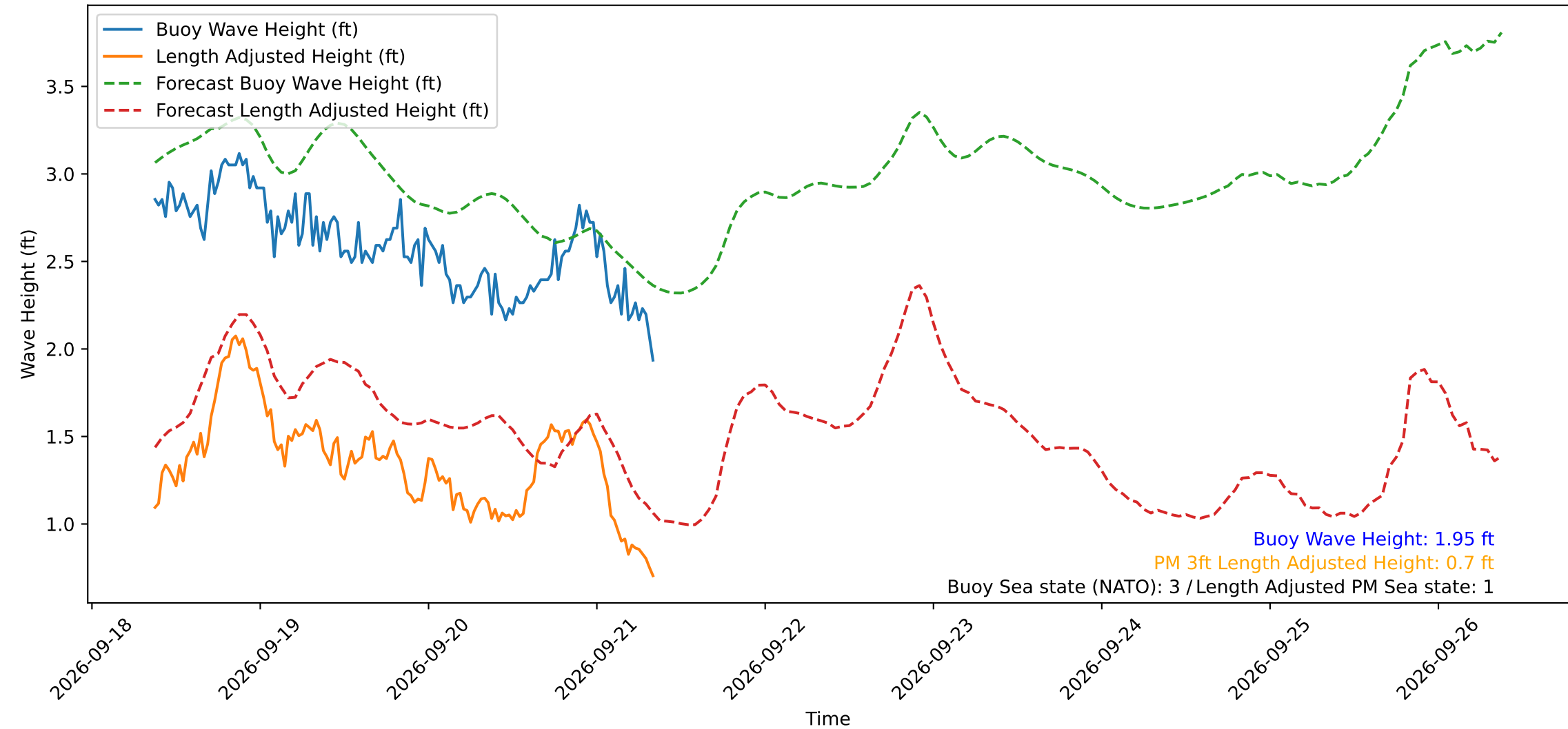
Wave Heights over Time for Green Beach at 2026-09-21 08:51:15
