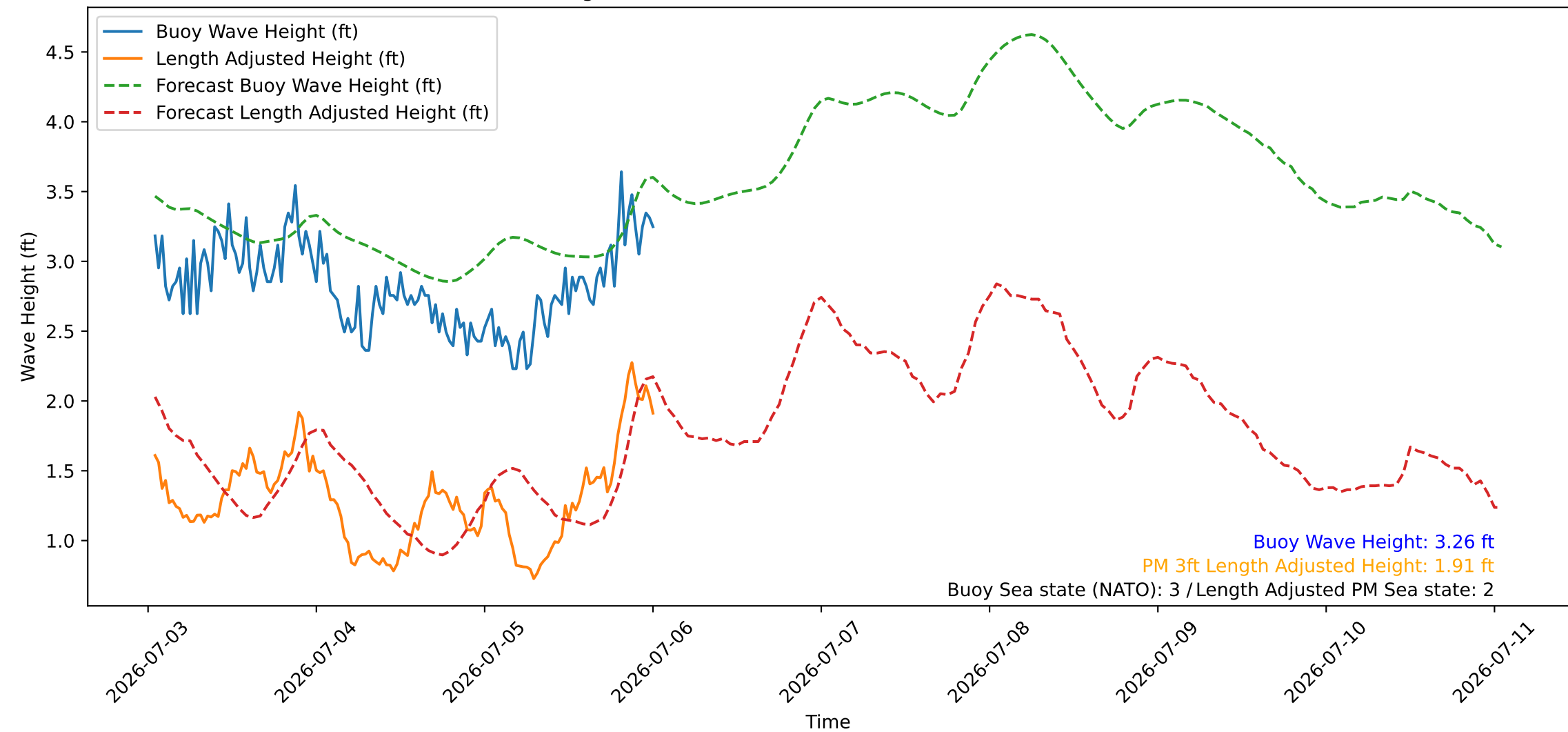
Wave Heights over Time for Red Beach at 2026-07-06 00:50:47
