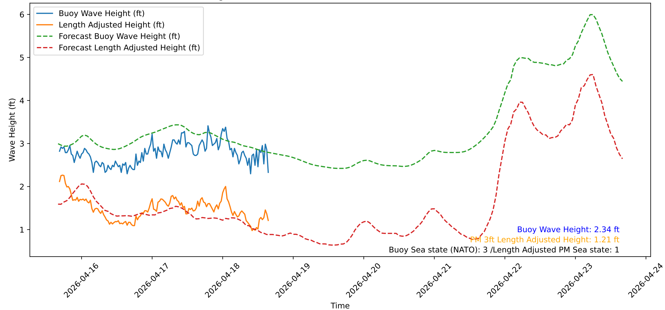
Wave Heights over Time for Oceanside Harbor at 2026-04-18 16:20:30
