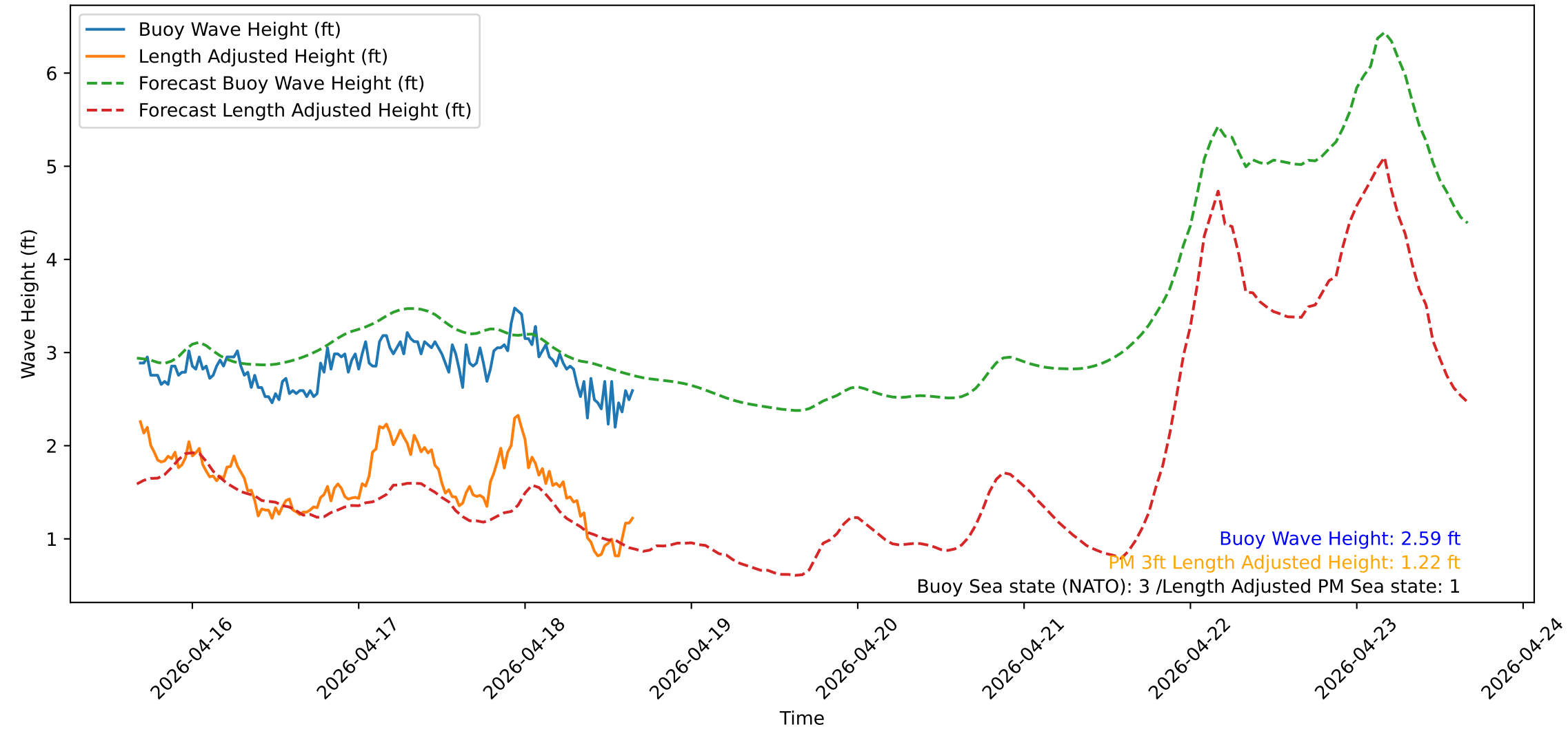
Wave Heights over Time for Green Beach at 2026-04-18 16:21:12
