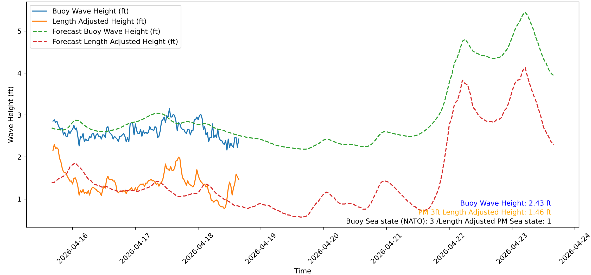
Wave Heights over Time for Red Beach at 2026-04-18 16:20:50
