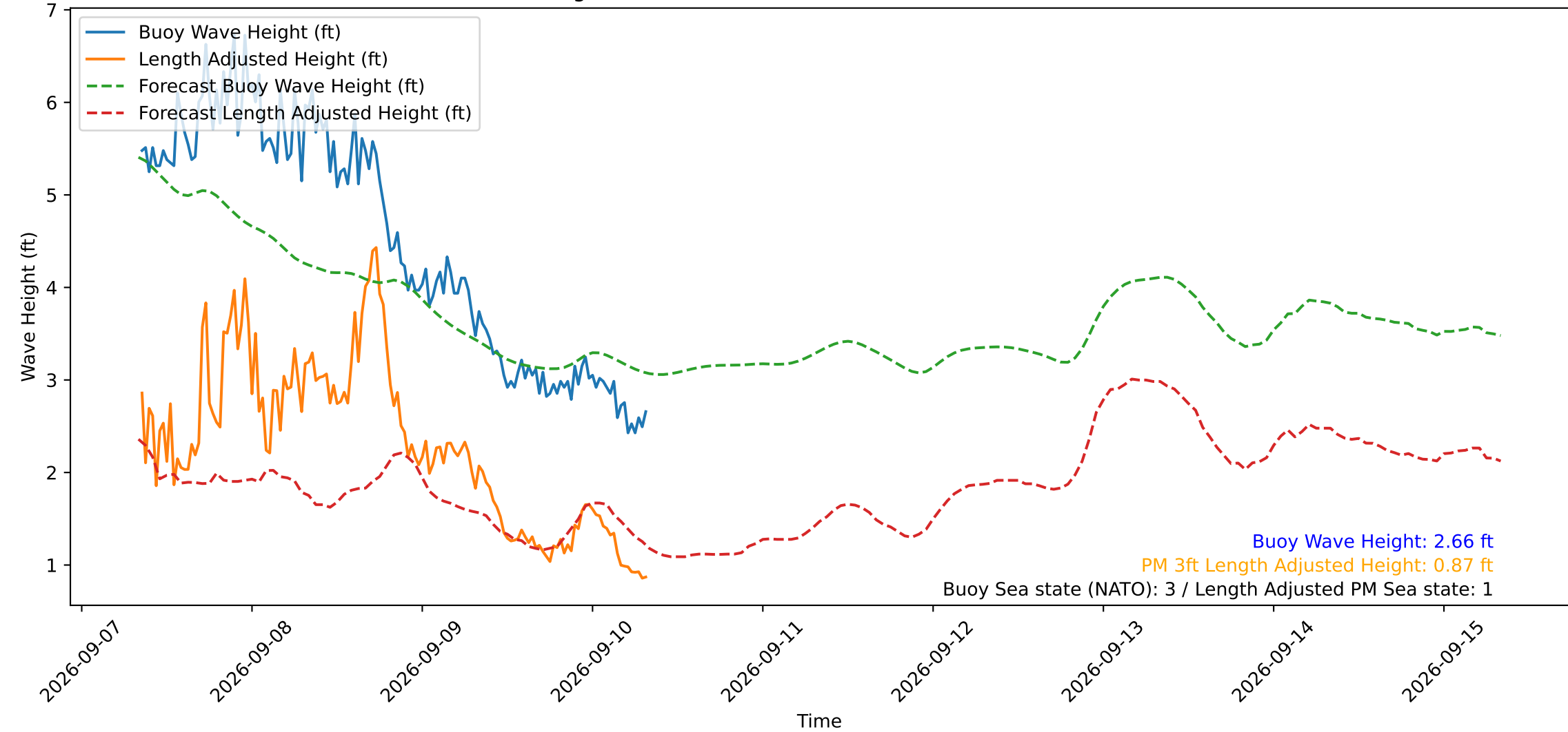
Wave Heights over Time for Red Beach at 2026-09-10 08:20:50
