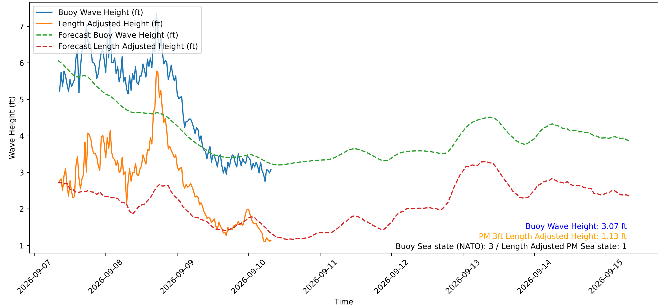
Wave Heights over Time for Oceanside Harbor at 2026-09-10 08:20:29
