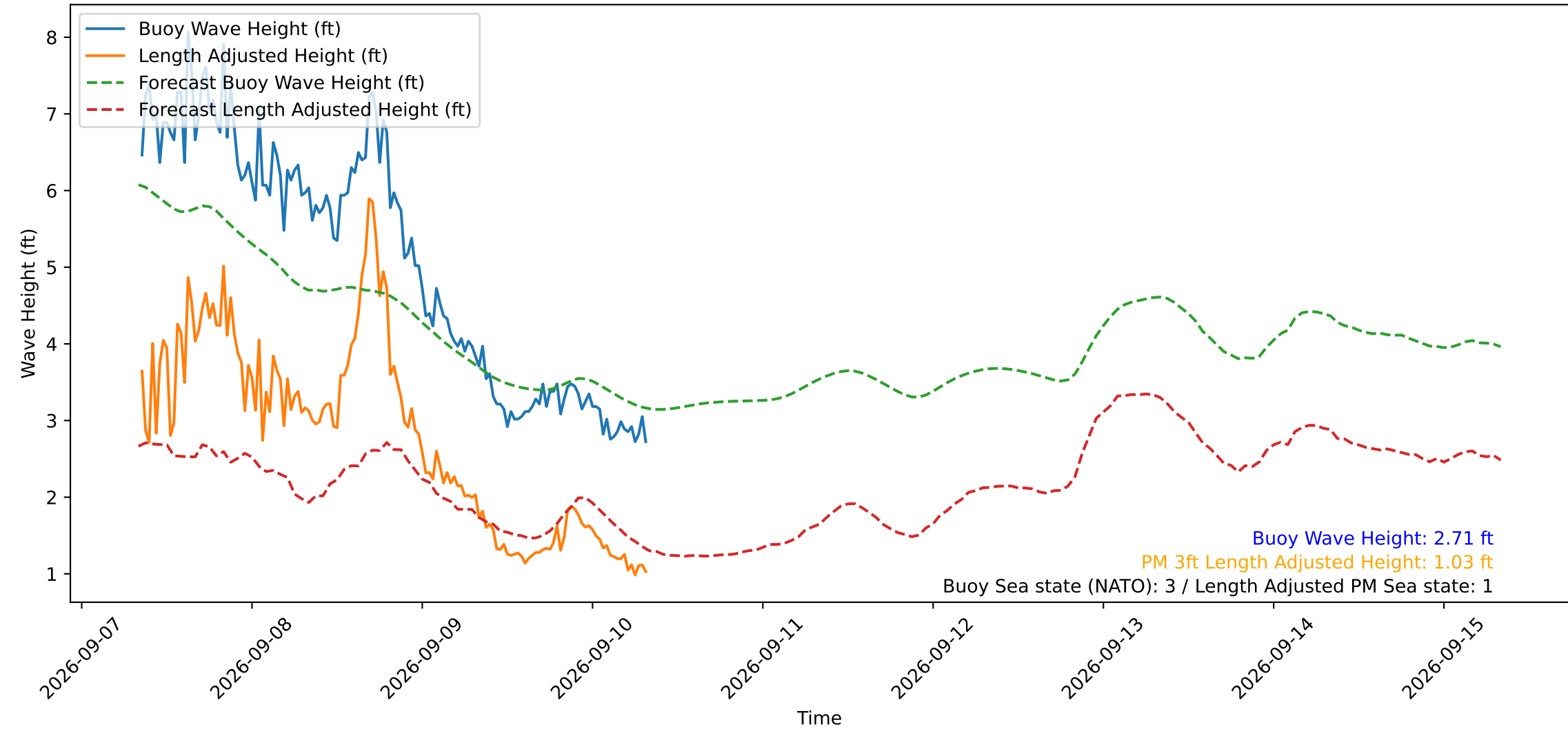
Wave Heights over Time for Green Beach at 2026-09-10 08:21:14
