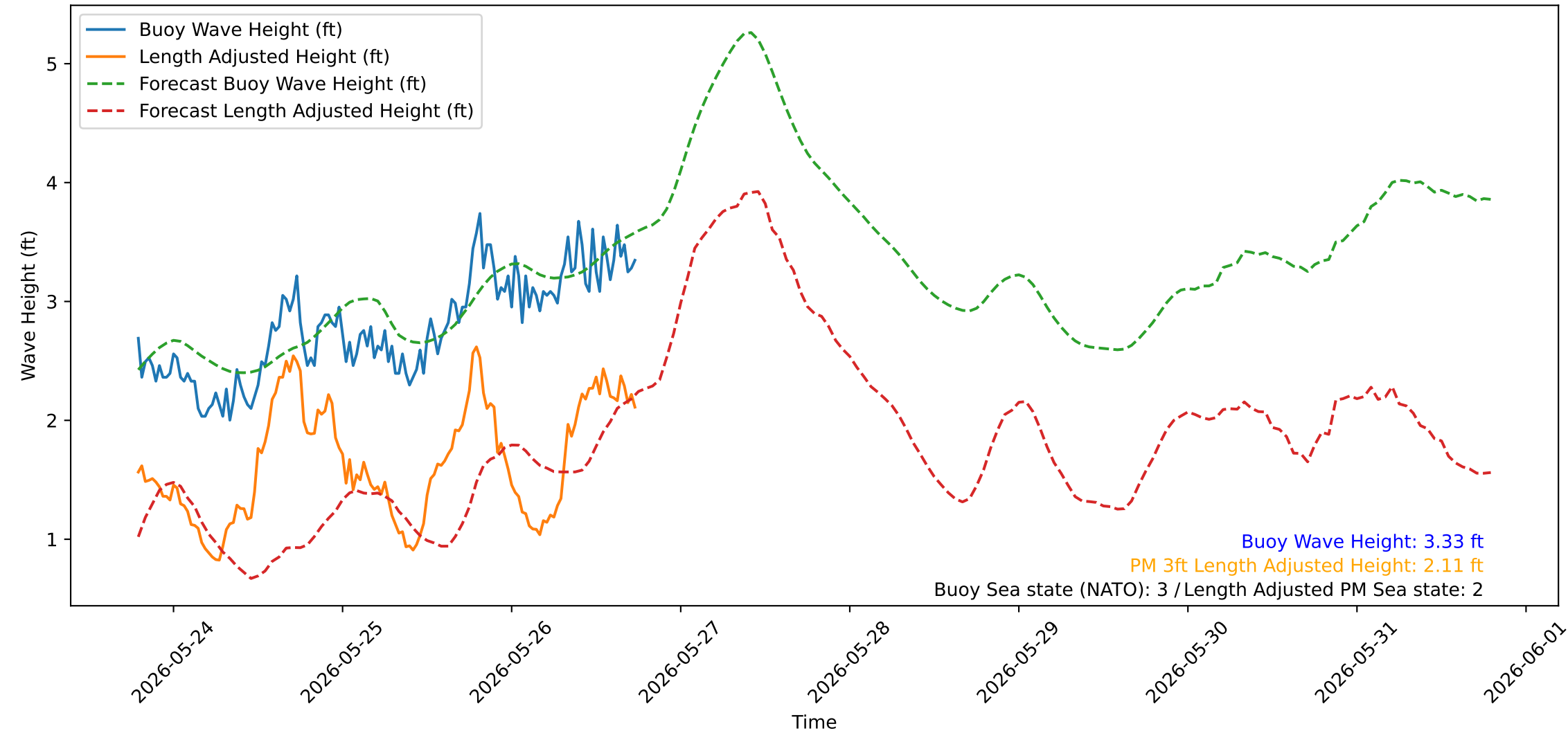
Wave Heights over Time for Red Beach at 2026-05-26 18:30:47
