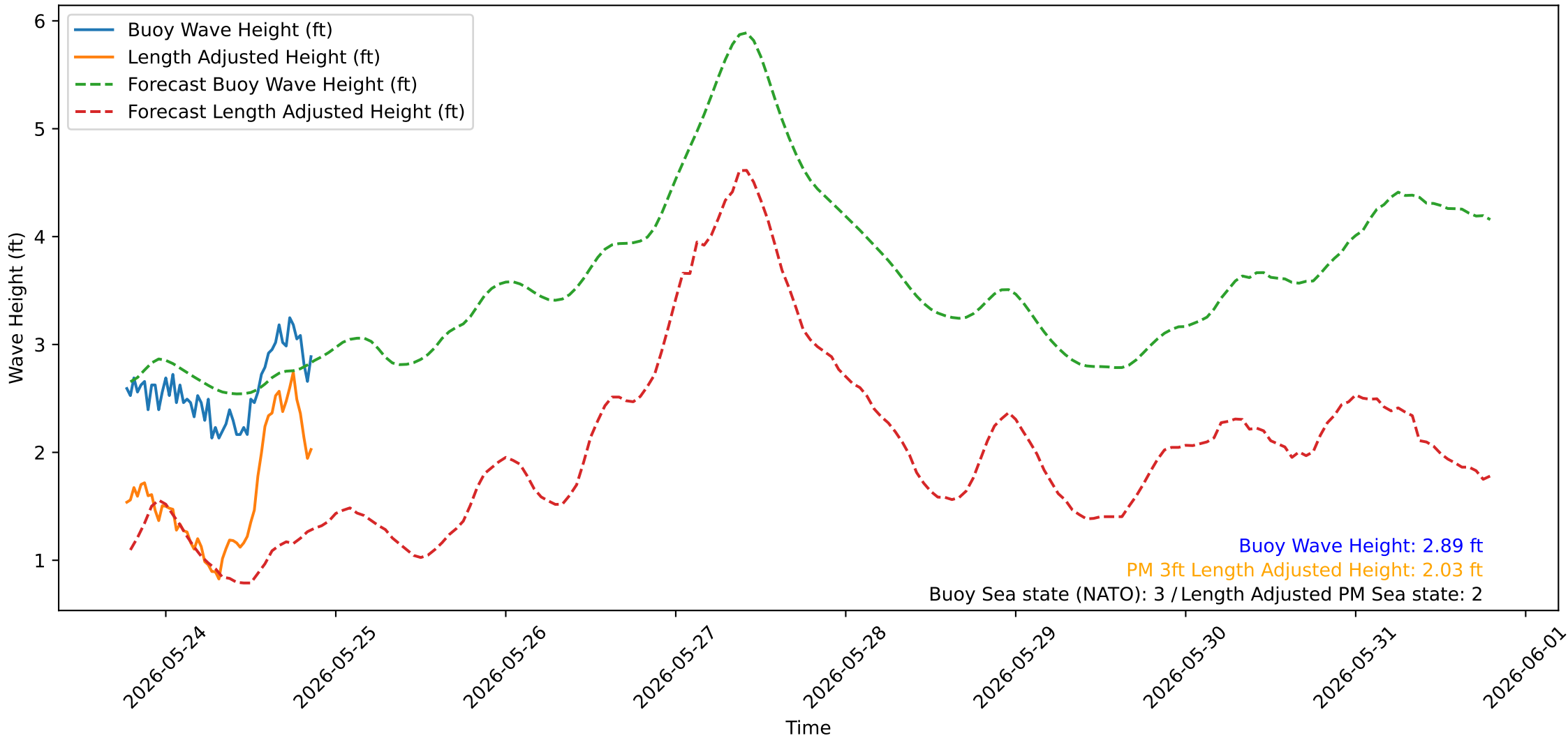
Wave Heights over Time for Oceanside Harbor at 2026-05-26 18:30:28
