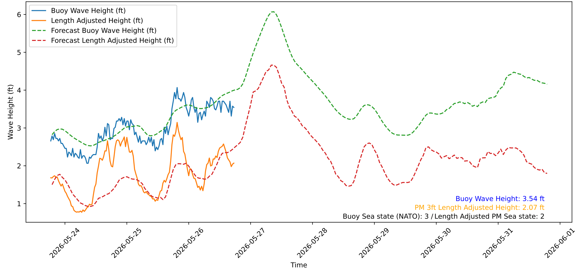
Wave Heights over Time for Green Beach at 2026-05-26 18:31:10
