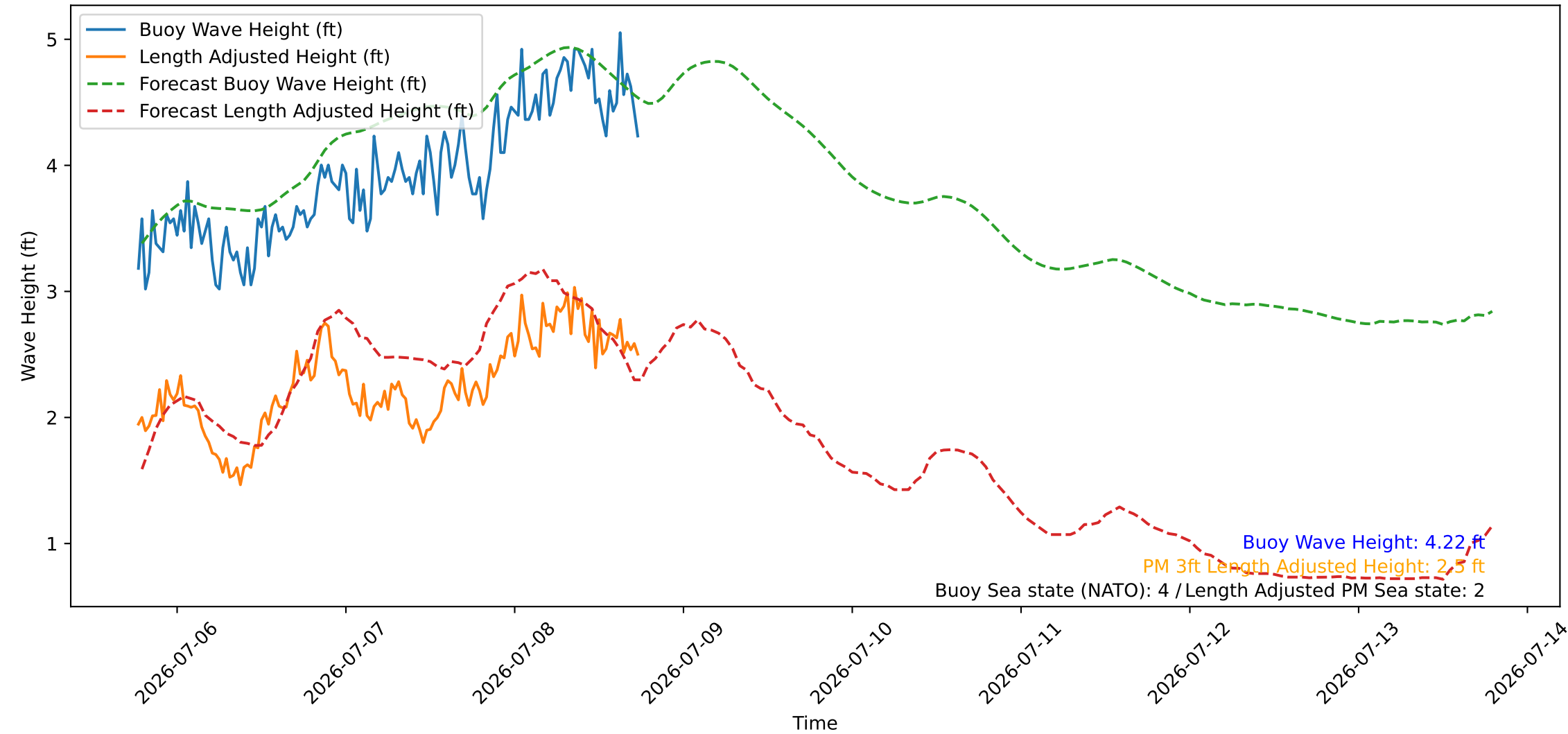
Wave Heights over Time for Oceanside Harbor at 2026-07-08 18:30:26
