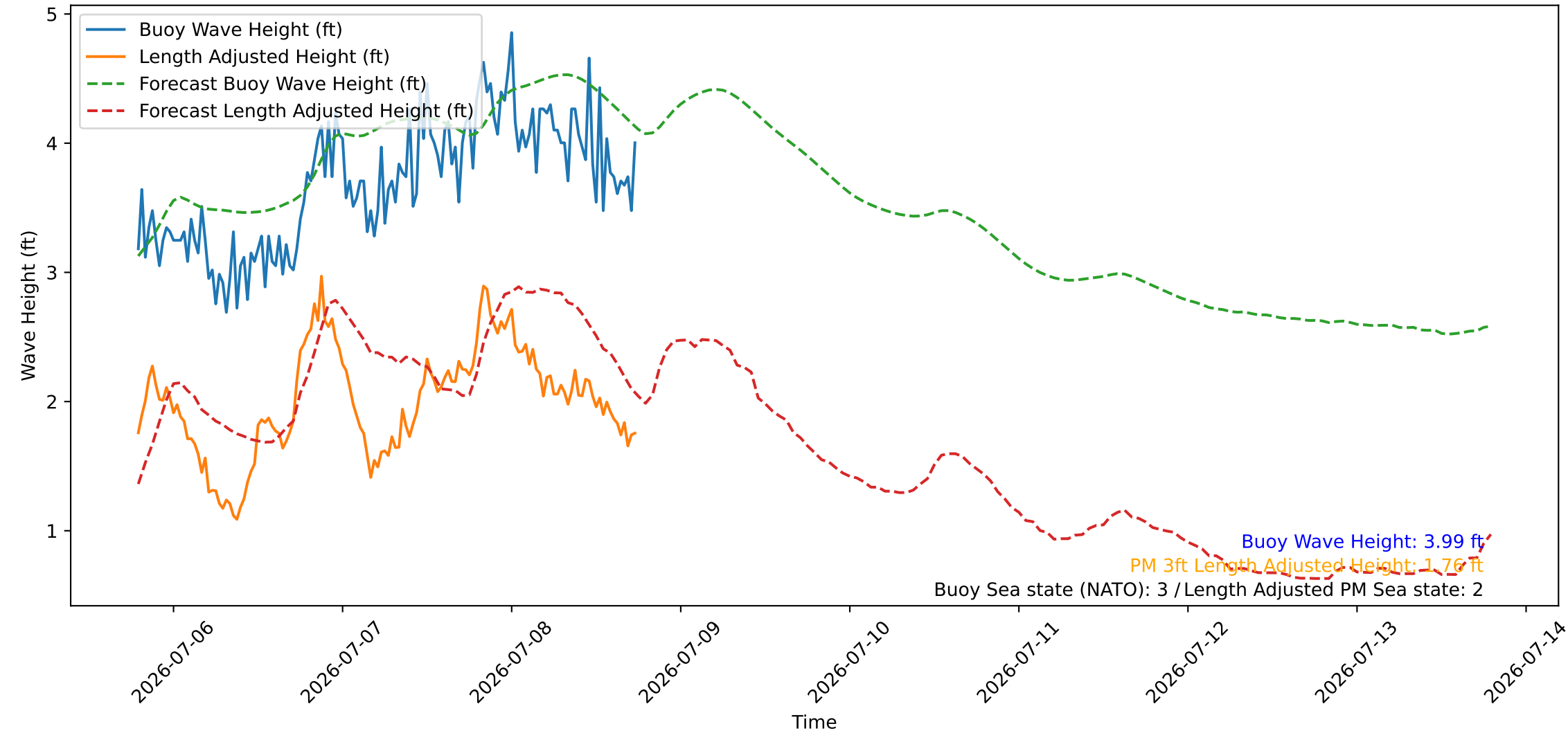
Wave Heights over Time for Red Beach at 2026-07-08 18:30:45
