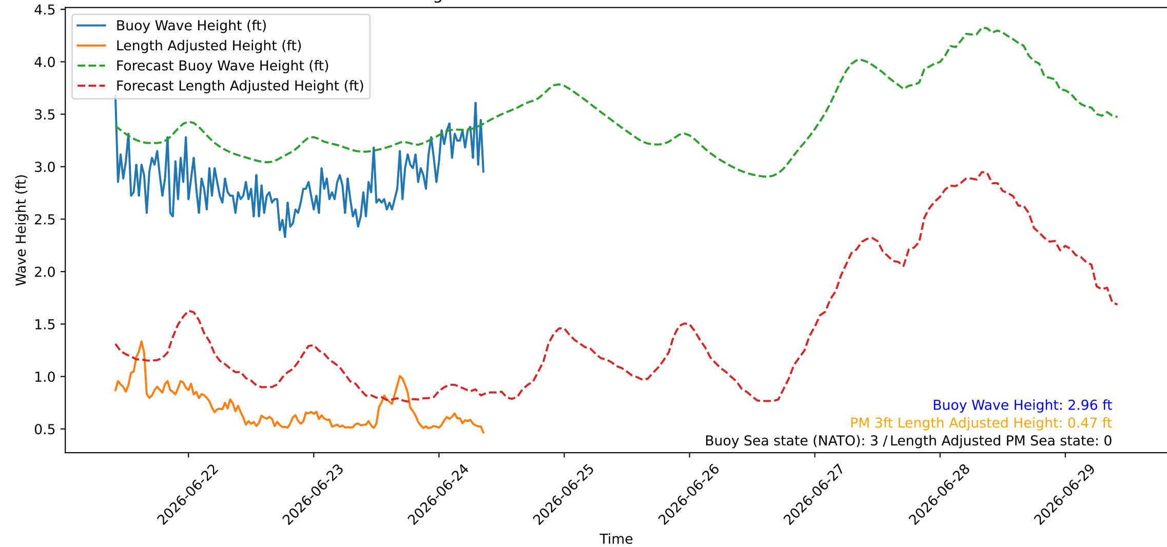
Wave Heights over Time for Red Beach at 2026-06-24 09:50:46
