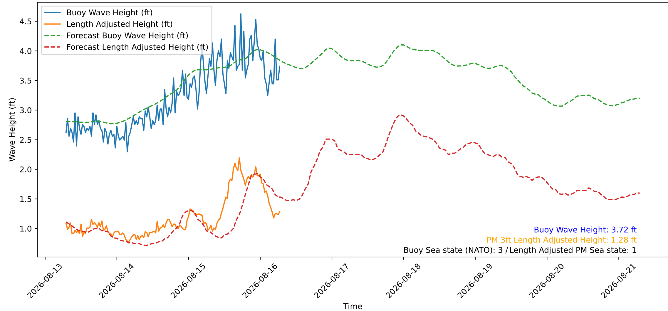
Wave Heights over Time for Oceanside Harbor at 2026-08-16 07:10:26
