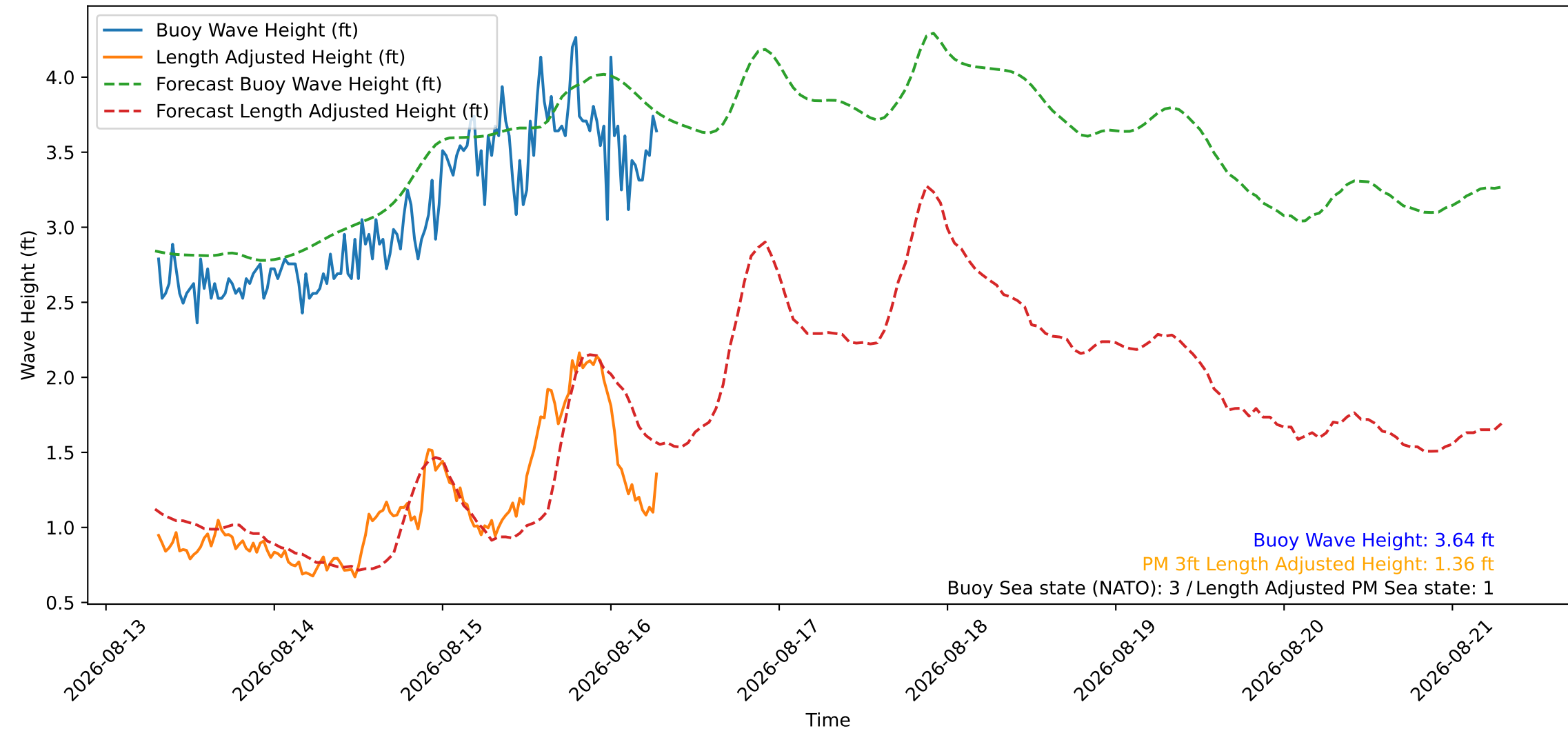
Wave Heights over Time for Green Beach at 2026-08-16 07:11:08
