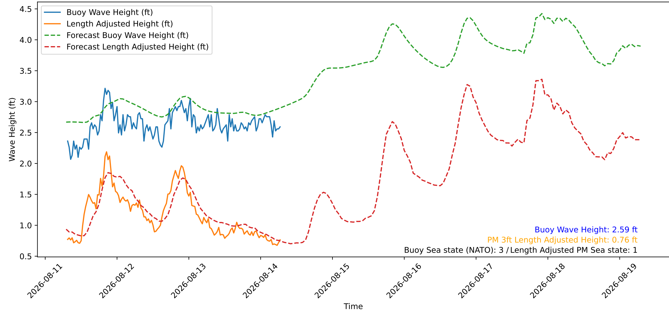
Wave Heights over Time for Green Beach at 2026-08-14 07:21:09
