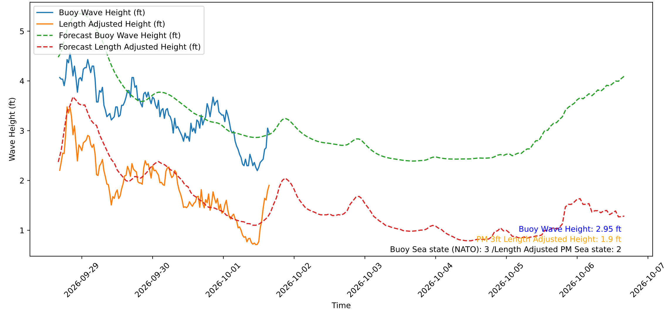
Wave Heights over Time for Green Beach at 2026-10-01 16:21:14
