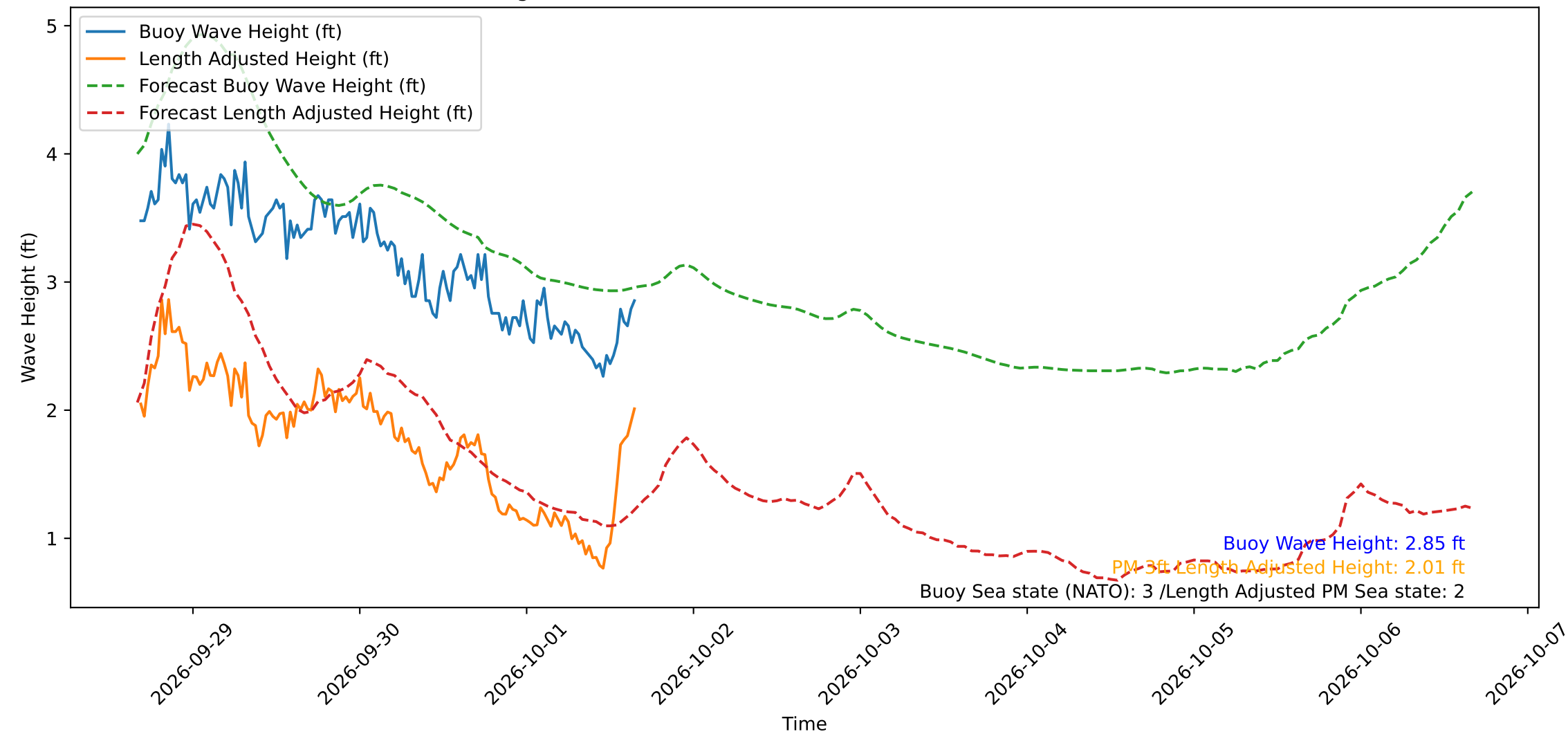
Wave Heights over Time for Oceanside Harbor at 2026-10-01 16:20:29
