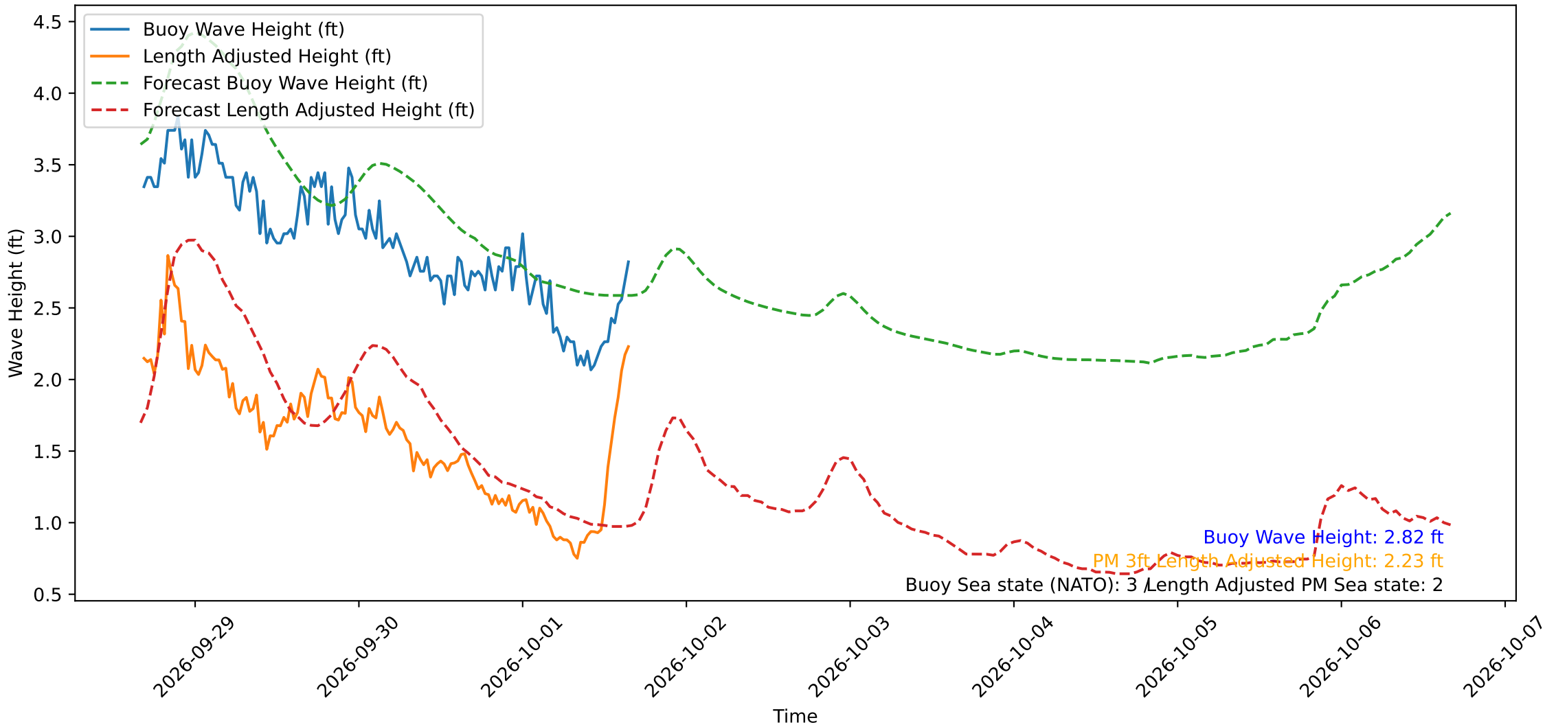
Wave Heights over Time for Red Beach at 2026-10-01 16:20:50
