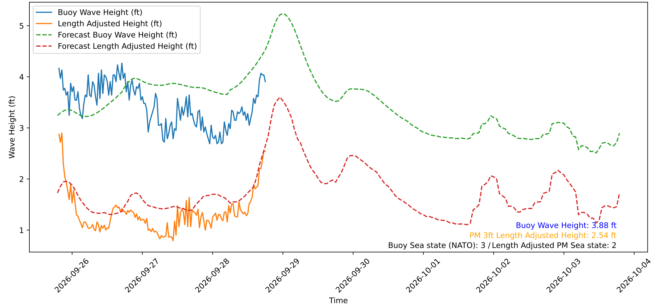
Wave Heights over Time for Green Beach at 2026-09-28 19:21:15
