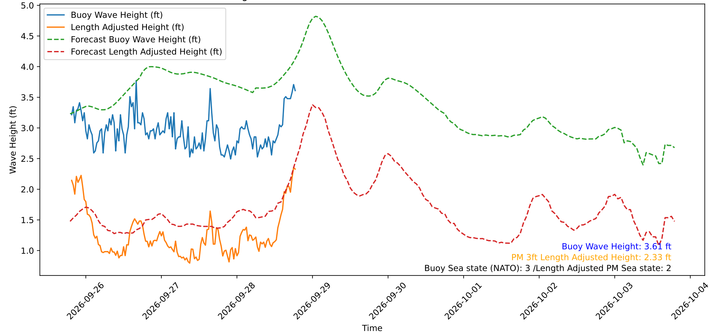
Wave Heights over Time for Oceanside Harbor at 2026-09-28 19:20:29
