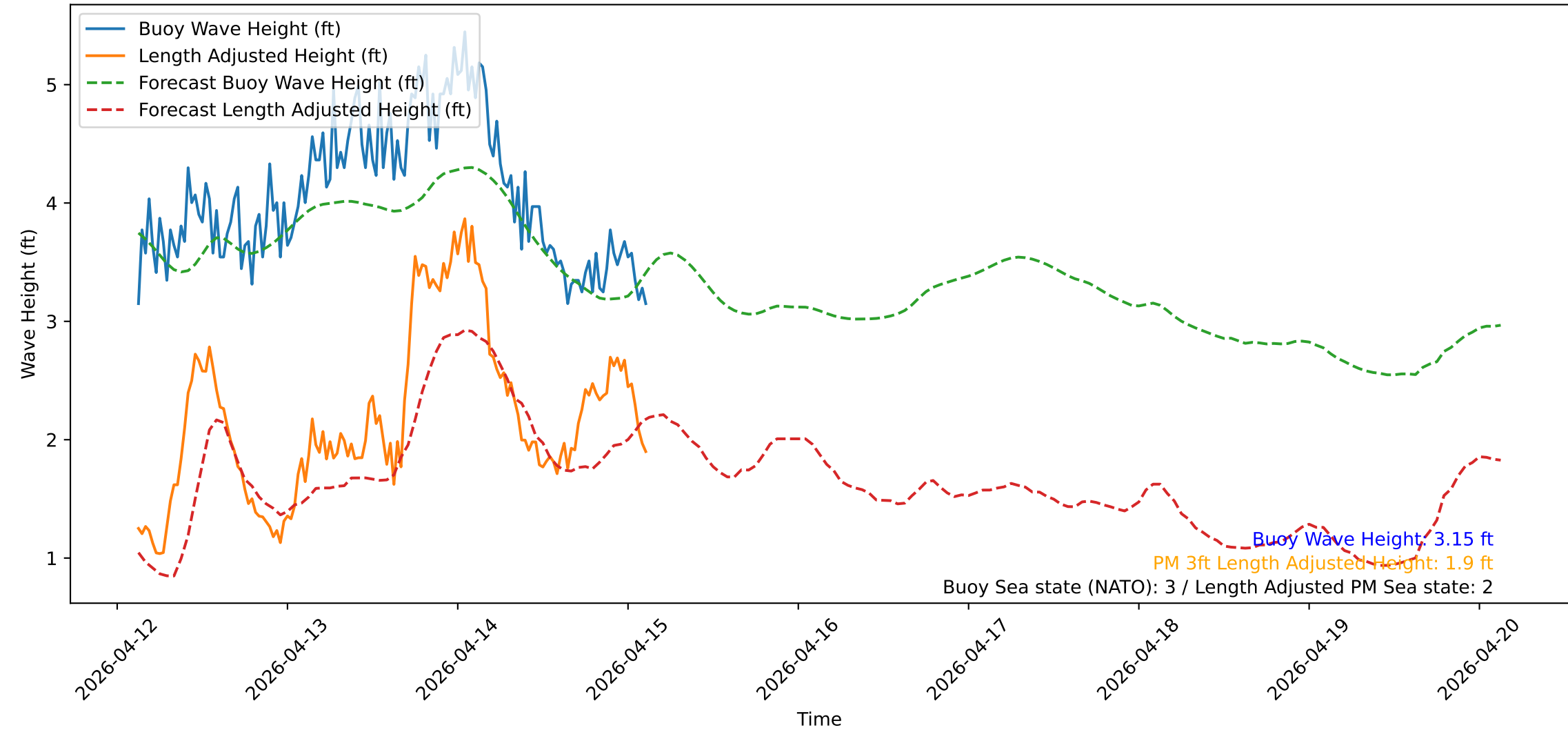
Wave Heights over Time for Oceanside Harbor at 2026-04-15 03:00:31
